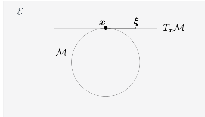
Figure 2.1: Illustration of a smooth embedded submanifold with the circle \mathcal{M} = S^1 \subset \mathcal{E} = \mathbb{R}^2 , its tangent space T_x\mathcal{M} = \{\xi \in \mathbb{R}^2 : x^T \xi = 0\} at a given x \in \mathcal{M} and a tangent vector \xi \in T_x\mathcal{M} .
