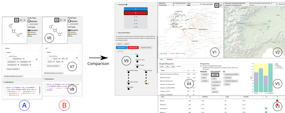
Figure 4.1 – The ComBiNet system was used to compare two subgroups of a social network of contracts from [55], extracted with dynamic visual queries. (A) and (B) show the two visual queries created by the user in the query panel using an interactive node-link diagram editor (V6), dynamic query widgets (V7), and the equivalent Cypher script (V8). The right part shows ComBiNet’s global interface in comparison mode: (V1) Network visualization panel, (V2) Map of the geolocalized nodes, (V3) Table of persons, (V4) Graph measures comparison, (V5) Attribute distribution plots, and (V9) Provenance tree. The two visual queries on the left, select the “Menafoglio” family on the left, and the “Zo” family on the right, along with their construction contracts and close collaborators.
