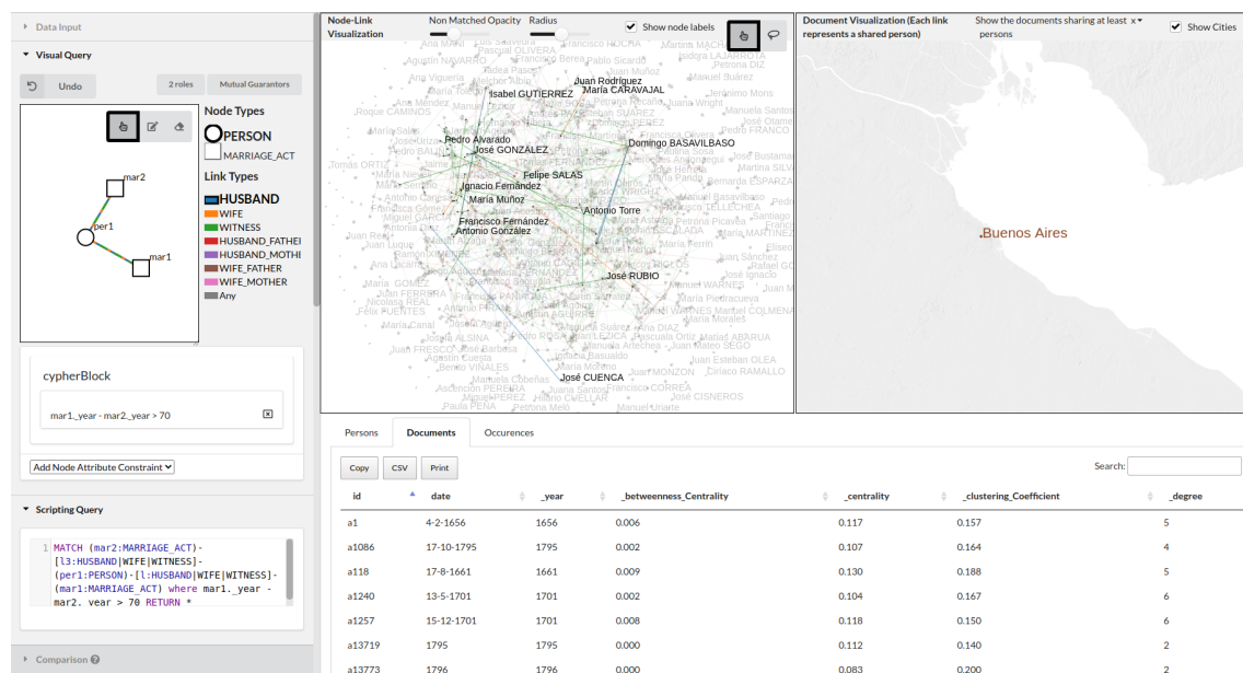
Figure 4.16 – ComBiNet used to request persons appearing as husband, wife, or witness in two marriages that occurred 70 years apart or more.
