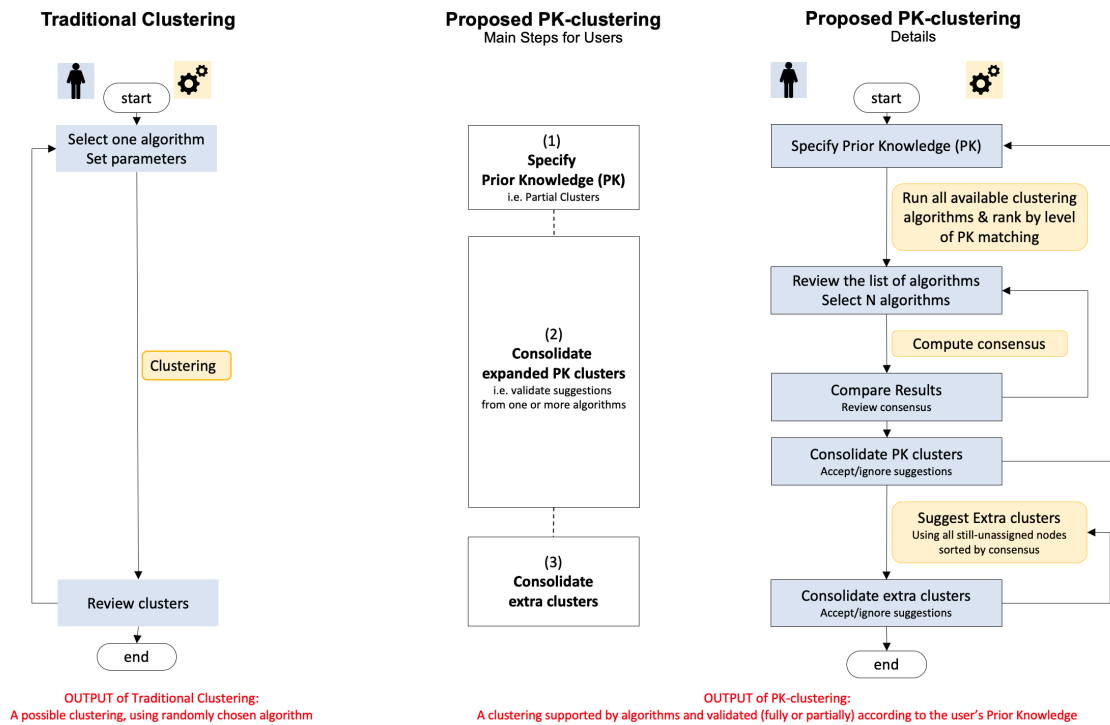
Figure 5.1 – Process of traditional clustering (left) and our PK-Clustering approach (middle and right). The output of traditional clustering is a possible clustering, using an algorithm among many choices. The output of PK-Clustering is a clustering supported by algorithms' consensus and validated (fully or partially) according to the user's PK.
