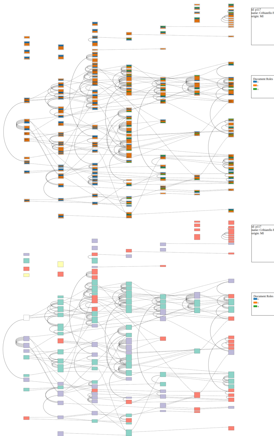
Figure 6.2 – Prototype of a document-centered dynamic layout for bipartite multivariate dynamic networks, showcased with construction contracts in Piedmont (see collaboration #1 in chapter 3). The layout can show the mentions of persons encoded with their roles as color (top) or a focus on the documents if a property is selected (bottom). Here, the region attribute is selected, hence coloring construction contracts depending on their locations.
