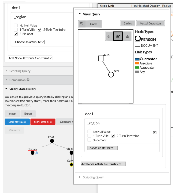
Figure 4.8 – Provenance tree to answer question 2 of collaboration #1: left branch leads to Torino documents (the node is labeled as A) while right branch leads to surrounding documents (the node is labeled as B). The user hovers over one node, revealing a tooltip that shows the visualization of the node’s query.
