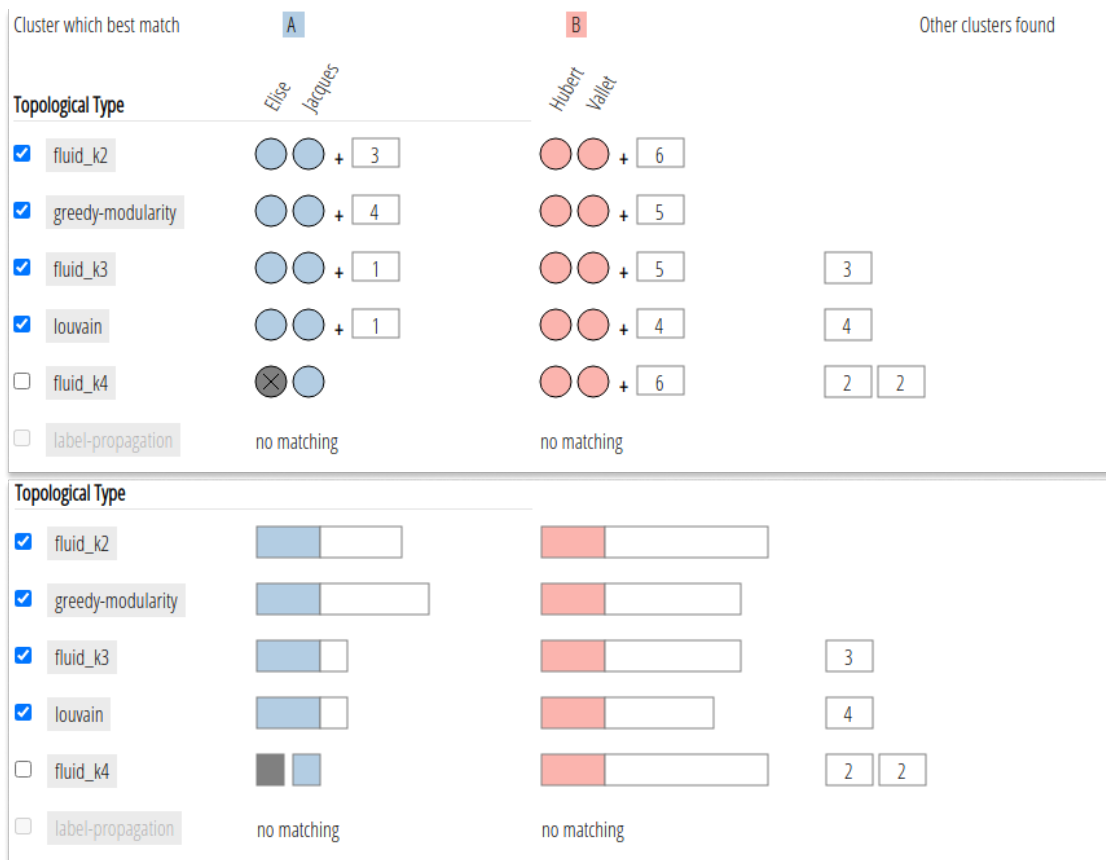
Figure 5.4 – Two different modalities for the ranked list of algorithms. Top: persons are shown as circles. Bottom: aggregated view. Colors indicate the matching group. Gray indicates no match. White indicates extra nodes or clusters.
