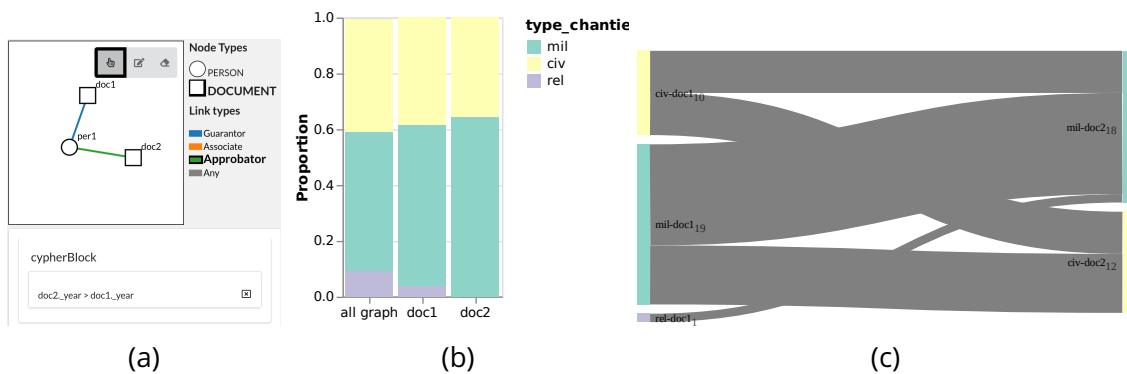
Figure 4.7 – Two ways of showing the distribution of “type chantier” (type of works), a categorical attribute with three possible values “religious”, “military”, and “civilian”. (a) A query matching the contracts made by the same person ( per1 ) as an “approbator” (green link to doc2 ) after being a “guarantor” (blue link to doc1 ) using the constraint ( doc2._year > doc1._year ). (b) Stacked bar chart for the matches, the earlier contract ( doc1 ), the older contract ( doc2 ), and (c) Sankey diagram with the early values on the left and the last on the right. The Sankey diagram reveals the value changes between the two documents: the guarantor who worked initially on religious work switched to military work.
