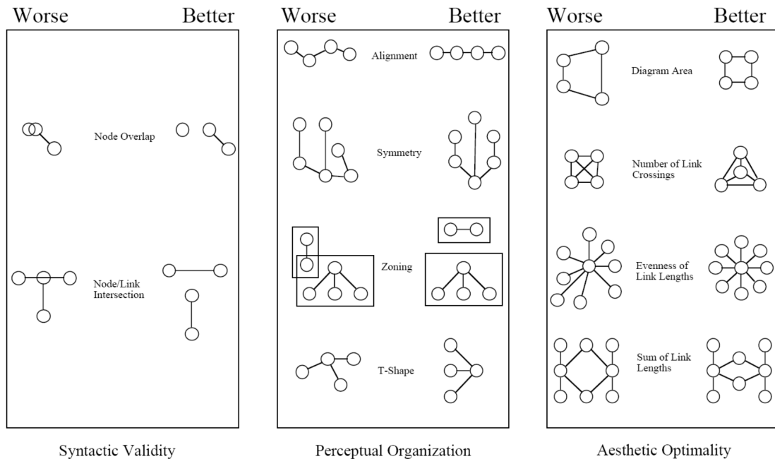
Figure 2.8 – Different criteria are proposed to enhance node-link diagram readability, such as the level of node overlap, the alignment of nodes, or the number of edge crossings. Image from [143].
