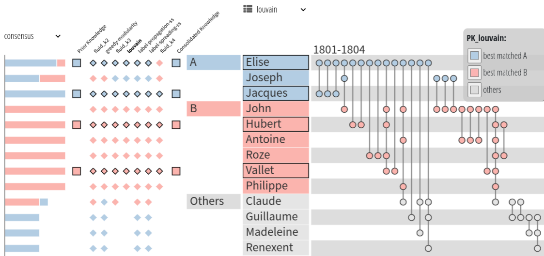
Figure 5.5 – Reviewing and comparing results of multiple algorithms. One algorithm is selected to order the names and group them, but icons show how other algorithms cluster the nodes differently, summarized in the consensus bar on the left.
