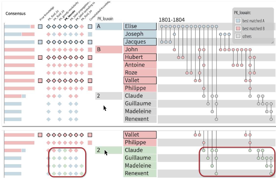
Figure 5.7 – The suggestion of extra clusters. The two PK-groups (red and blue) are validated (nodes in the consensus column are all squared). One extra cluster is proposed by the Louvain algorithm, labeled as 2. Hovering over cluster 2, the consensus is displayed by the green diamonds. This feedback is also visible in the graph.
