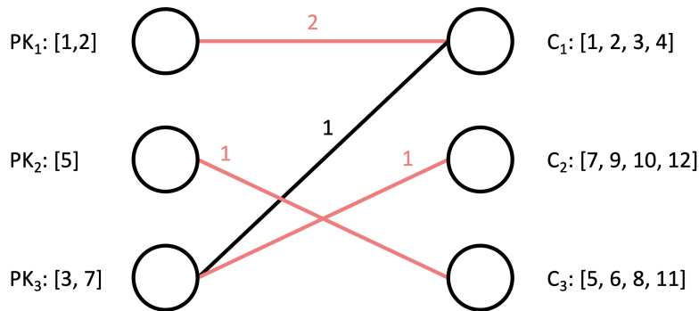
Figure 5.3 – Red edges represent the prior knowledge matching.
