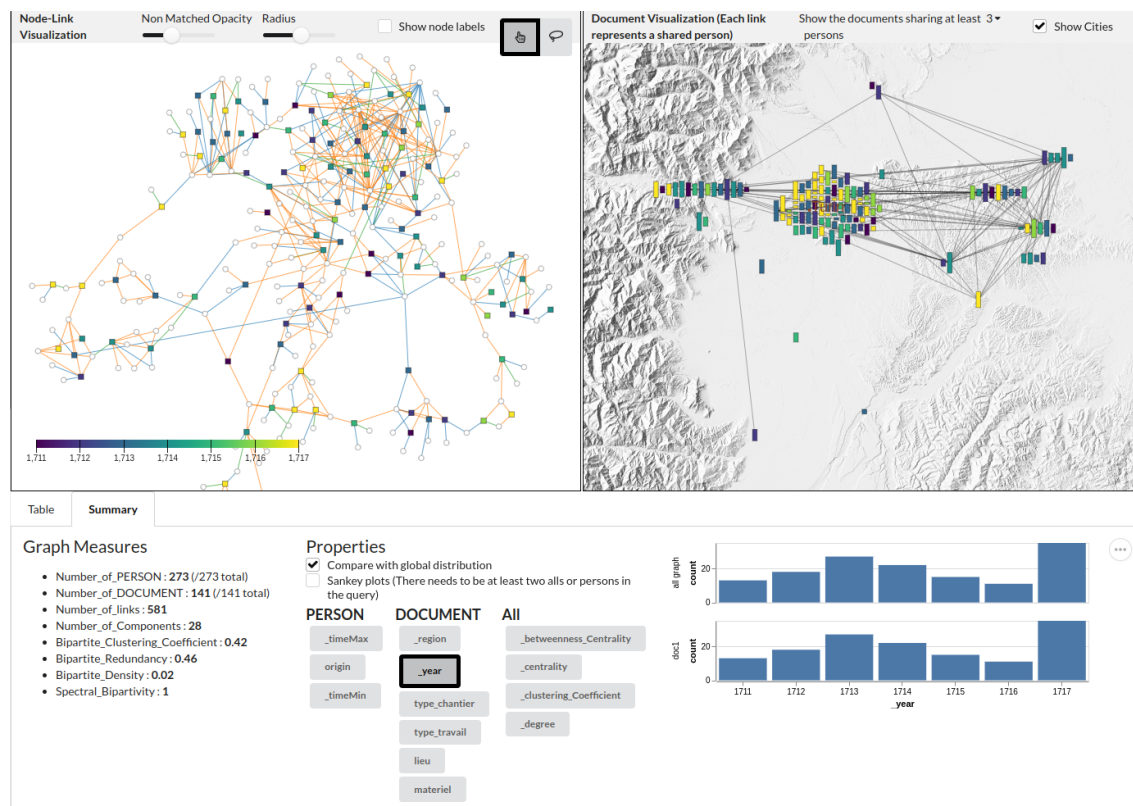
Figure 4.2 – ComBiNet interface with the dataset of collaboration #1. The user selected the _year attribute, showing the distribution of document years with a histogram (bottom right), and coloring the documents node on the bipartite view (left) and map view simultaneously (right).
