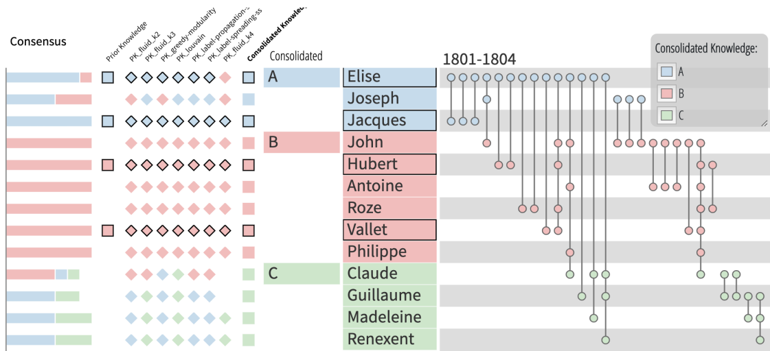
Figure 5.8 – The dataset has been fully consolidated. The persons are grouped and colored by the consolidated knowledge. The user decided to assign Claude, Guillaume, Madeleine, and Renexent to cluster C , by taking into account the graph and the consensus of the algorithms.
