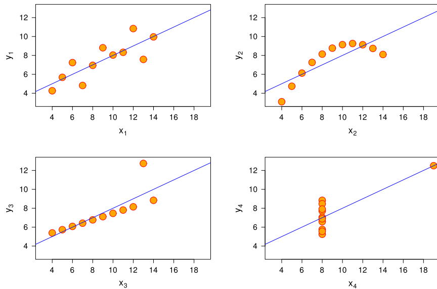
Figure 2.2 – Anscombe quartet. The four datasets have the same descriptive statistics (mean, variance, correlation coefficient, linear regression line) but very different structures. Image from [8].
