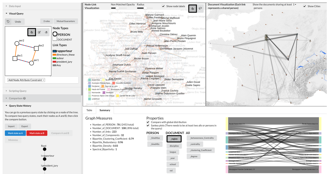
Figure 4.18 – Sociology thesis dataset explored with ComBiNet. The user constructed a visual query to see if there are symmetrical relationships between the thesis directors and reviewers (or jury directors). The region attribute is selected with the Sankey option, letting the user see if there are correlations between the regions of the thesis found in this pattern.
