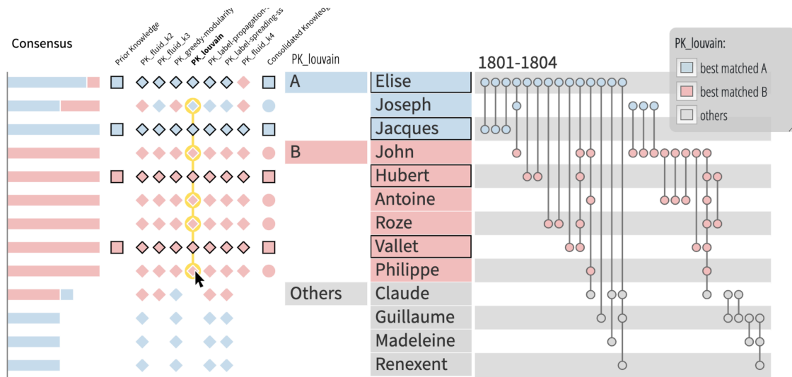
Figure 5.6 – The user quickly drags on consecutive icons (in yellow) representing the suggestions made by one algorithm to validate node clustering. Once the cursor is released the validated nodes appear as squares icons in the Consolidated Knowledge column.
