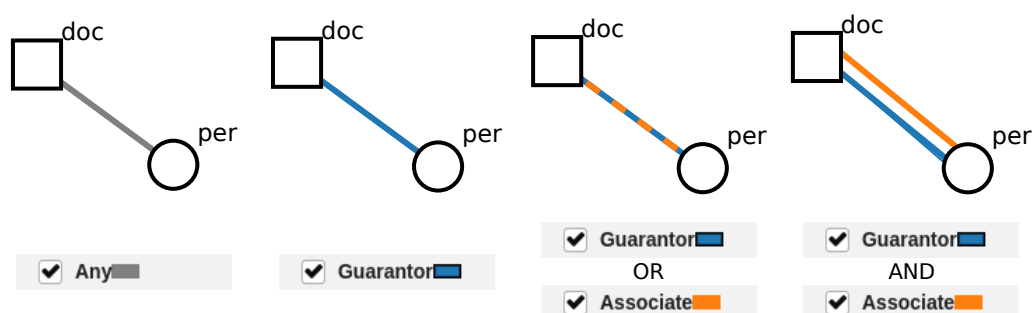
Figure 4.3 – All link creation possibilities: Any link type (left), one selected link type, here guarantor (middle left), the union of several link types (middle right), several links with different types (right).
