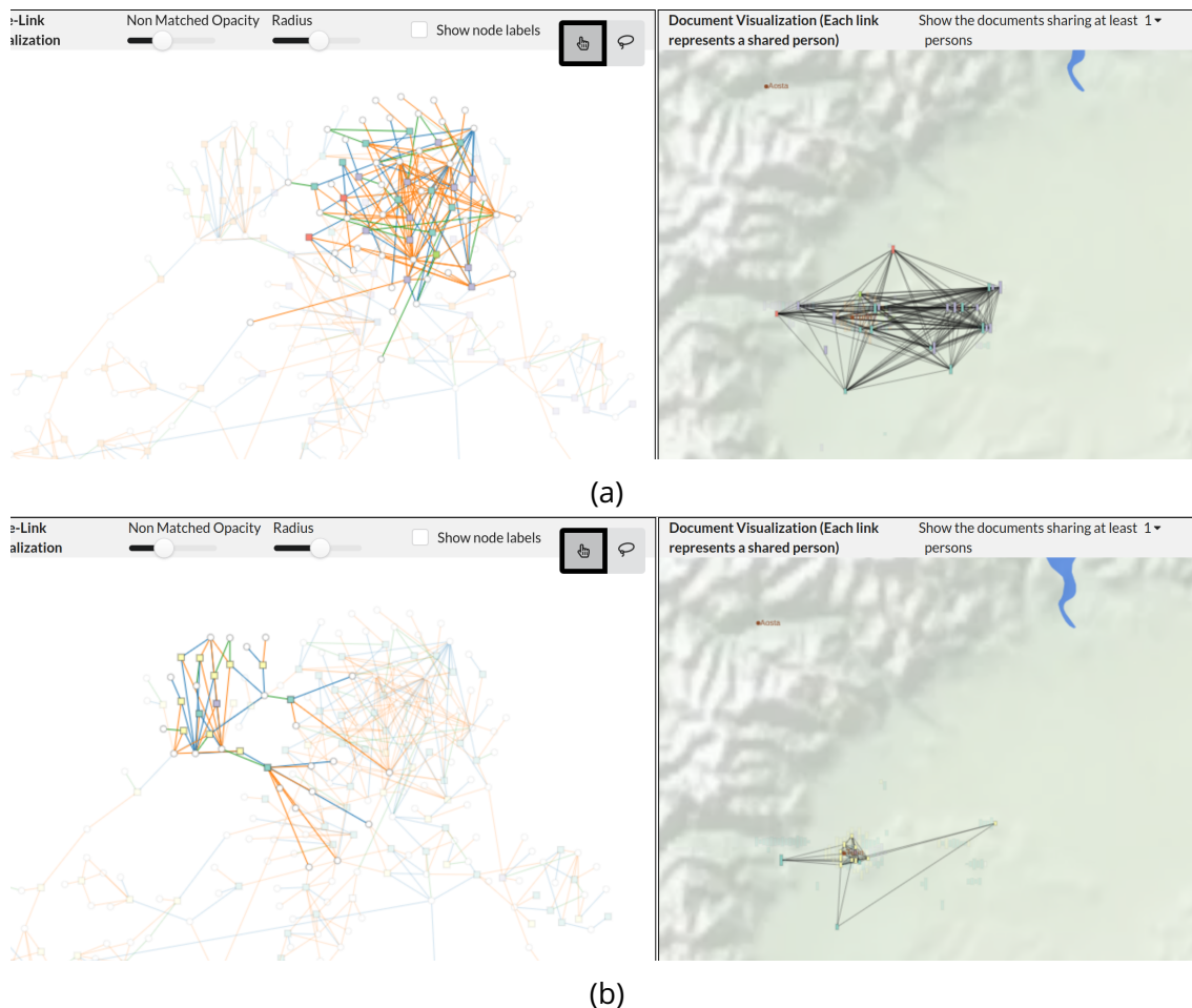
Figure 4.11 – Menafoglio (a) and Zo (b) families were retrieved with queries and highlighted in the bipartite node-link and map views.
