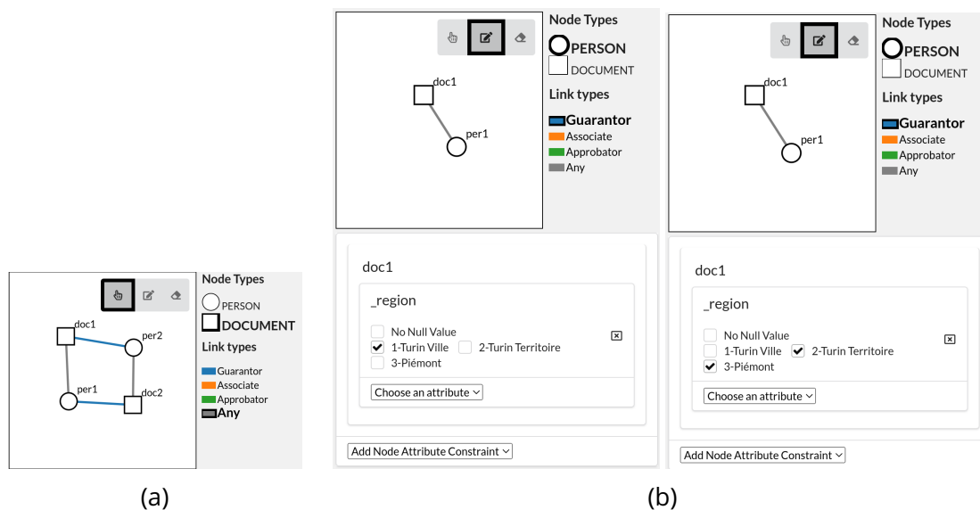
Figure 4.4 – Visual queries created to answer questions 2 and 6 of our collaboration #1. (a) The visual query retrieves individuals who are mutually guarantors to each other in separate construction contracts. (b) The two visual queries retrieve the documents—along with the signatories—of Torino ( Turin in french) (left) and of Torino’s surroundings ( Turin Territoire and Piémont ) (right).
