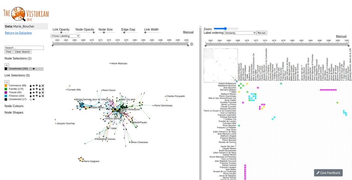
Figure 2.10 – The Vistorian interface [221] used to explore a historical social network of business trades in the 17th century, with a coordinated node-link diagram and a matrix visualization.
