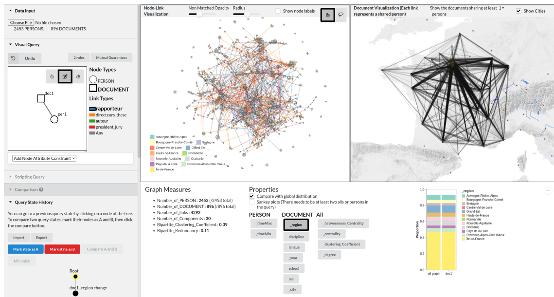
Figure 4.17 – ComBiNet used for exploring theses of sociology defended in France between 2016 and 2021. The bipartite and map views show an overview of two visions of the network. The user selects the region attribute, showing the geographical distribution of the defended thesis.
