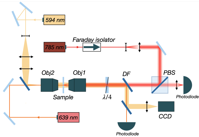
Figure 2.1: Simplified optical setup: the 785 nm trapping laser beam, drawn in red, is optically isolated with a Faraday isolator, expanded with a telescope to overfill the input lens of the microscope objective Obj.1 (Nikon Plan-Apo VC, 60 \times 1.20 Water Immersion) thus focused on the sample. A second low-power 639 nm laser beam is used as a passive probe to measure the position of the bead. The beam is sent to the sample via a low-NA objective Obj.2 (Nikon Plan-fluo ELWD 6 \times 0.70 ) and the light scattered by the sphere is collected by Obj.1 and sent to a photodiode (Thorlabs Det10a). A third low-power 594 nm laser beam is used to image the sphere, focused at the back focal plane of Obj. 2 to go through the sample as a plane wave. The light is collected by Obj. 1 and sent to a CCD camera using a dichroic filter (DF).
