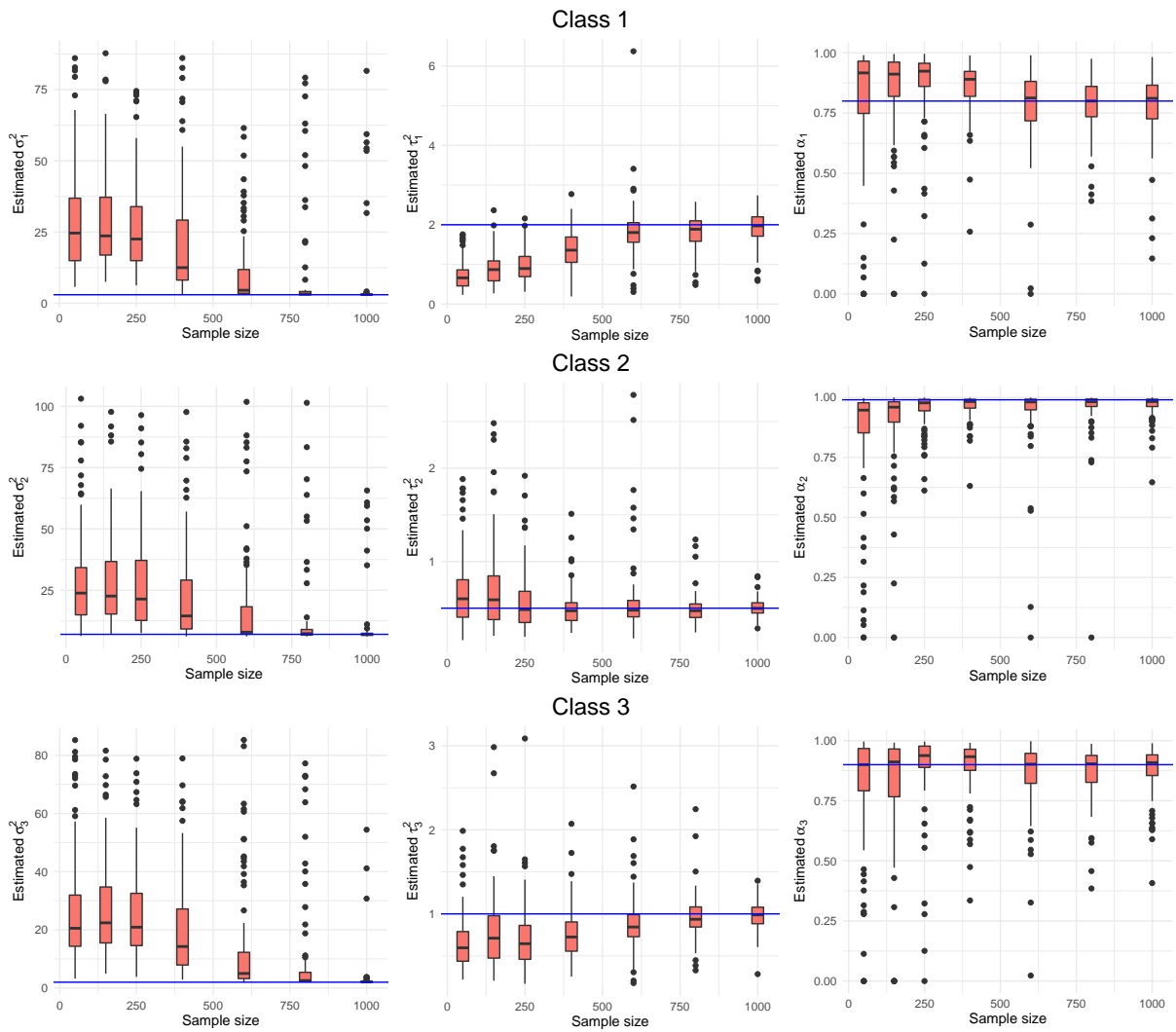
Figure 5.8 – Estimated parameters \sigma_k^2 , \tau_k^2 , and \alpha_k^2 for each class k=1,2,3 as a function of the sample size varying from 50 to 1000. The blue line corresponds to the true value of the parameter.
