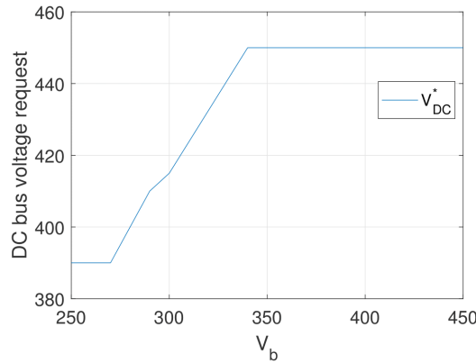
Figure 4.8 – DC bus voltage request in function of the battery voltage
