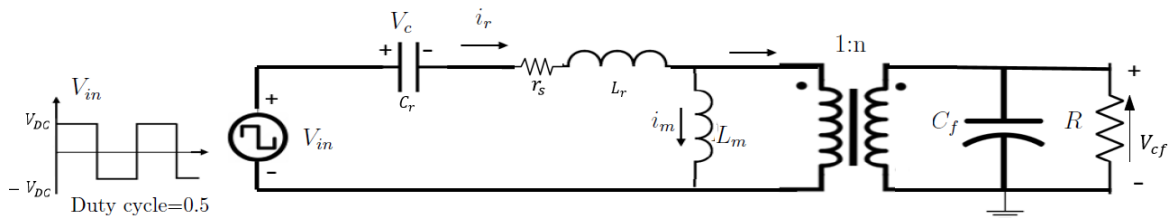
Figure 1.13 – Equivalent circuit of the LLC resonant converter in the forward mode
