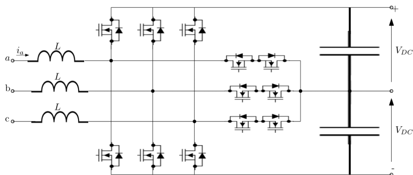
Figure 4.3 – Bidirectional Vienna AC-DC topology
