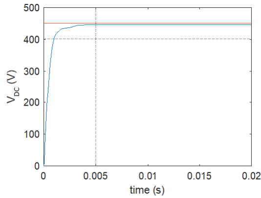
Figure 2.9 – DC bus voltage with PFM for V_{bat}= 350 V and P= 9000 W
