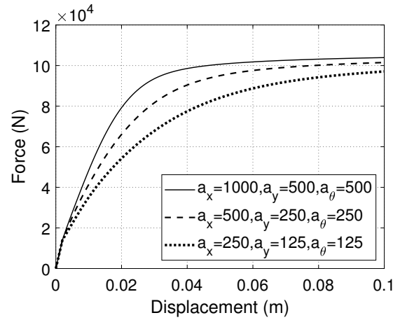
(b) Influence of the parameters a_x , a_y , a_\theta on the global response of a beam.
