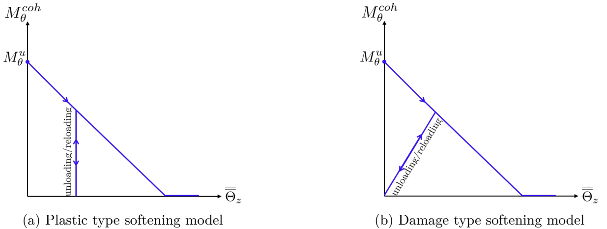
Figure 4.3: Cyclic loading of constant sign: plastic hinge moment – rotational jump relations.
