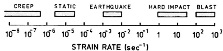
Figure 1.14: Typical strain rates for various types of loading (Bischoff and Perry 1991).
