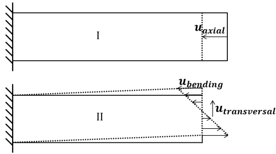
Figure 2.24: 3D loading: I: axial loading, II: radial bending and shear loading by keeping constant the ratio u_{bending}/u_{transversal} .
