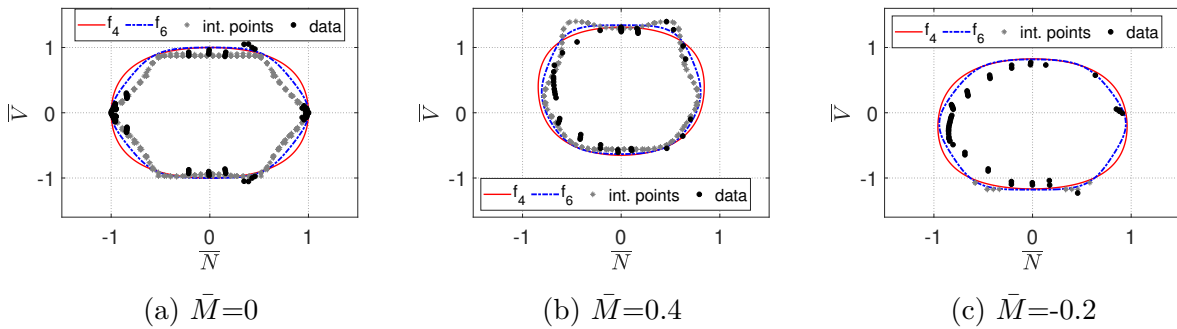
Figure 2.32: M3 section: Axial force - shear force interaction diagrams obtained by polynomials f_4 , f_6 compared to data by numerical simulations and interpolated points.
