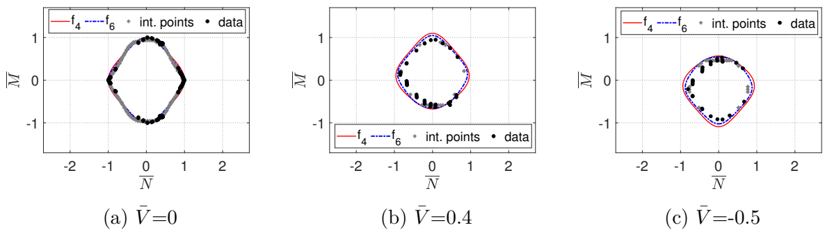
Figure 2.30: M3 section: Moment - axial force interaction diagrams obtained by polynomials f_4 , f_6 compared to data by numerical simulations and interpolated points.
