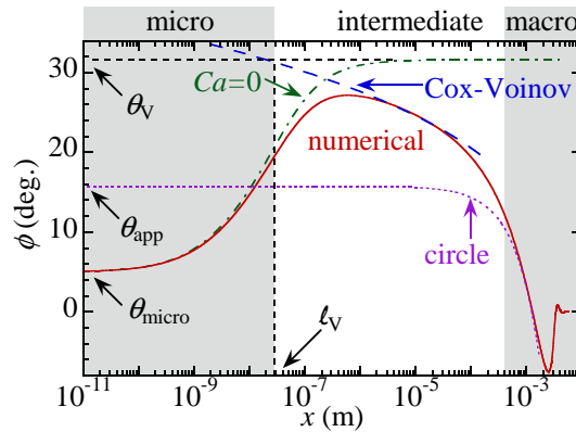
(c) Interface slope variation for Ca = 1.614 \times 10^{-3} .
