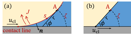
Figure 23: Sketch of (a) a curved interface and (b) the straight liquid wedge, corresponding to the point A.
