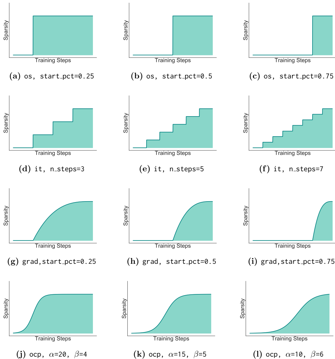
Figure 4.2. Evolution of sparsity along training for the available pruning schedules. While the sched_func parameters defines the general evolution, the schedule can further be customized by modifying the start_pct and end_pct values.
