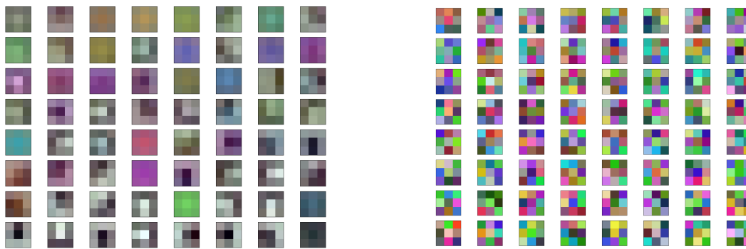
(a) Filters ranked by ascending l_1 -norm for FT-Network. (b) Filters ranked by ascending l_1 -norm for FS-Network.
