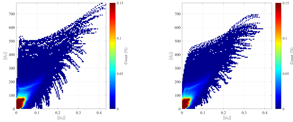
(a) Plastic strain vs plastic strain-rates distribution using FE simulations,
