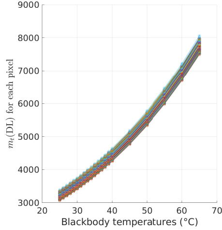
Figure 4.3: \overline{\text{DL}}_t for each pixel versus the BB's temperature, IT = 20 \mu s.
