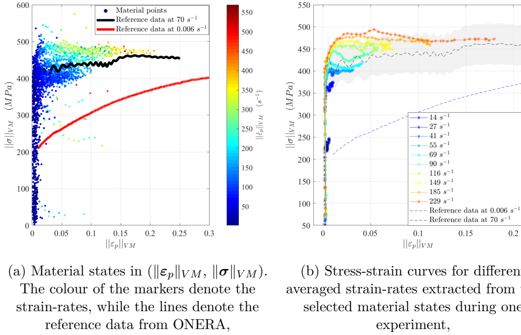
Figure 9.5: Material states in the space (\|\epsilon_p\|_{VM}, \|\sigma\|_{VM}) as well as stress-strain curves for different averaged strain-rates obtained during one experiment.
