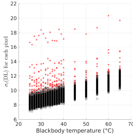
Figure 4.4: \sigma_t[\text{DL}] as a function of T_{\text{BB}} for all the pixels, \text{IT} = 20 \mu\text{s} .
