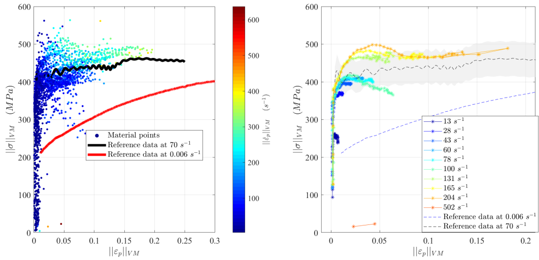
(a) Material states in (\|\epsilon_p\|_{VM}, \|\sigma\|_{VM}) . The colour of the markers denote the strain-rates, while the lines denote the reference data from ONERA,
