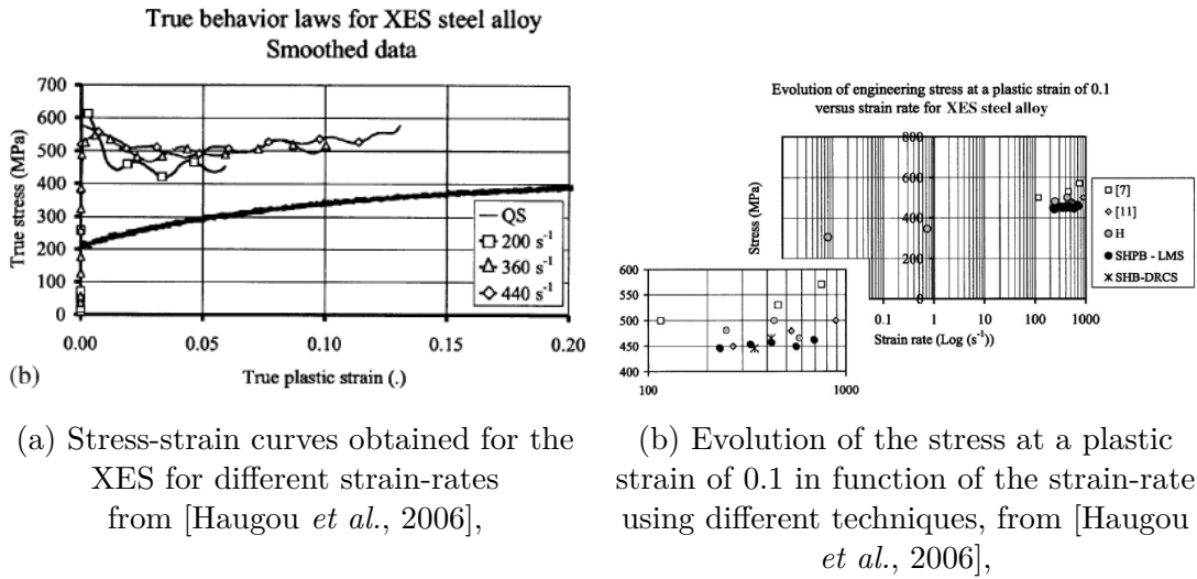
Figure 9.6: XES characterization data from [Haugou et al. , 2006] and comparison of the results obtained using different experimental techniques.
