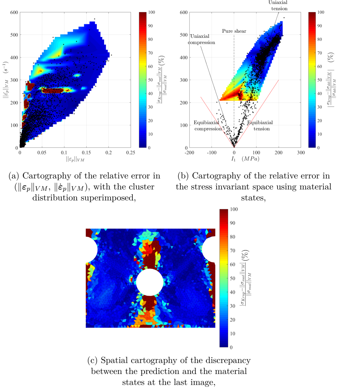
Figure 9.7: Comparison between the stress predictions using the modified Krupkowsky model and the material states from the DDI.
