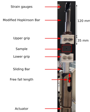
Figure 7.3: Photo of the dynamic tensile machine setup, with a focus on the distances between the strain gage, the grip and the ROI.
