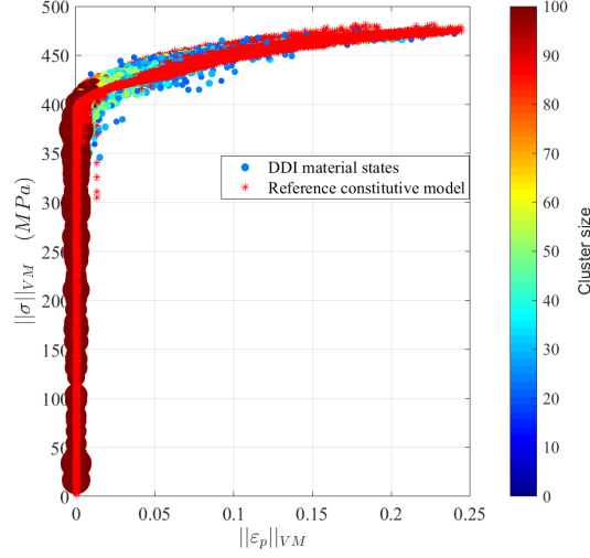
Figure 8.15: Comparison of the DDI material states versus the reference solution (in red) in one projection of the constitutive space ( \|\epsilon_p\|_{VM} , \|\sigma\|_{VM} ). The marker size and colour for the DDI output are related to the size of the cluster. Only the selected clusters are represented.
