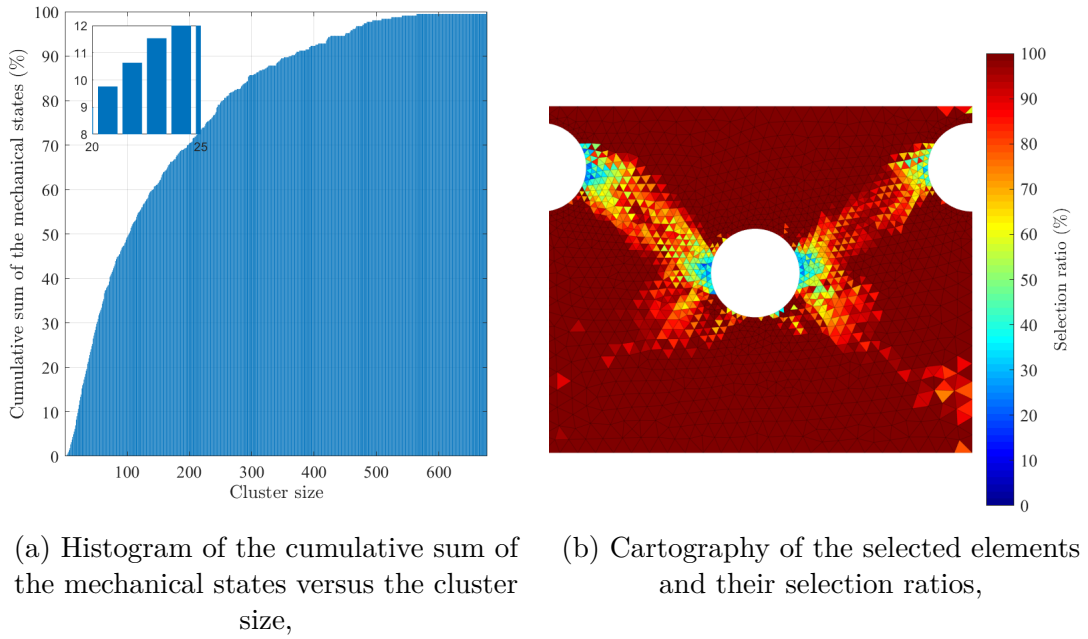
Figure 8.6: Investigation of a selection criterion based on the cluster size.
