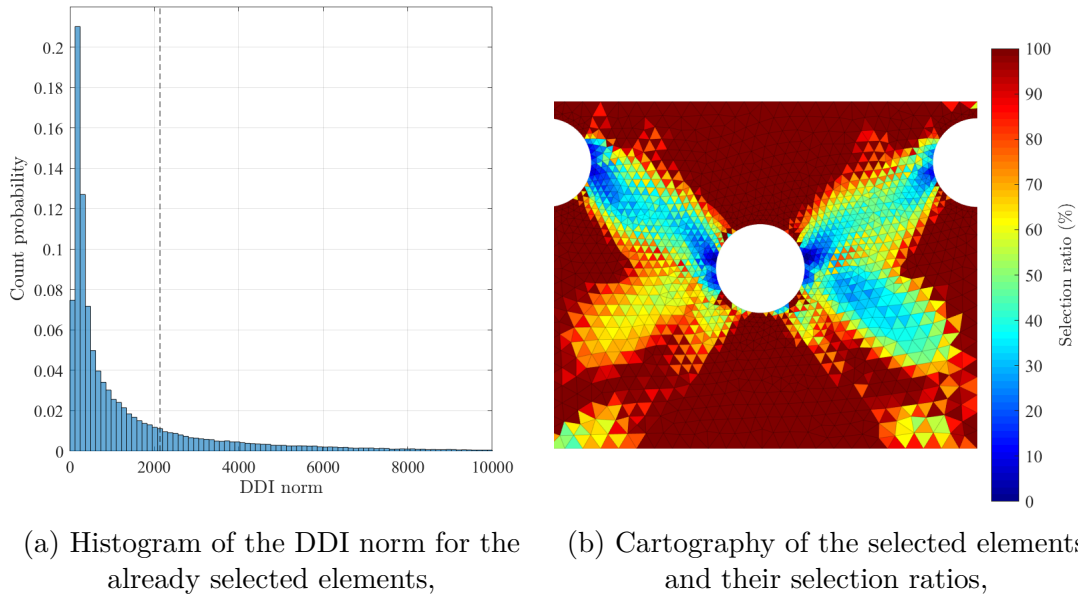
Figure 8.8: Investigation of a selection criterion based on the \|\cdot\|_r norm for the already selected clusters and associated elements.
