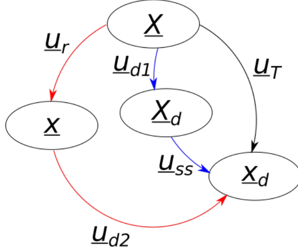
Figure 3.3: Schematic diagram of the transformations for a static sample (in blue) and for a moving sample (in red). This Figure emphasizes the fact that the distortions can differ from one shot to another. \underline{u}_r is the effective displacement, while \underline{u}_{ss} denotes the displacement obtained using a sensor-to-sensor approach.
