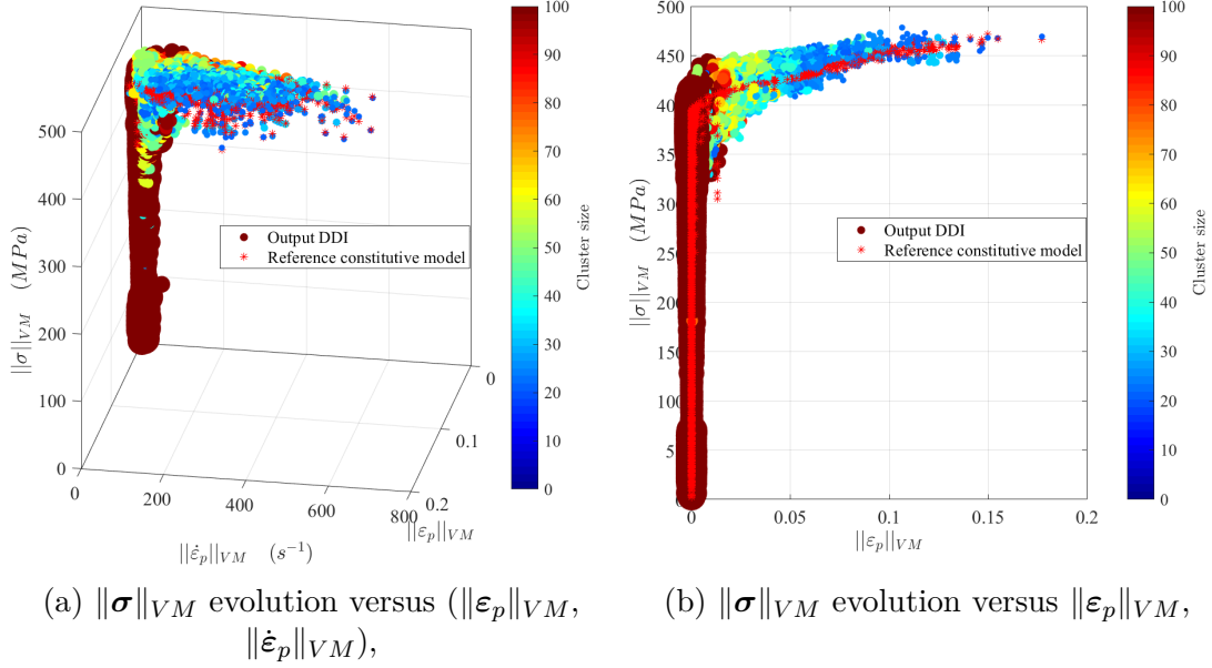
Figure 8.9: Comparison of the DDI output versus the reference solution (in red) in the constitutive space ( \|\epsilon_p\|_{VM} , \|\dot{\epsilon}_p\|_{VM} , \|\sigma\|_{VM} ), and in one projection. The marker size and colour for the DDI output are related to the size of the cluster containing the mechanical state. Only the mechanical states contained in the selected clusters are represented.
