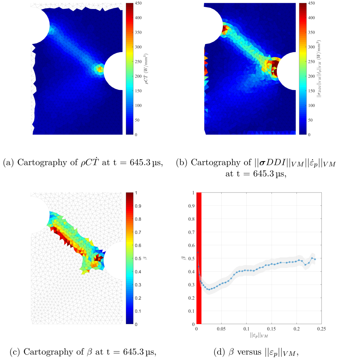
Figure 9.10: Cartography of the Taylor-Quinney coefficient at the last time step from the experiment. The evolution of the average coefficient in a localization band is then plotted versus \|\varepsilon_p\|_{VM} .
