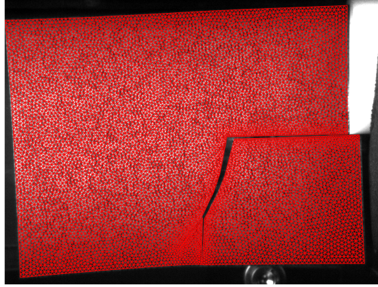
Figure 5.4: Unstructured mesh (in red) with twin nodes along the crack path, deformed and superimposed onto the final frame taken during an impact test.
