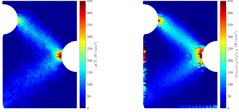
(a) Cartography of \rho C \dot{T} at t = 793 \mu s , (b) Cartography of \|\sigma DDI\|_{VM} \|\dot{\varepsilon}_p\|_{VM} at t = 793 \mu s ,
