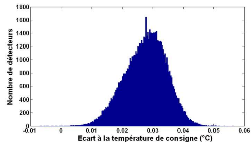
(b) [Bodelot, 2008], IT = 1.100 \mu s , 28^\circ C ,
