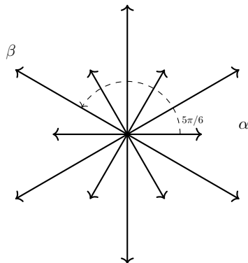
Figure 1: Root system of G_2 .
