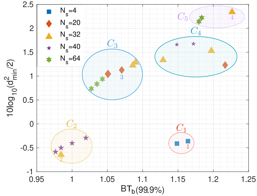
Figure 3.4 – Three Pareto optimum objective functions configurations for LSSB-FSK using B_{99} .
