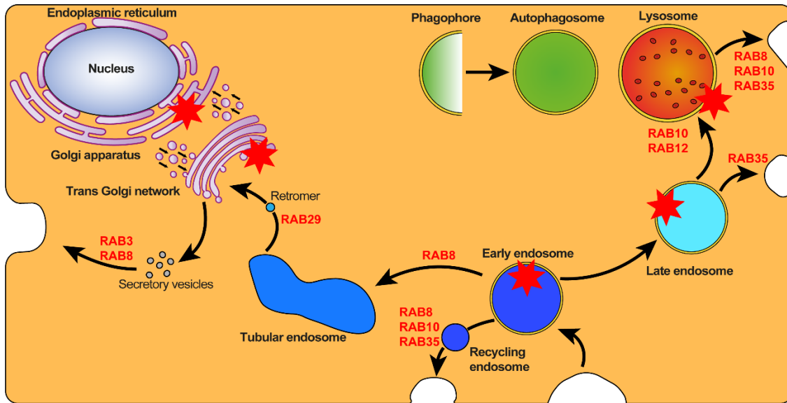
Figure 19: LRRK2 RAB substrates are implicated in the regulation of vesicular trafficking. At the Golgi, RAB1, 29 and 43 regulate the trafficking between the Golgi, TGN and ER. The secretion is regulated by RAB3a, 8, 10 35. The endosomal system transport and maturation is regulated by RAB8a, 10, 12, 35. Adapted From (Bae and Lee, 2020).
