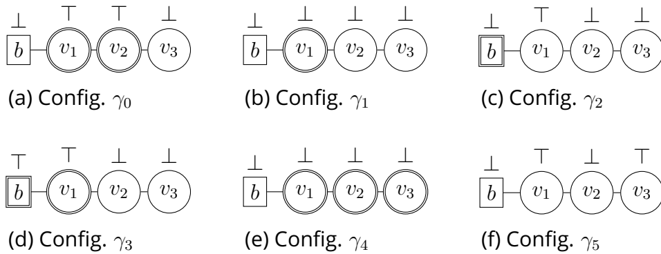
Figure 3.1: An example of execution. The square node is a Byzantine node, the double bordered nodes are those activated in the next transition.
