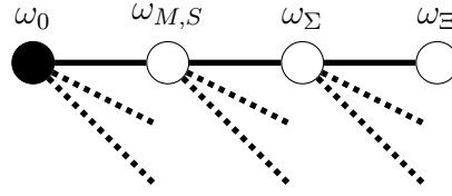
Figure 6.7: The exploration tree after the addition of the third layer of vertices.
