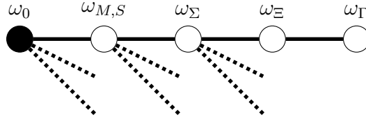
Figure 6.8: The exploration tree after the addition of the fourth layer of vertices.
