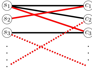
Figure 6.9: A matching in the bipartite graph with parts \Sigma to the left and colors of available partial matching to the right.
