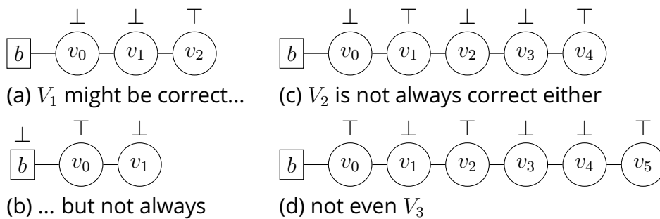
Figure 3.2: What is the good containment radius?
