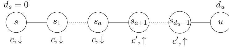
Figure 4.3: Node s propagates its clock value along a shortest path from s to u where c' \in \{c, c - 1\} .
