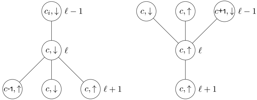
Figure 4.2: Branch coherence condition. The couples (c, \downarrow) or (c, \uparrow) represent the local variables (c_i, b_i) of the nodes. The value on the right of the nodes represents their distance to the leader node ( i.e. their d -value). The central node in both figures is the reference, and the other nodes represent the possible couples for its neighbors with different d -value.
