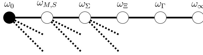
Figure 6.10: The completed exploration tree.
