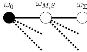
Figure 6.6: The exploration tree after the addition of the second layer of vertices.
