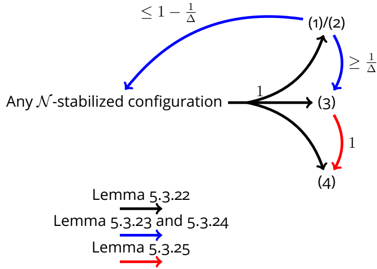
Figure 5.1: (1), (2), (3), and (4) refer to configurations having properties numbered in Lemma 5.3.22. Values on arrows are probabilities given by the lemmas.
