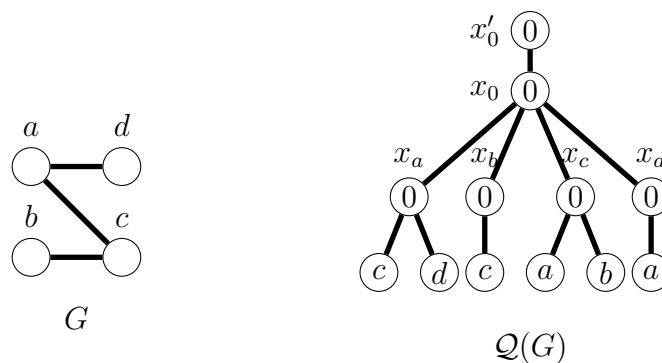
Figure 6.2: A bipartite graph G , and its transformed version Q(G) (colors depicted in the nodes).
