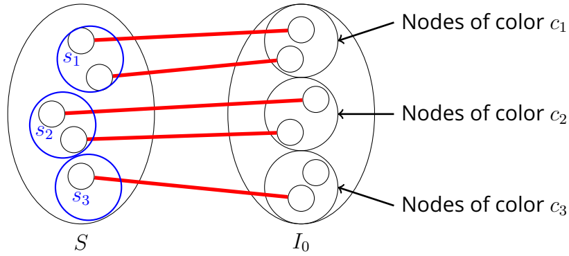
Figure 6.5: The partition \Sigma = \{s_1, s_2, s_3\} of S by matching color on the “exterior side” ( I_0 ). Red edges are the edges of a matching compatible with the partition \Sigma .
