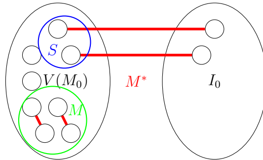
Figure 6.3: Decomposition of a matching M^* according to the structure of M_0 .
