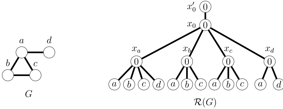
Figure 6.1: A graph G , its transformed version \mathcal{R}(G) (colors depicted in the nodes).
