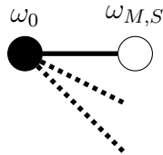
Figure 6.4: The exploration tree after the addition of the first layer of vertices.
