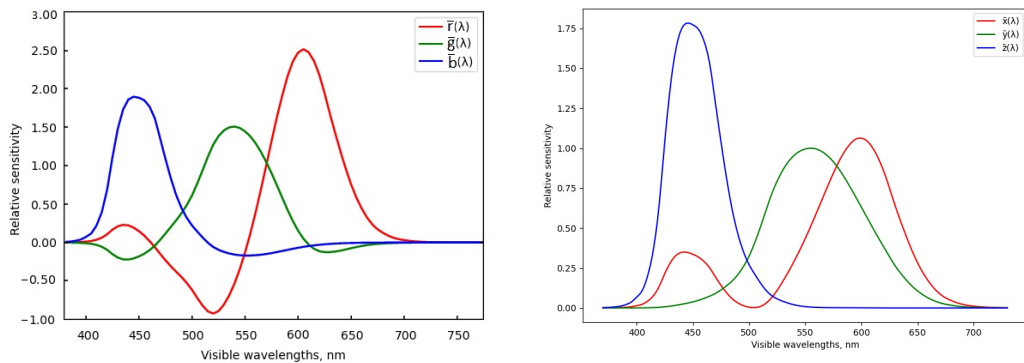
(a) CIE 1931 \bar{r} , \bar{g} , \bar{b} color matching functions. (b) CIE 1931 \bar{x} , \bar{y} , \bar{z} color matching functions.
