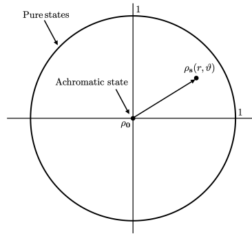
Figure 3.2: Hering's rebit as a quantum-like formalization of Newton's chromatic disk.
