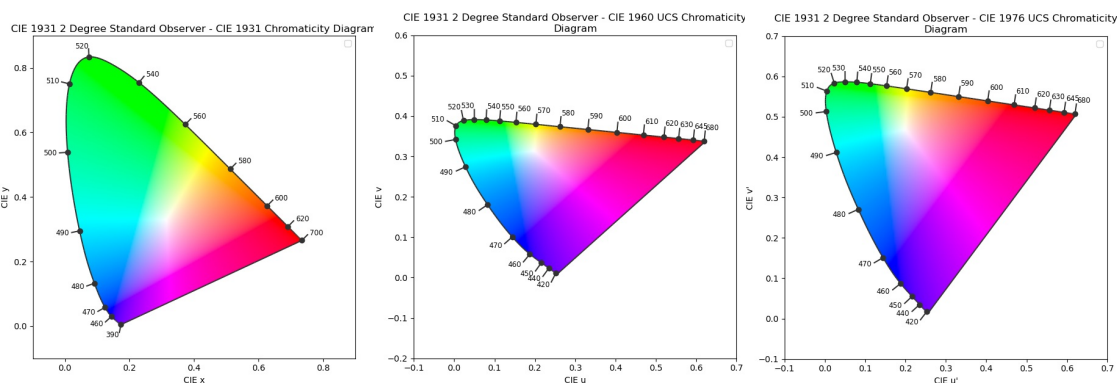
Figure 1.5: Left : CIE 1931 xy chromaticity diagram. Center : CIE 1960 UCS uv chromaticity diagram. Right : CIE 1976 UCS u'v' chromaticity diagram. These figures have been created using the open-source Python package Colour , see https://colour.readthedocs.io/en/develop/ .
