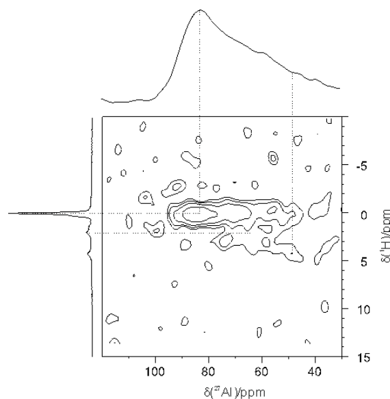
Figure 2.7.14. ^1\text{H} - ^{27}\text{Al} HMQC experiment
