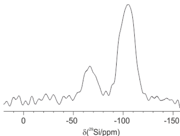
Figure 5.3.9. ^{29}\text{Si} CPMAS NMR spectrum of SiO 2 -1000-Pic (9.4 T, \nu_r = 6 kHz)
