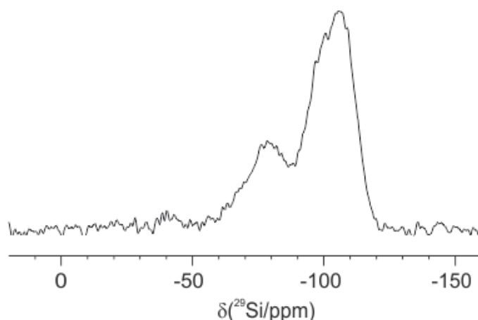
Figure 5.3.13. ^{29}\text{Si} CPMAS NMR spectrum of SiO 2-1000 -DMBA
