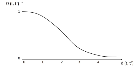
Figure 5.13: Diagram of autocorrelation independence. The omega-covariance function admits independence after 4 weeks.
