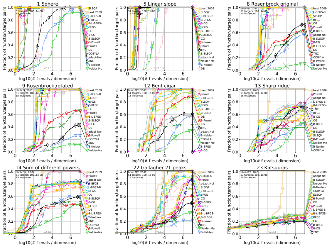
Figure 3.5: Empirical cumulative distribution of simulated (bootstrapped) runtimes, measured in number of function evaluations, divided by dimension (FEvals/DIM) for the 51 targets 10^{-8, \dots, 2} in dimension 20.
