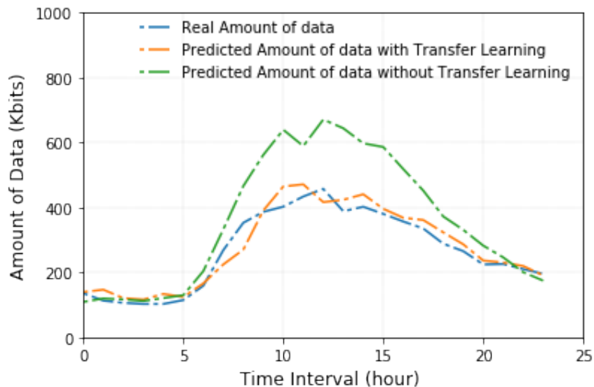
FIGURE 3.3: The pertinence of transfer learning use with One hour granularity prediction
