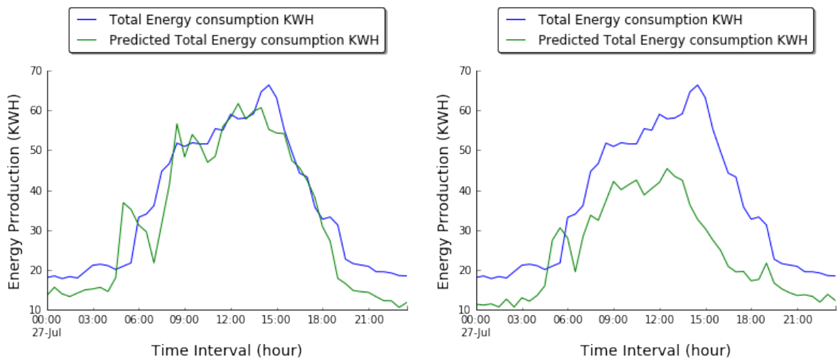
(A) 30 Minutes energy consumption real vs pre-predicted with LSTM (B) 24 Hour energy consumption real vs predicted with LSTM
