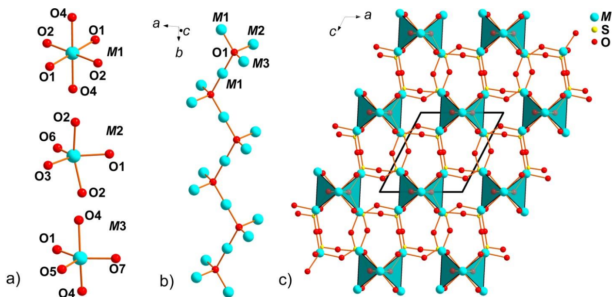
Figure 26. Coordination of M sites in (\text{Zn,Cu})_3\text{O}(\text{SO}_4)_2 (a). [\text{M}_3\text{O}]^{2+} chain elongated along the b axis (b). General projection of the crystal structure of (\text{Zn,Cu})_3\text{O}(\text{SO}_4)_2 (c). [\text{M}_3\text{O}]^{2+} chains are highlighted by blue.
