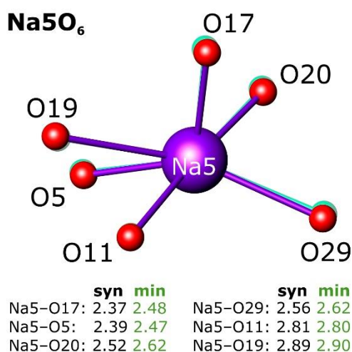
Figure 12. Geometrical environment of the Na5 site in the structure of synthetic Na 2 Cu(SO 4 ) 2 . Projections of the O positions in the structure of saranchinaite are shown by green color for comparison. Distances are given in Å.
