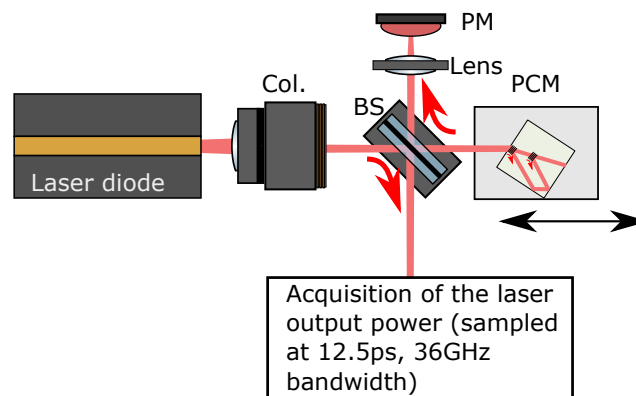
Figure 4.8: The experimental setup used in that section, and its components. The support of the phase-conjugate mirror (PCM), represented in light green, is as close as possible to the mount of the beam splitter (BS). In the illustration, the single-trip distance between the output of the EEL (edge-emitting laser) and the PCM is 14.7 cm.
