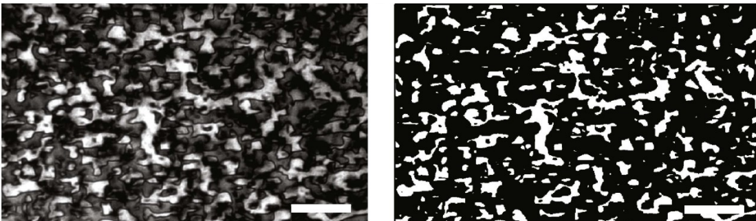
Figure 1.16: (a) The dark field TEM on the g = (002) diffraction peak of a 20 nm thick GaP/Si sample grown by molecular beam epitaxy. (b) Binarized image after applying a threshold mask in (a). The scale bars are 50 nm long. Image: Courtesy of Ref.[34].
