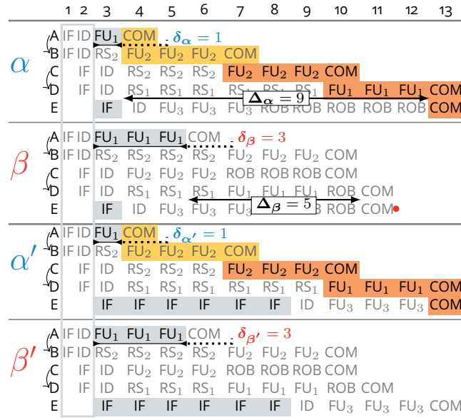
Figure 7.1: Execution of a program with data dependencies ( L ) on our OoO-pipeline model (with superscal = 2 and N_{FU} = 3 , cf. Sec. 2.3). Traces \alpha/\alpha' vs. \beta/\beta' exhibit a local variation wrt. FU_1 for A ( \blacktriangleleft ). \alpha/\beta vs. \alpha'/\beta' exhibit a local variation wrt. IF for E ( \blacksquare ). \beta' is the local-worst-case trace according to the definition by Reineke et al. [22], which indicates the absence of TAs. \alpha/\alpha' vs. \beta/\beta' , however, constitute a well-established example of a TA [21, 22, 23, 24, 34]. Symbols \delta , \Delta , and the colored cells are relevant for our definition (cf. Sec. 7.2).
