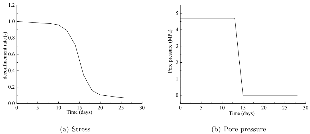
Figure V .9: Deconfinement curve
