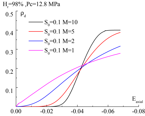
(b) Volume fraction of debonded inclusions \rho_d
