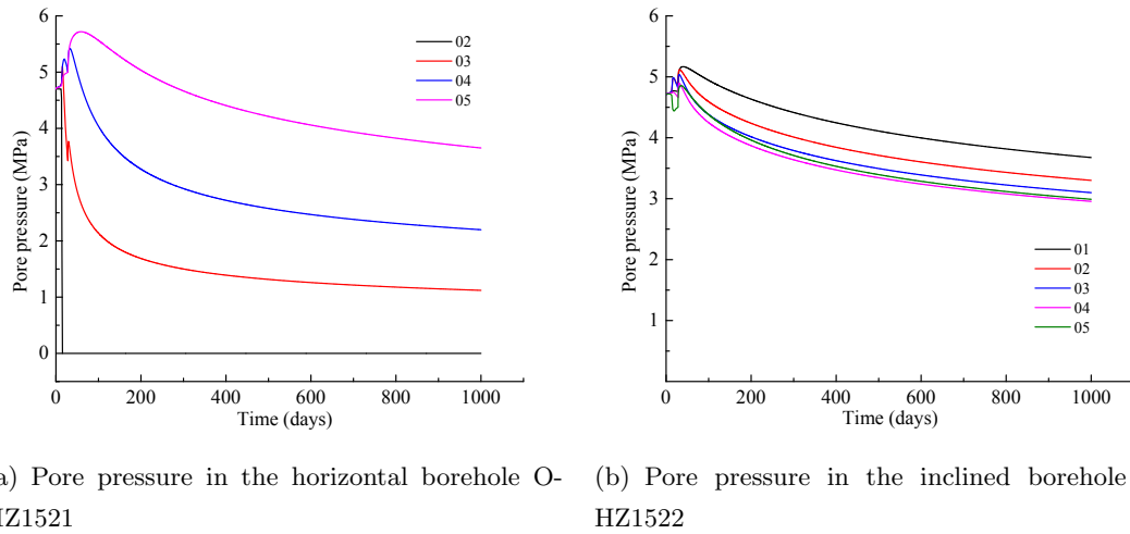
Figure V .22: Variation in pore pressure in horizontal and inclined borehole for GED gallery
