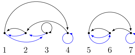
Figure 9.2: Multipermutation of rank 2 and size 7.
