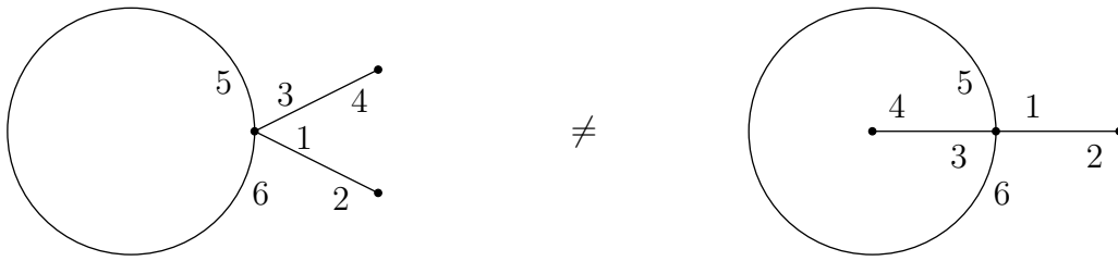
Figure 11.3: Different combinatorial maps with the same underlying graph.
