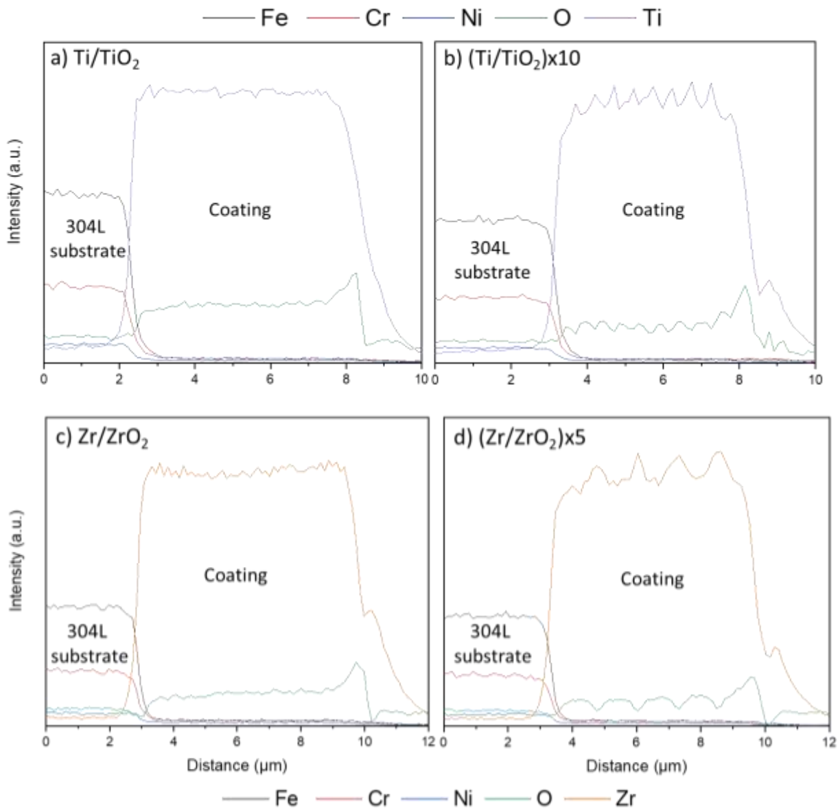
Figure 22: EDX line scans of cross-sections of a) Ti/TiO_2 , b) (Ti/TiO_2) \times 10 , c) Zr/ZrO_2 and d) (Zr/ZrO_2) \times 5 coatings after electrochemical measurements in a 3.56 wt.% NaCl solution at ambient temperature.
