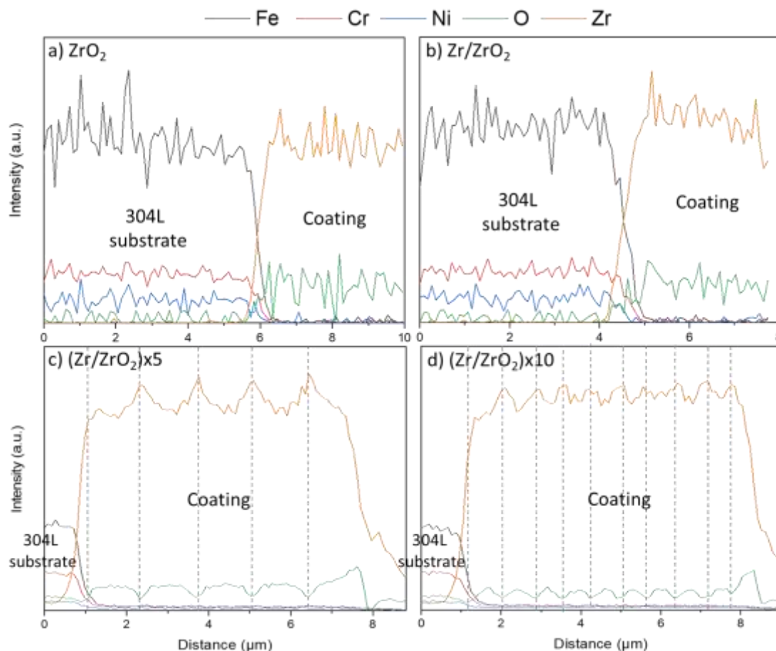
Figure 6: SEM-EDX profiles of cross-sections of a) monolayer ZrO_2 , b) bilayer Zr/ZrO_2 , c) (Zr/ZrO_2) \times 5 and d) (Zr/ZrO_2) \times 10 coatings.
