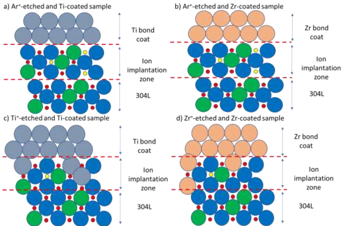
Figure 18: Model of the substrate/bond coat interface obtained for a) \text{Ar}^+ -etched and Ti-coated, b) \text{Ar}^+ -etched and Zr-coated, c) \text{Ti}^+ -etched and Ti-coated and b) \text{Zr}^+ -etched and Zr-coated samples.
