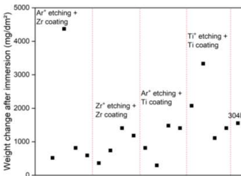
Figure 4: Weight change measurements after 15 days of immersion in natural seawater at Sentosa at ambient temperature (29-30°C)
