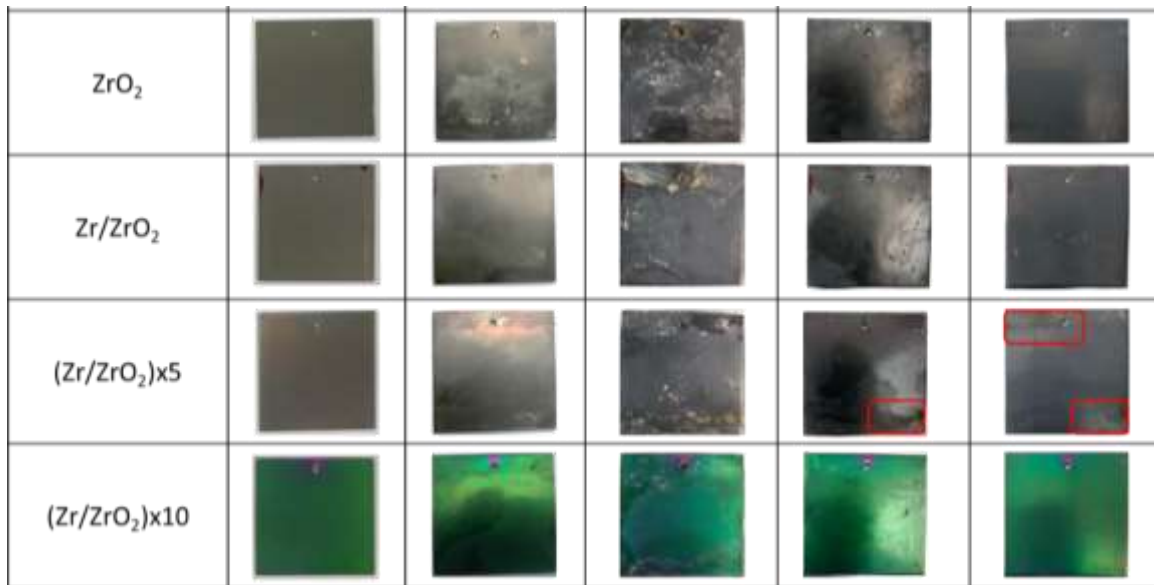
Figure 25: Visual inspection of 304L steel and metal oxide-based coatings each 15 d during the 60 d of immersion in Singapore natural seawater.
