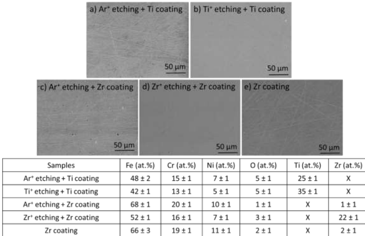
Figure 38: SEM-SE micrographs of a) Ar + -etched and Ti-coated, b) Ti + -etched and Ti-coated, c) Ar + -etched and Zr-coated, d) Zr + -etched and Zr-coated and e) Zr-coated samples and atomic percentages of elements obtained by EDX spectra after electrochemical measurements in a nitric acid (2.5 mol/L HNO 3 , 2.5 mol/L NaNO 3 and 2 g/L Fe(NO 3 ) 3 ) solution at 110°C.
