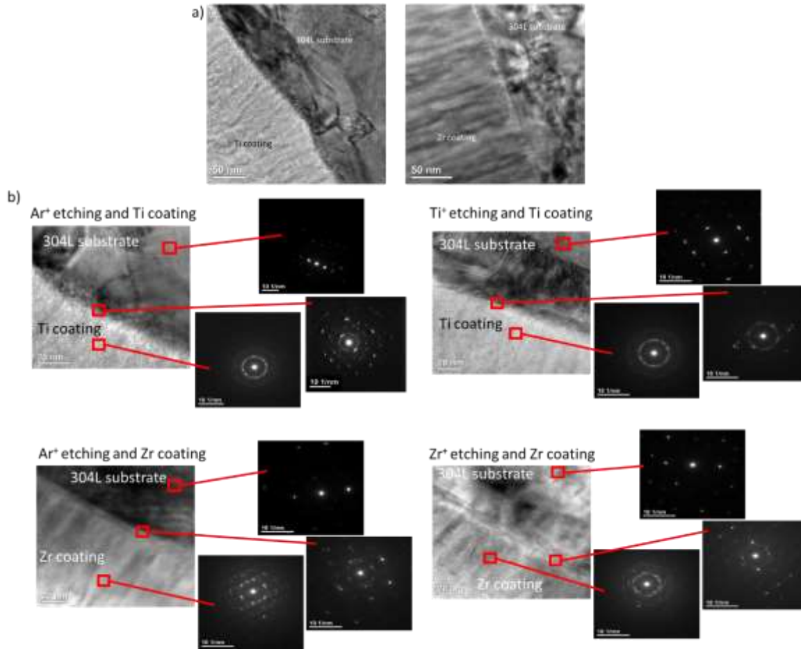
Figure 10: a) TEM images of Ar + -etched and Ti-coated and Ar + -etched and Zr-coated and b) TEM diffraction pattern for different areas of all etched and coated samples.
