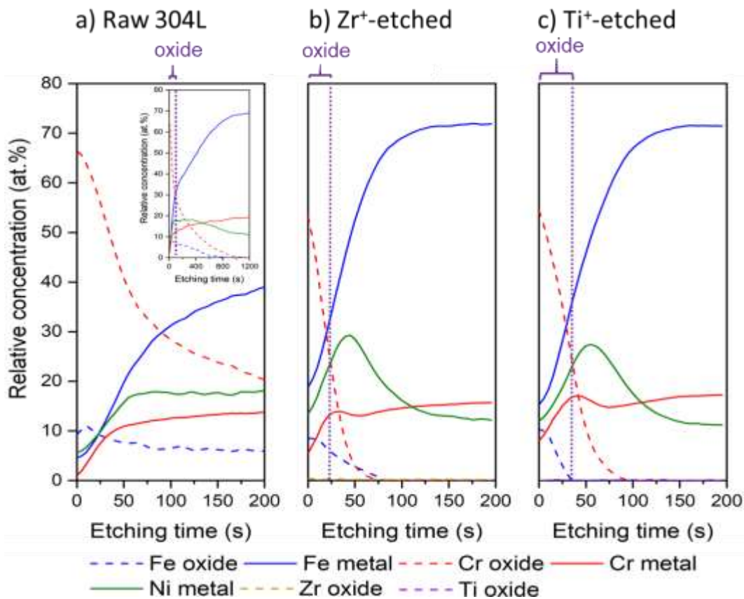
Figure 23: XPS depth profiles of (a) 304L steel and (b) Zr + - and (c) Ti + -etched samples after 2 d of immersion in nitric acid (2.5 mol/L HNO 3 , 2.5 mol/L NaNO 3 and 2 g/L Fe(NO 3 ) 3 ) solution at 110 °C.
