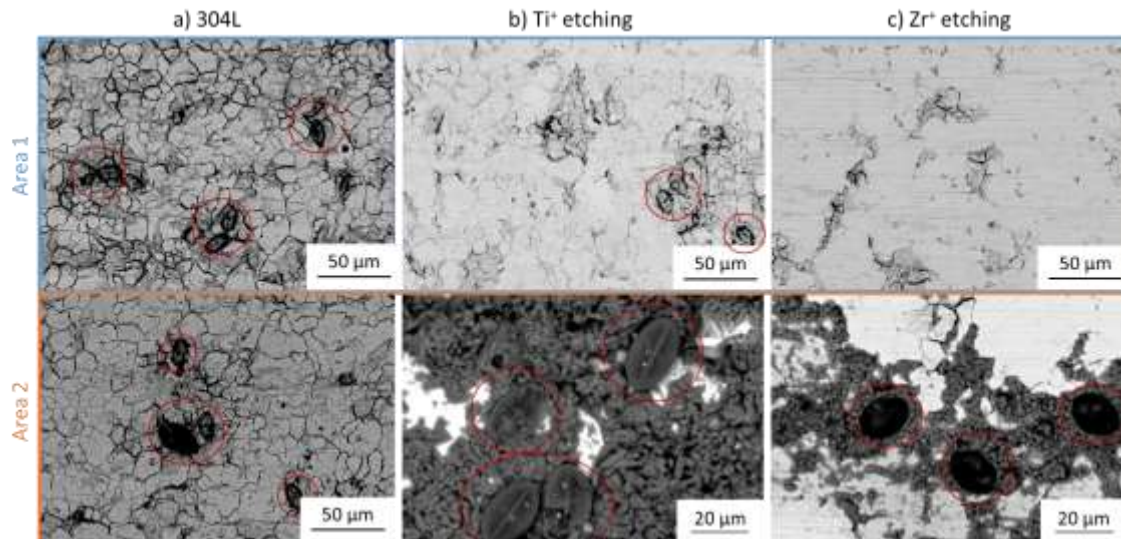
Figure 34: SEM-BSE micrographs on two different areas of the surface of the a) 304L steel, b) Ti^+ - and c) Zr^+ -etched substrates after 56 d of immersion in Cherbourg natural seawater.
