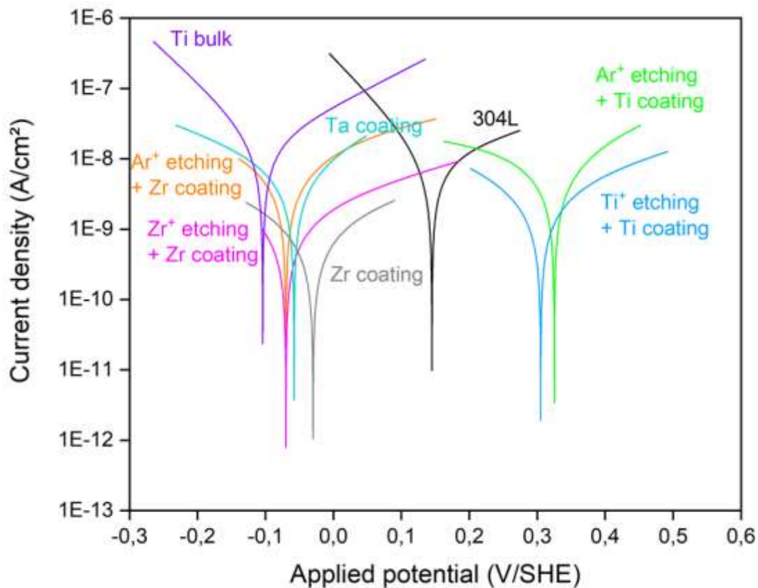
Figure 41: Potentiodynamic polarization curves of the initial and etched 304L steel samples and, the etched and metallic bond coat deposited samples in a 3.56 wt.% NaCl solution at ambient temperature after 6 h of immersion.
