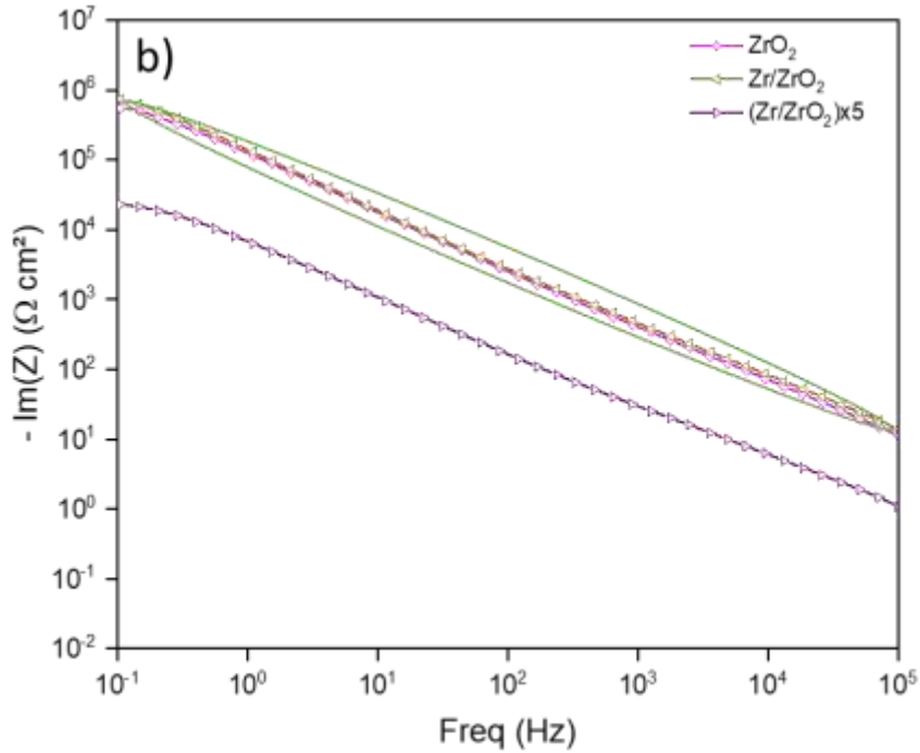
Figure 2: Imaginary part of the impedance as a function de frequency of a) Ti- and b) Zr-based coatings after immersion in a nitric acid (2.5 mol/L HNO 3 , 2.5 mol/L NaNO 3 and 2 g/L Fe(NO 3 ) 3 ) solution at 110°C – focus on single slope curves.
