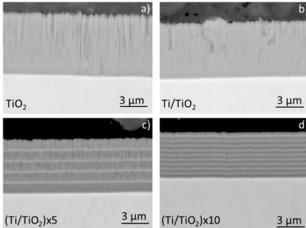
Figure 2: SEM-BSE images of cross-sections of a) monolayer \text{TiO}_2 , b) bilayer \text{Ti/TiO}_2 , c) (\text{Ti/TiO}_2)\times 5 and d) (\text{Ti/TiO}_2)\times 10 coatings.
