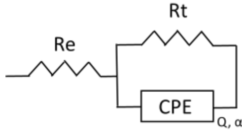
Figure 37: Equivalent electrical circuit of the initial and etched and metallic bond coat deposited samples in a nitric acid (2.5 mol/L \text{HNO}_3 , 2.5 mol/L \text{NaNO}_3 and 2 g/L \text{Fe}(\text{NO}_3)_3 ) solution at 110°C.
