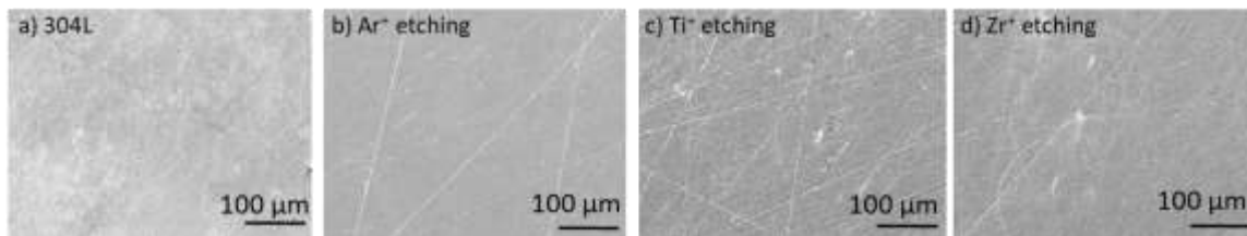
Figure 26: SEM-SE micrographs of the 304L and etched samples after electrochemical measurements in a 3.56 wt.% NaCl solution at ambient temperature.
