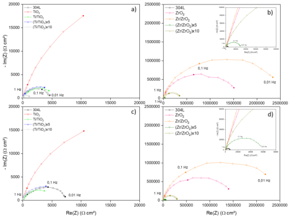
Figure 12: Nyquist diagram at open potential after 6 h for a) Ti-based, b) Zr-based coatings and after 2 d in a nitric acid (2.5 mol/L \text{HNO}_3 , 2.5 mol/L \text{NaNO}_3 and 2 g/L \text{Fe}(\text{NO}_3)_3 ) solution at 110°C for c) Ti-based and d) Zr-based coatings.
