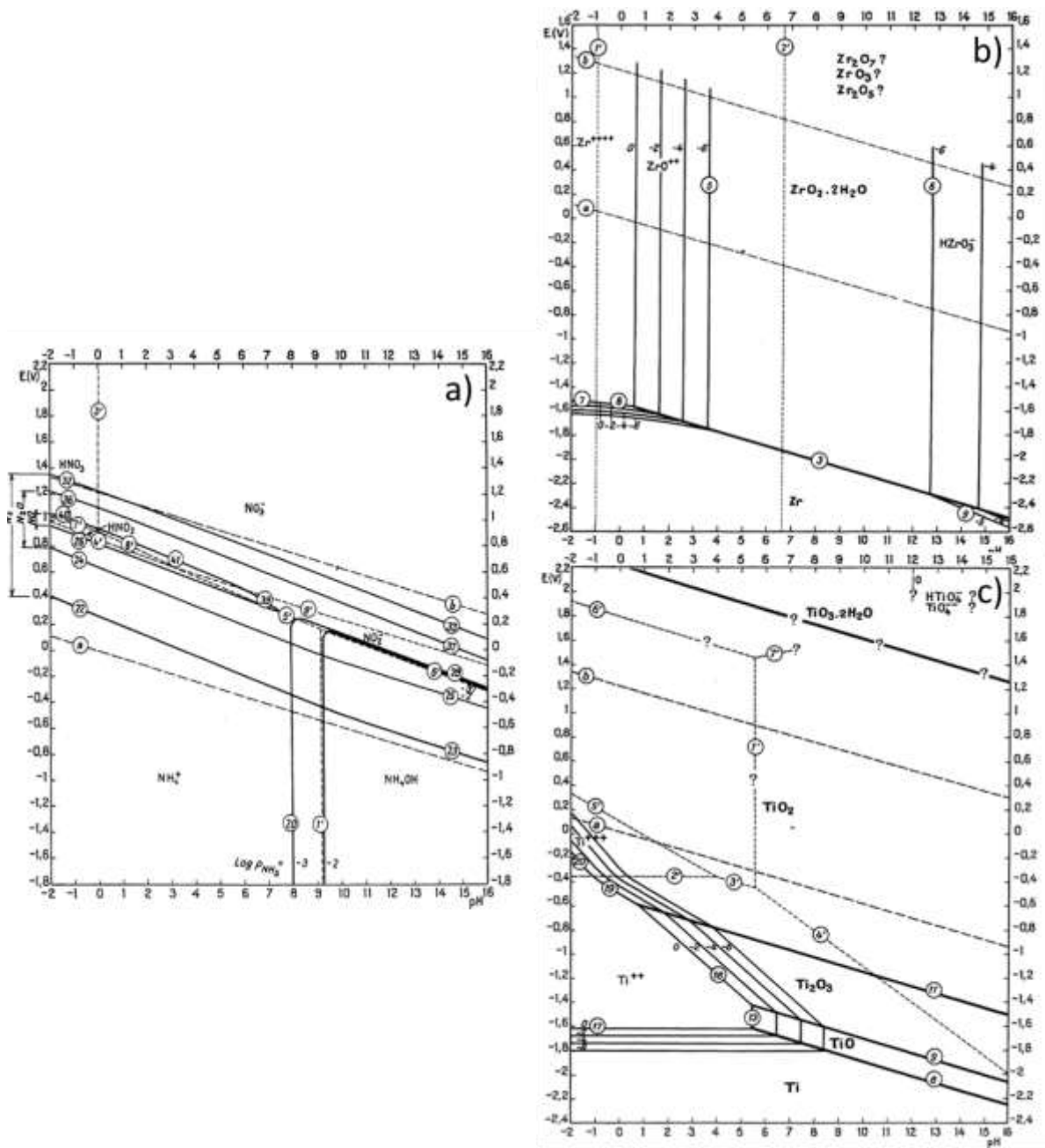
Figure 21: Pourbaix diagrams of a) N, b) Zr and c) Ti in H 2 O at 25 °C, from [131].
