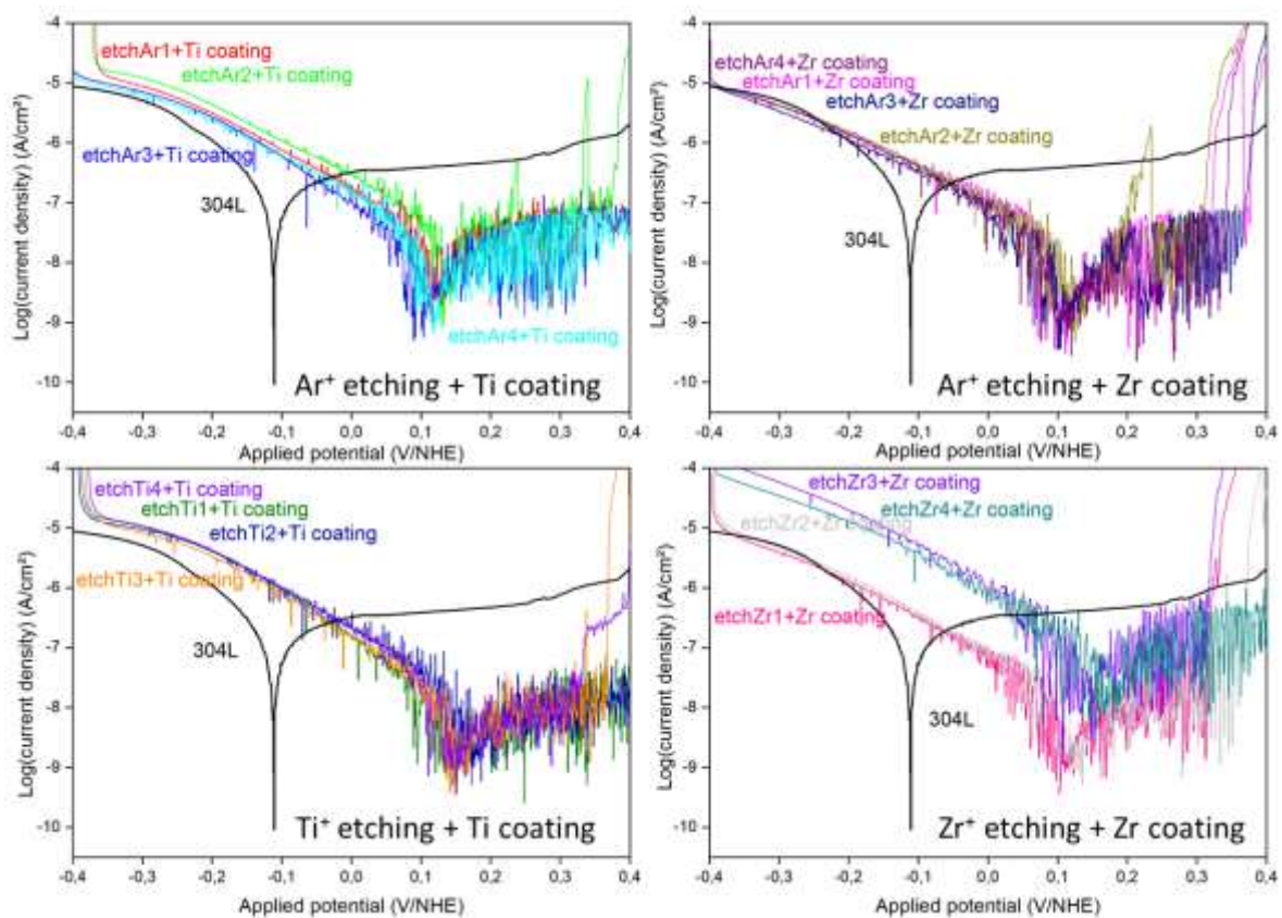
Figure 1: Comparison of anodic polarization curves for bare 304L and coated samples in a 5 wt% NaCl solution
