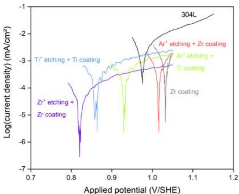
Figure 35: Potentiodynamic polarization curves of the 304L steel and the etched and metallic bond coat deposited samples in a nitric acid (2.5 mol/L \text{HNO}_3 , 2.5 mol/L \text{NaNO}_3 and 2 g/L \text{Fe}(\text{NO}_3)_3 ) solution at 110 °C after 6 h of immersion.
