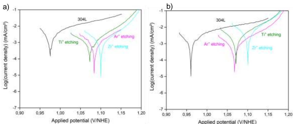
Figure 2: Anodic polarization curves of etched samples in a nitric acid solution at boiling temperature (2.5 mol/L HNO 3 , 2.5 mol/L NaNO 3 , 2 g/L Fe(NO 3 ) 3 at 110°C) after a) 6 h and b) 2 days compared to bare 304L before etching optimization
