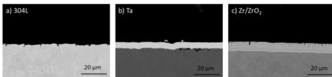
Figure 19: SEM-BSE micrographs of the cross-section of a) initial 304L steel, b) Ta and c) Zr/ZrO 2 coatings after 9 d in a nitric acid (2.5 mol/L HNO 3 , 2.5 mol/L NaNO 3 and 2 g/L Fe(NO 3 ) 3 ) solution at 110°C.
