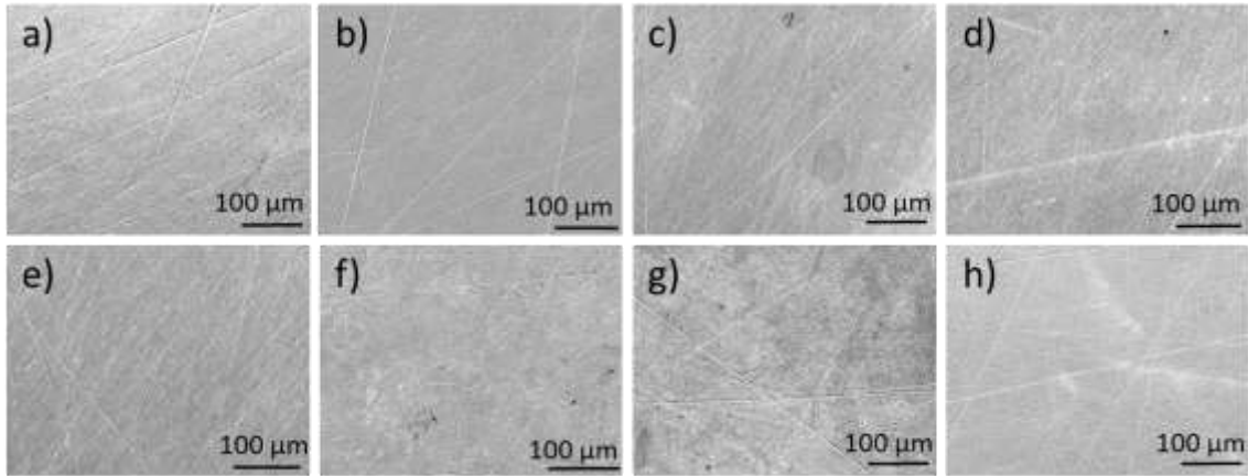
Figure 21: SEM-SE micrographs of the 304L as well as \text{Ar}^+ -, \text{Ti}^+ -, and \text{Zr}^+ -etched samples before (a, b, c, d) and after (e, f, g, h) electrochemical measurements in a nitric acid (2.5 mol/L \text{HNO}_3 , 2.5 mol/L \text{NaNO}_3 and 2 g/L \text{Fe}(\text{NO}_3)_3 ) solution at 110°C.
