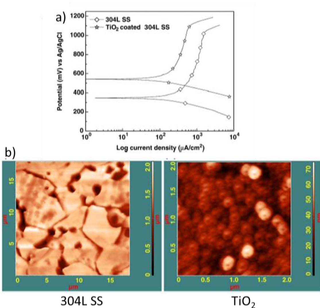
Figure 26: a) Potentiodynamic polarization curves for initial and TiO 2 coated 304L SS in 8 mol/L HNO 3 at room temperature (Ag/AgCl electrode) and b) AFM surface morphology after potentiodynamic polarization, from [151].
