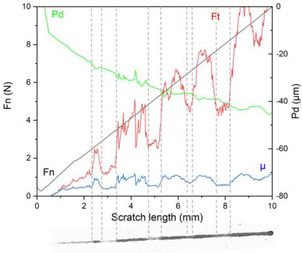
Figure 14: Evolution of the parameters ( F_n , F_t , P_d and \mu ) vs. the scratch length and comparison with the SEM-BSE observation of this scratch performed on Ar + -etched and Zr-coated sample.
