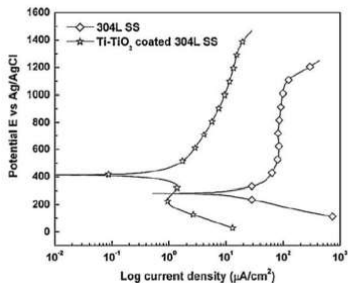
Figure 19: Potentiodynamic polarization curves of initial 304L and Ti/TiO 2 coating in 8 mol/L \text{HNO}_3 at room temperature (Ag/AgCl electrode), from [57].
