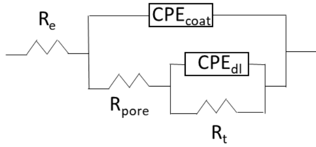
Figure 4: Equivalent electrical circuit of the TiO_2 , Ti/TiO_2 and (Zr/ZrO_2)_x5 coating systems in a nitric acid (2.5 mol/L HNO_3 , 2.5 mol/L NaNO_3 and 2 g/L Fe(NO_3)_3 ) solution at 110°C.
