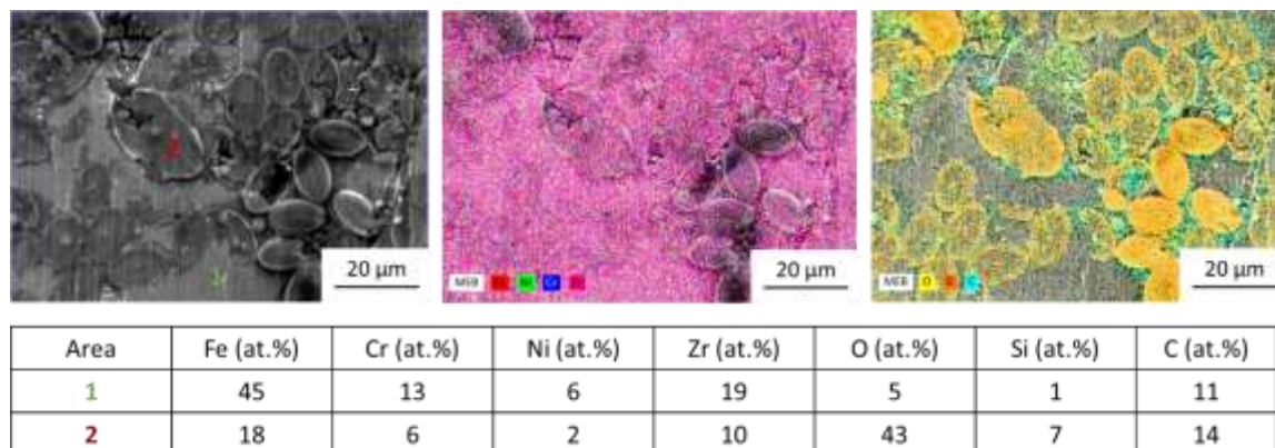
Figure 49: SEM-SE EDX analysis at an area of the Zr + -etched + Zr-coated sample showing biofilm residue after 56 d of immersion in Cherbourg seawater.
