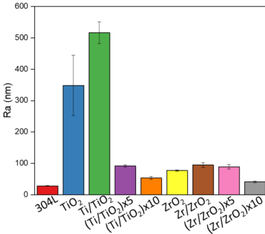
Figure 8: Surface roughness of the initial 304L substrate and all the oxide and multilayer-coated samples.
