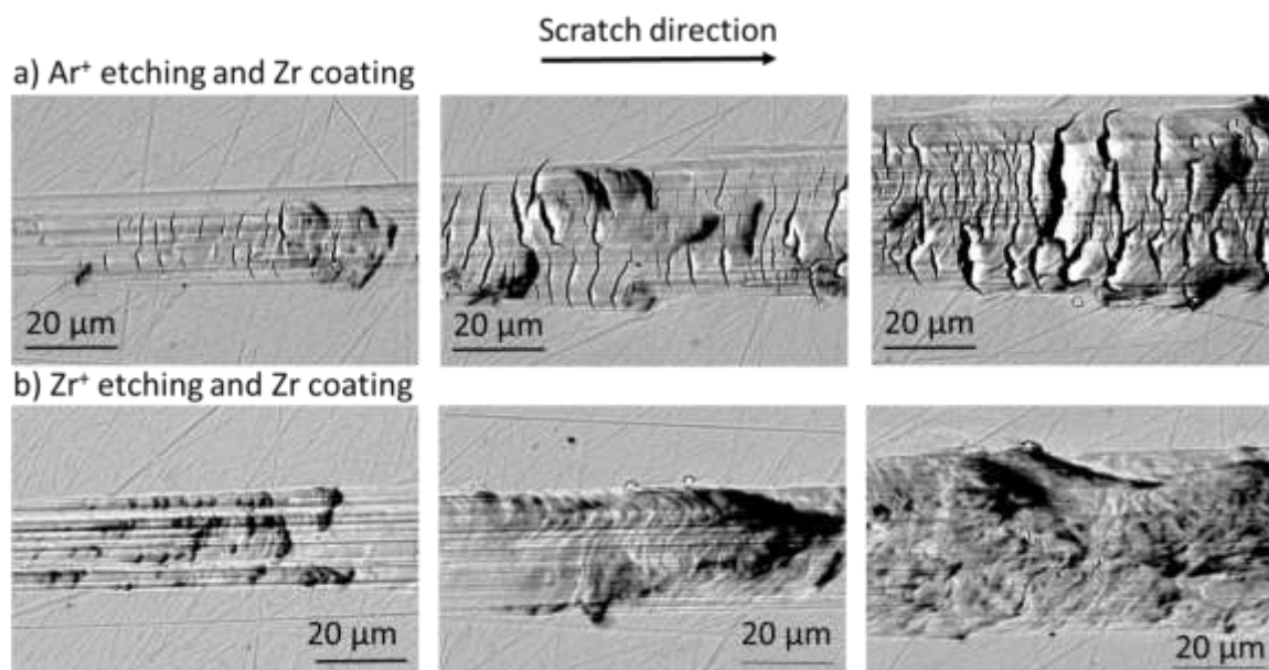
Figure 15: SEM-BSE micrographs of scratch testing track of a) \text{Ar}^+ -etched and Zr-coated sample and b) \text{Zr}^+ -etched and Zr-coated sample at different locations.
