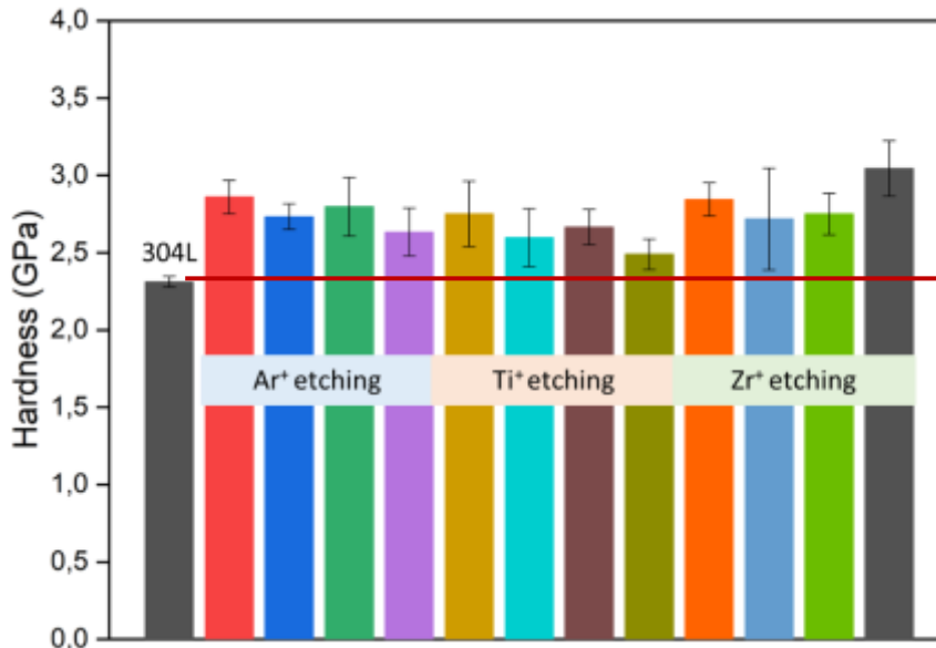
Figure 3: Hardness measurements of etched samples compared to 304L substrate obtained by nanoindentation technique
