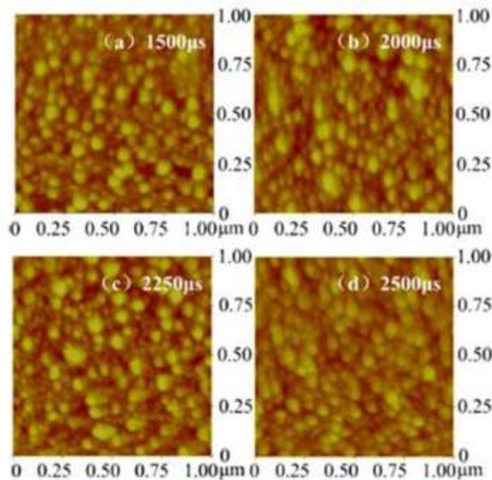
Figure 24: AFM images of ZrO_2 films prepared with various pulse-off time of a) 1500 \mu s , b) 2000 \mu s , c) 2250 \mu s and 2500 \mu s from [145].
