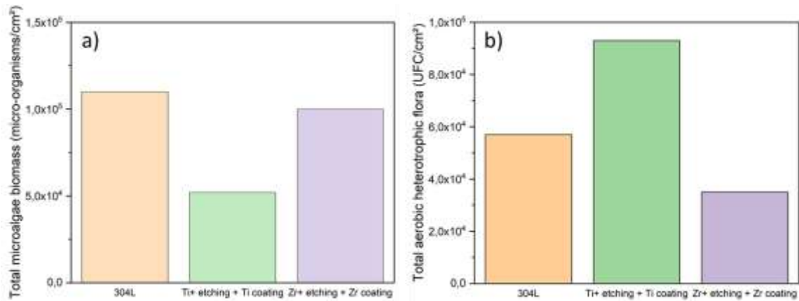
Figure 47: Results of microbiological analyses indicating the a) total microalgae biomass and b) total aerobic heterotrophic flora after 56 d of immersion in Cherbourg seawater.
