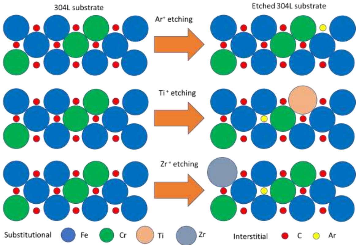
Figure 5: Schematic drawing in 1D of the substrate surface structure after a) \text{Ar}^+ , b) \text{Ti}^+ and c) \text{Zr}^+ etching.
