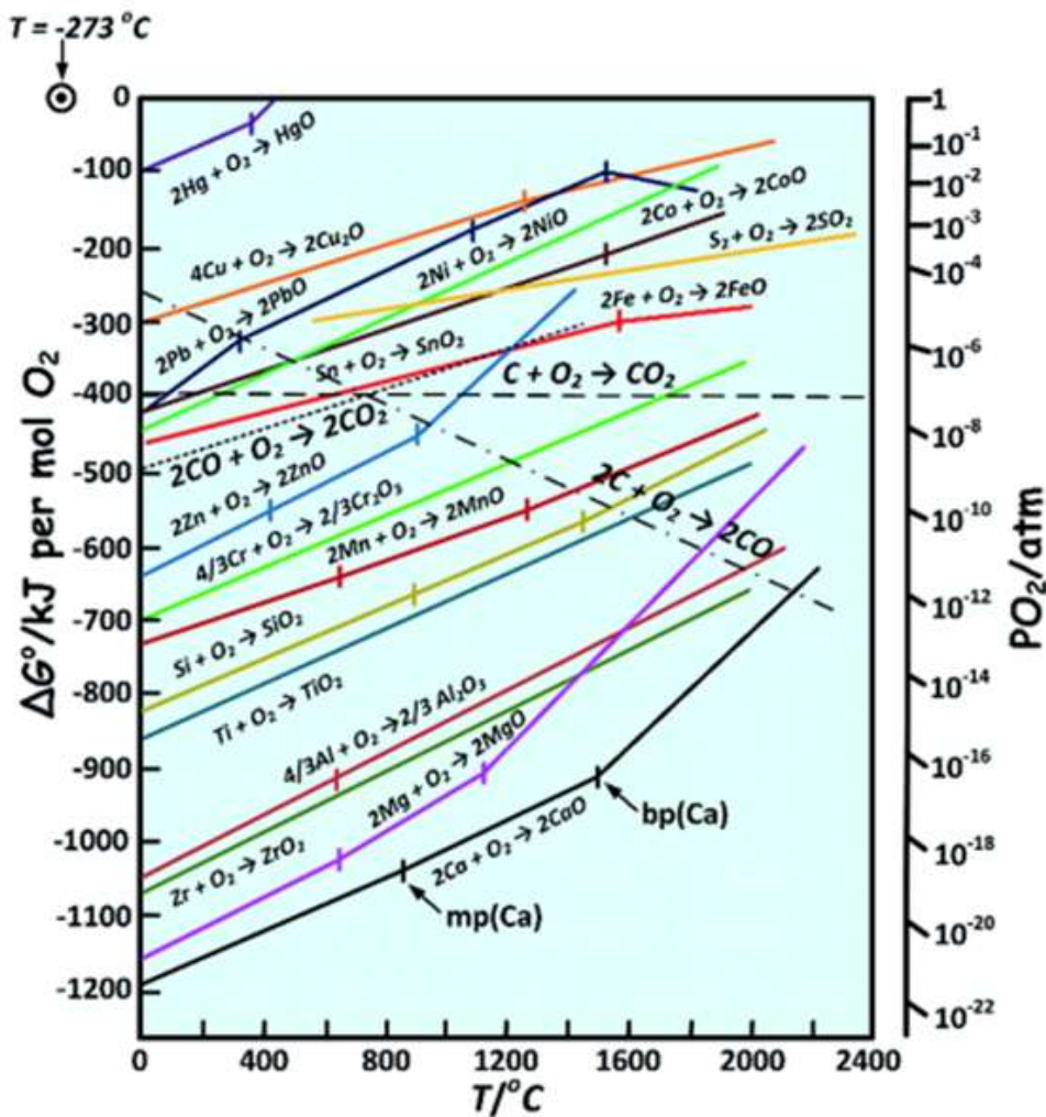
Figure 20: Ellingham diagram for oxides, from [130].
