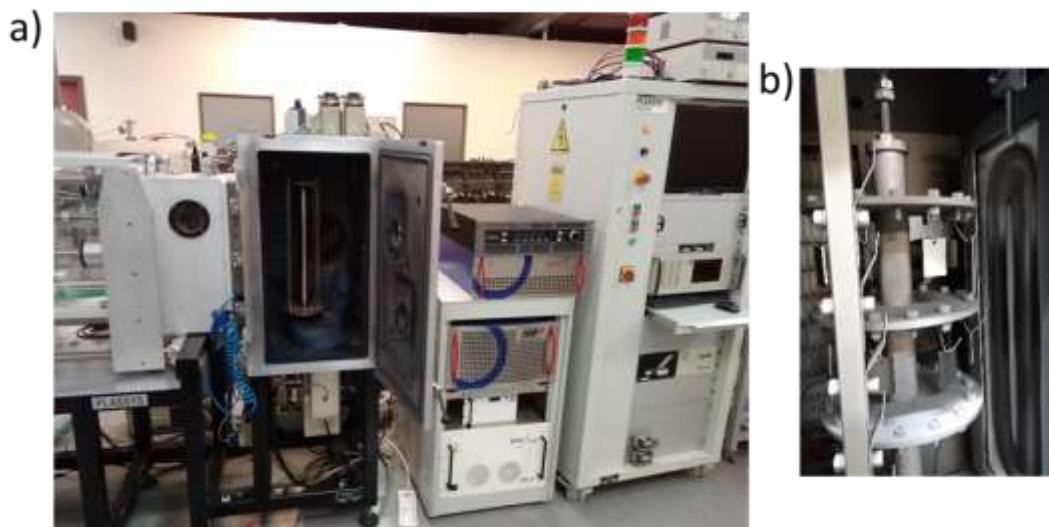
Figure 3: Photographs of a) the DEPHIS deposition chamber and b) the substrate-holder.
