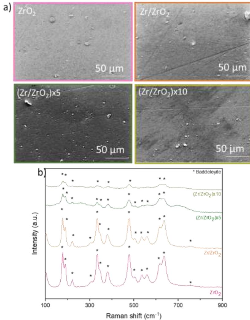
Figure 15: a) SEM-SE surface observation and b) Raman spectra of Zr-based coatings after 2 d in a nitric acid (2.5 mol/L \text{HNO}_3 , 2.5 mol/L \text{NaNO}_3 and 2 g/L \text{Fe}(\text{NO}_3)_3 ) solution at 110°C.
