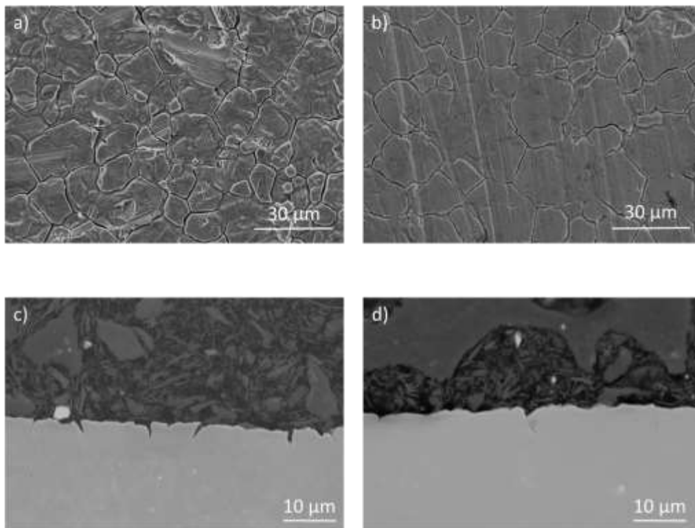
Figure 28: SEM-SE micrographs of surface of a) initial 304L steel and b) Zr + -etched sample and cross-section of c) 304L steel and d) Zr + -etched sample after 9 d of immersion in a nitric acid (2.5 mol/L HNO 3 , 2.5 mol/L NaNO 3 and 2 g/L Fe(NO 3 ) 3 ) solution at 110 °C.
