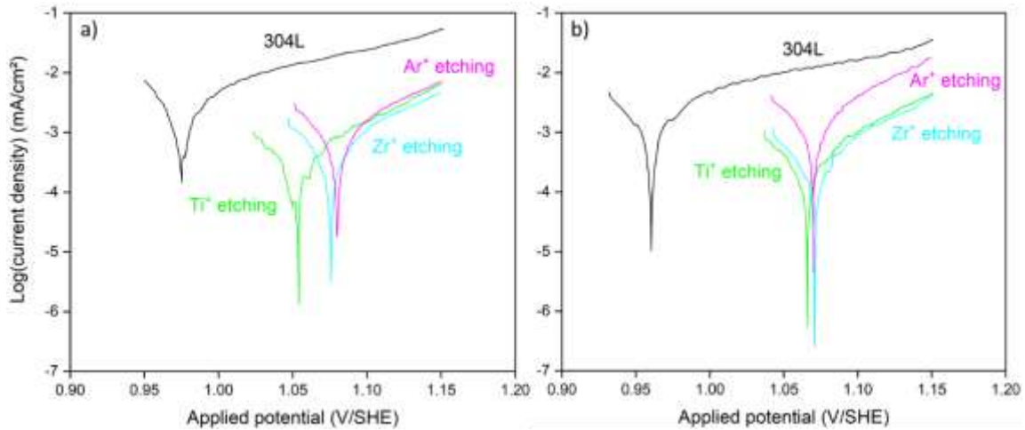
Figure 19: Potentiodynamic polarization curves of initial 304L and etched samples in a nitric acid (2.5 mol/L \text{HNO}_3 , 2.5 mol/L \text{NaNO}_3 and 2 g/L \text{Fe}(\text{NO}_3)_3 ) solution at 110°C after (a) 6 h and (b) 2 d of immersion.
