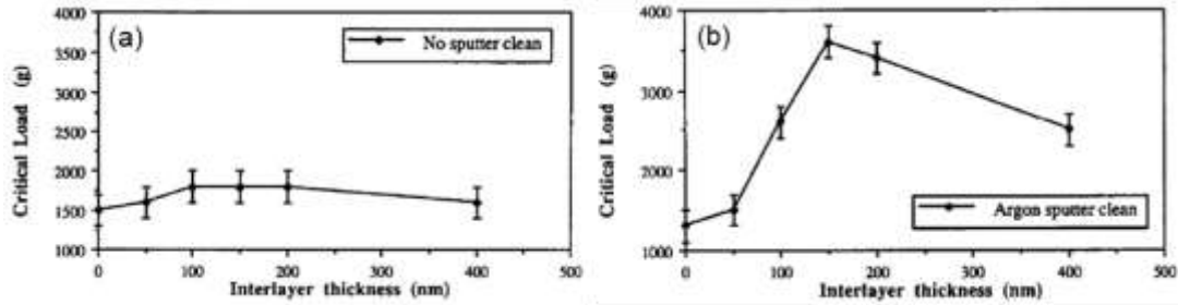
Figure 9: Variation of critical load for coating spallation with Ti interlayer thickness for 2 \mu\text{m} TiN coatings on stainless steel: (a) no sputter clean and (b) sputter clean in argon, from [54].
