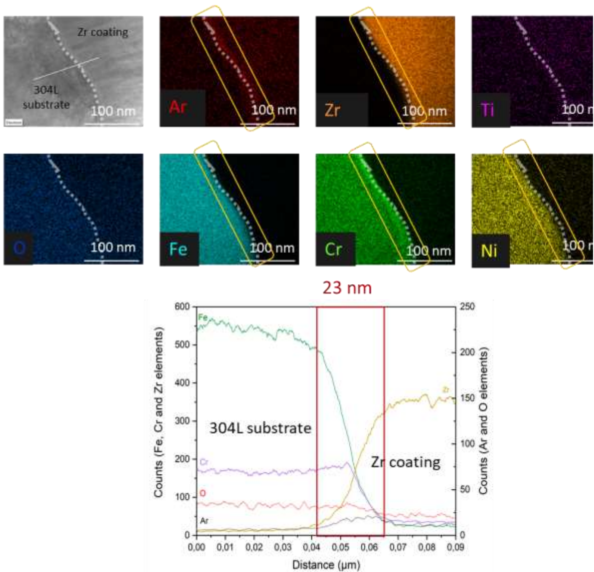
Figure 2: a) TEM mapping and b) TEM profile of an argon-etched and Zr-deposited sample and estimation of the interface thickness
