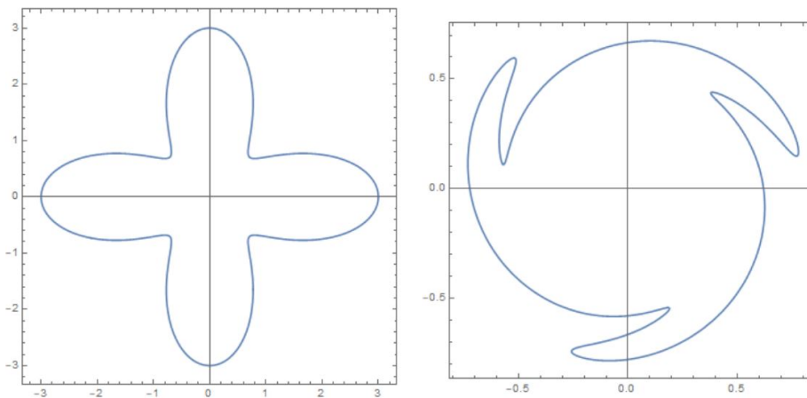
FIGURE 3.5 – Plot for b(x) = (2 + \cos(8\pi x))e^{i2\pi x} (left), and b(x) = \frac{\exp\left(2i\pi\left(x + \frac{1}{8}\cos(6\pi x)\right)\right)}{\frac{3}{2} + \frac{1}{4}\cos(6\pi x)} (right), with x \in [0, 1] .
