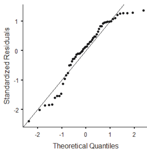
Figure G. QQ plot of the stroke orientation variable in the delayed recall trial
