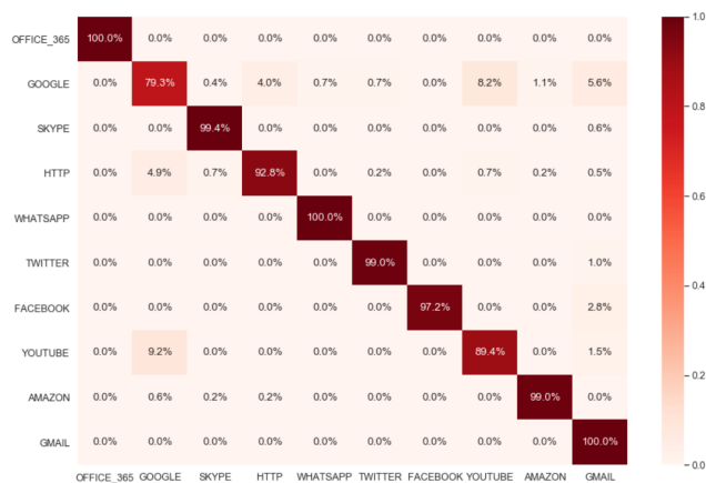
(b) Confusion matrix for Autoencoder
