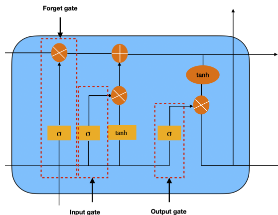
Figure 2.14: LSTM (Long Short-Term Memory)
