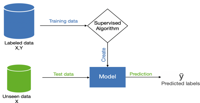
Figure 2.2: Training process of supervised learning algorithm
