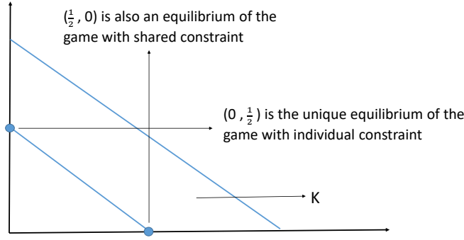
Figure 1.4: One equilibrium in individual constraints, an infinity of equilibria in shared constraint
