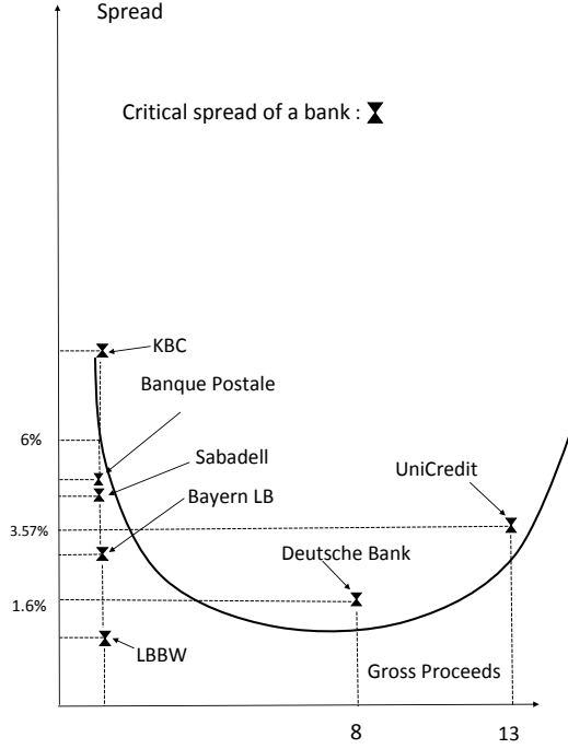
Figure A.4: Spread as a U-shaped function and critical spread
