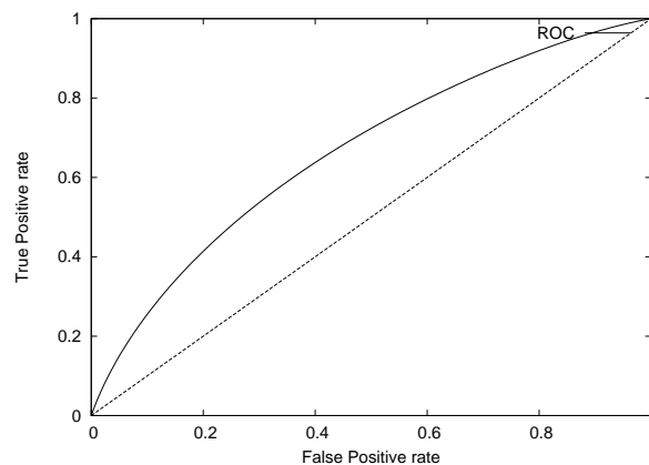
FIGURE 2.6 – Courbe ROC.
