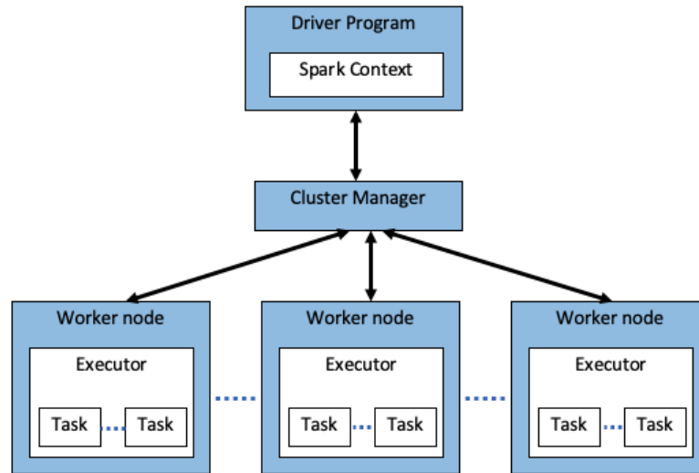
FIGURE 6.2 – Architecture de Apache Spark.
