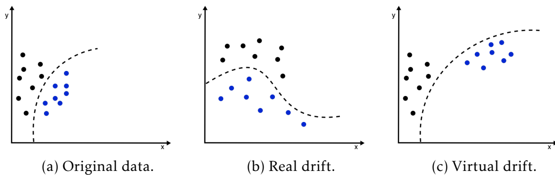
FIGURE 5.1 – Types de concept drift.
