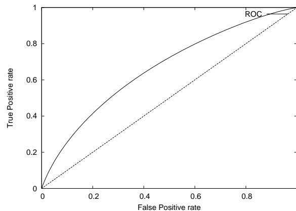
FIGURE 2.6 – Courbe ROC.
