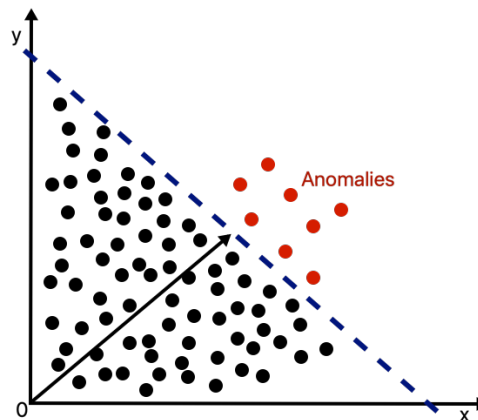
FIGURE 2.3 – One-Class Support Vector Machine.
