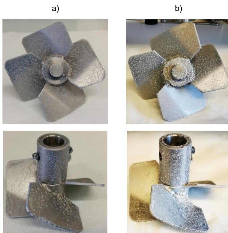
Figure 4.10 Bottom and side views of the material attached to the hydrofoil after the semi-batch reactions performed with different volumes of water a) 2.2 L and b) 1.6 L.
