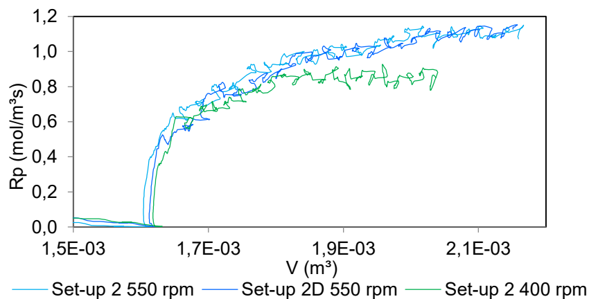
Figure 5.13 Semi-batch polymerization rates of reactions performed with different set-ups and speeds.
