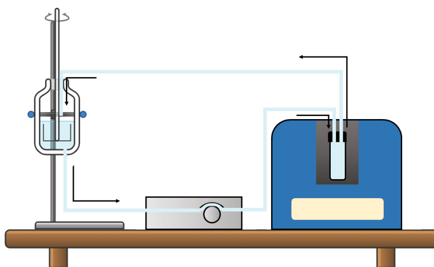
Figure 3.18 Schematic representation of the experiment by turbidity (Turbifixer).
