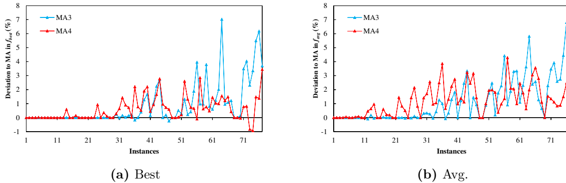
Figure 3.9 – Comparative results of MA with two variants MA3 (without operator M3) and MA4 (without operator M6) on the 77 instances of Sets S and L.
