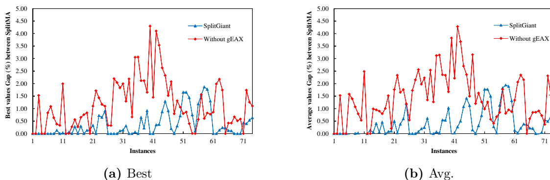
Figure 5.4 – Performance gaps of SplitGiant (with the giant tour crossover) and SplitMA1 (with the gEAX crossover disabled) compared to SplitMA on the 74 instances of Sets I and II (a positive gap indicates a deteriorating result).
