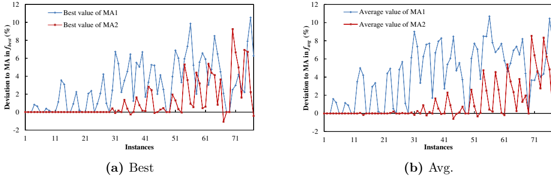
Figure 3.7 – Comparative results of MA with the variants MA1 (without mEAX) and MA2 (without the post-optimization) on the 77 instances of Sets \mathbb{S} and \mathbb{L}
