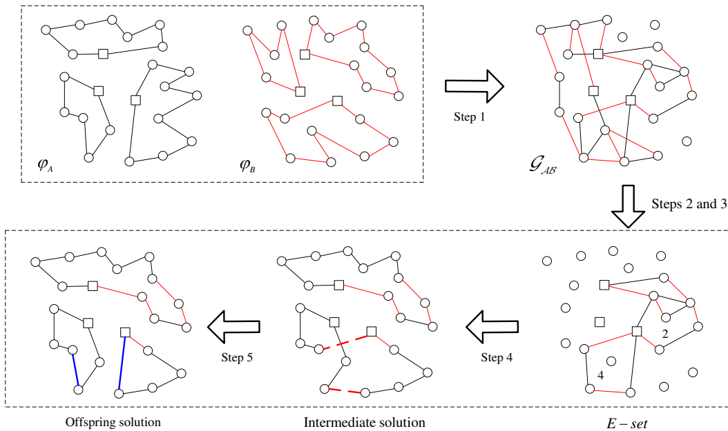
Figure 3.2 – Illustration of the mEAX crossover steps of the minmax multidepot mTSP
