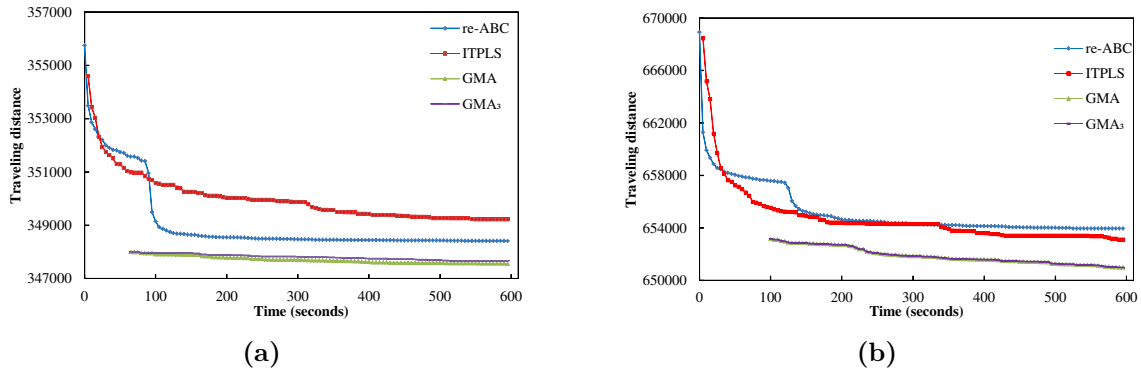
Figure 2.6 – Convergence charts (running profiles) of re-ABC, ITPLS, GMA and GMA 3 for solving two representative instances (gr431-25 and gr666-30). The results were obtained from 20 independent executions of each compared algorithms
