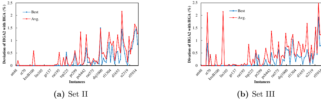
Figure 4.6 – Results of HGA2 (without mutation) in terms of deviation in percentage compared to the results of HGA (with mutation).
