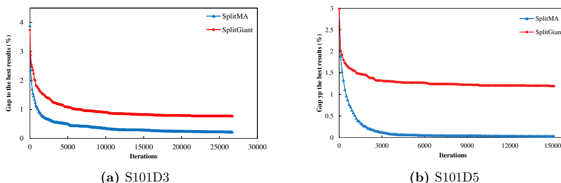
Figure 5.5 – Convergence charts of SplitMA and SplitGiant for solving two representative instances.
