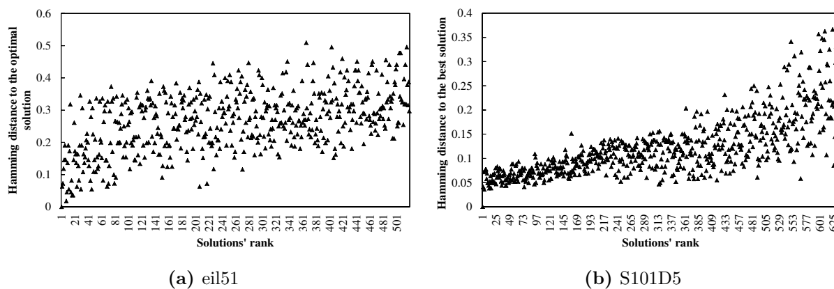
Figure 5.7 – Hamming distance between solutions and the best/optimal solution
