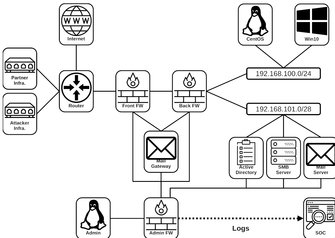
Figure 4.5 – High-level architecture of the lab environment.
