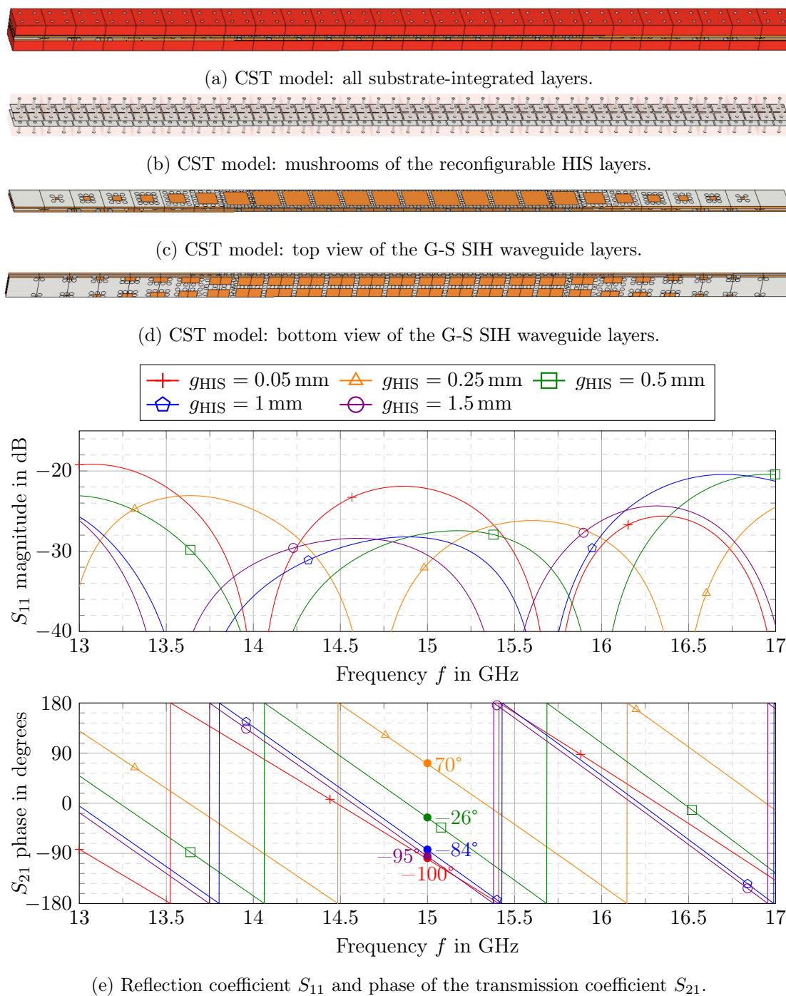
Figure 6.28: S-parameter of 10 chained unit cells as described in Fig. 6.19, with 8 tapered cells with the dimensions in Tab. 6.1. The waveguide is reconfigured by changing the gap g_{\text{HIS}} for both outer HIS layers.
