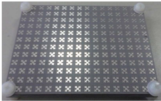
(a) Fractal frequency-selective surface [54].
