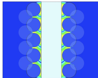
(c) Magnitude of the electric field in the leakage plane, with holes.
