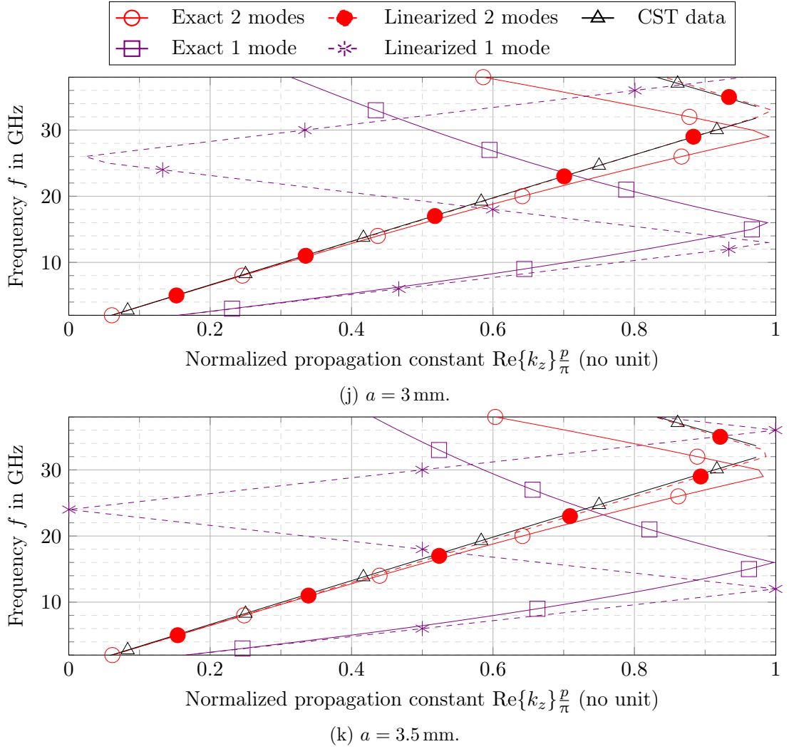
Figure 3.6: Brillouin diagram for the G-S structure with p = 4 mm, h = 0.5 mm, g = 0.1 mm and varying corrugation width a . The dispersion curve obtained with CST is compared with the 2-mode and 1-mode models. For both models, the true dispersion curve is compared to its linearized version (3.12) or (3.16). 50 harmonics are considered for each model.
