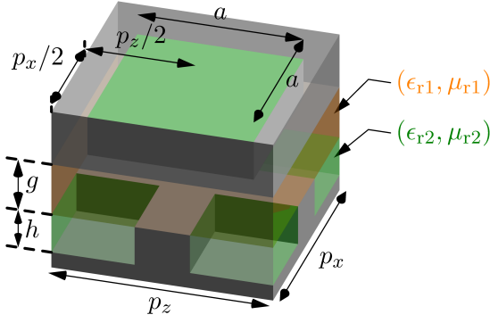
(a) Unit cell under study.
