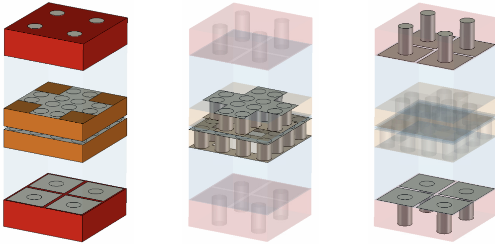
(a) CST unit cell model.
