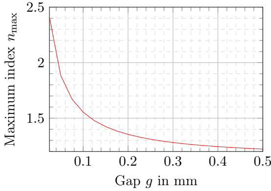
(c) Maximum achievable index as function of g .
