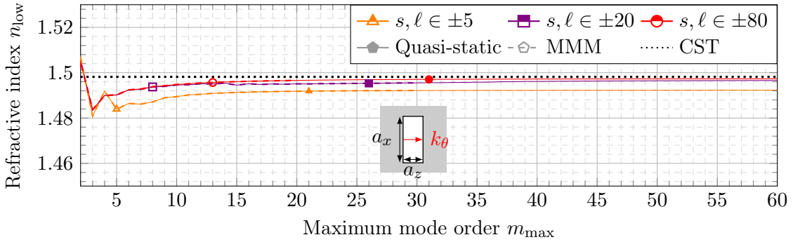
(b) a_z = 1.5 mm, a_x = 3.5 mm.
