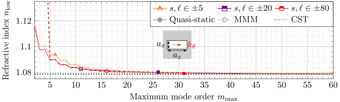
(c) a_z = 3.5 mm, a_x = 1.5 mm.
