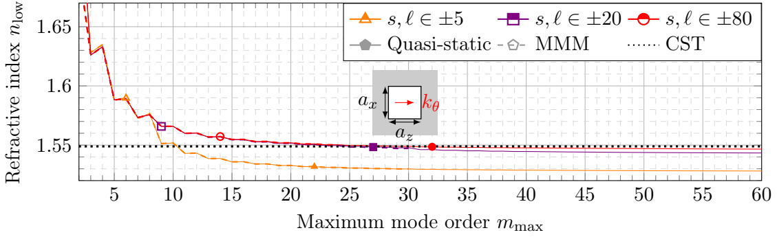
(a) a_z = a_x = 3 mm.
