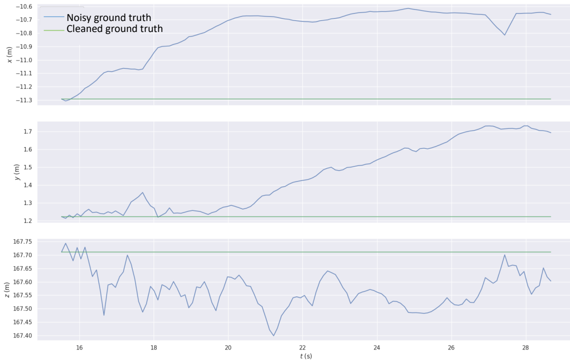
Figure 6.6 – Illustration of groundtruth pose noise
