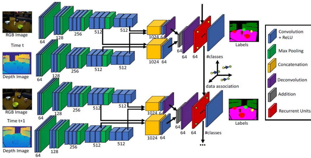
Figure 2.10 – Pipeline of [Xiang and Fox, 2017], features are extracted from RGB and depth images and used with current hidden state for segmentation and hidden state update.
