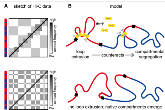
Fig. 1.14 Loop extrusion mechanism may compete with epigenomic-driven microphase separation. (A) Scheme of Hi-C signatures when both mechanisms are present (top, TADs and compartments) or with only microphase separation (bottom, only compartments). (B) Sketch of the mechanistic models when both mechanisms are considered (top) or when only epigenomic-driven interactions are accounted for (bottom). Adapted from [107].
