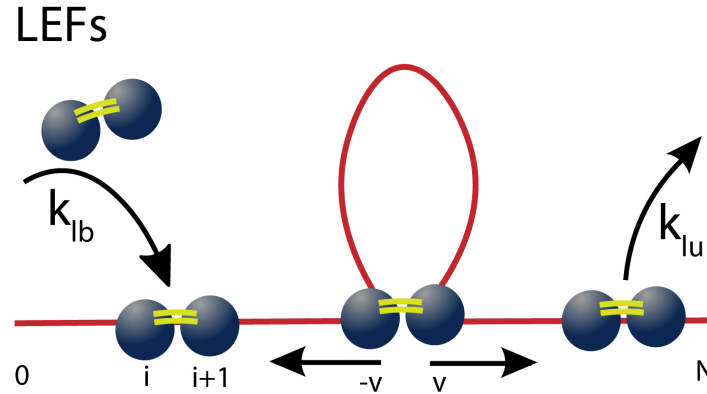
Fig. 2.3 Illustration of the loop extrusion model. Loop extruding factors (LEFs) can bind to the chromatin (in red) at position i, i+1 with a fixed rate k_{lb} and unbind at a rate k_{lu} . The two subunits of the LEFs move bidirectionally in opposite directions at velocity v leading effective extrusion of chromatin loops.
