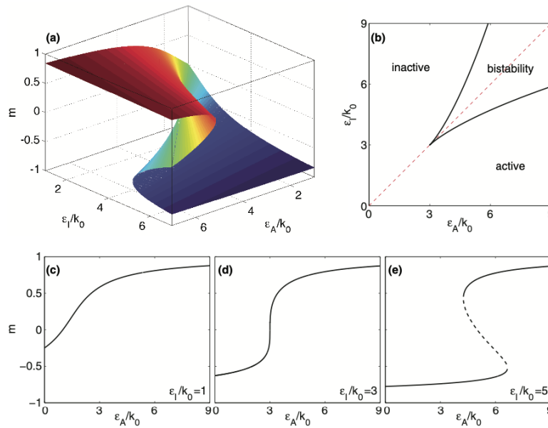
Fig. 1.7 3 states model (Fig. 1.4), asymmetric regime. (a) Cusp catastrophe surface representing the fixed points of the dynamical system as a function of \epsilon_A/k_0 and \epsilon_I/k_0 . (b) Stability diagram and boundaries between the mono- and bistable regions. (c)–(e) Bifurcation diagrams for m as a function of \epsilon_A/k_0 for fixed values of \epsilon_I/k_0 [(c) = 1, (d) = 3, (e) = 5]. Figure and legend from [22] (Figure 2).
