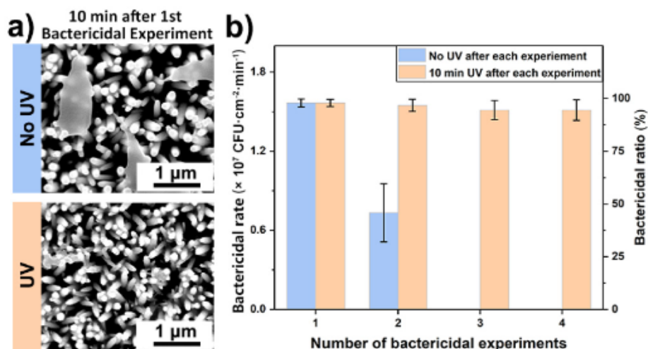
Figure IV. 15: Experimental evidences of the by photocatalytic degradation of the bacterial debris under UV light. SEM images of E. coli cells debris on hexagonal pyramid
