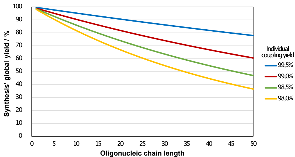
Figure 2.6: Theoretical global synthesis yield. The global yield depends on phosphoramidite individual coupling yield (colour-coded). The longer the oligonucleotide, the more the yield is dropping.
