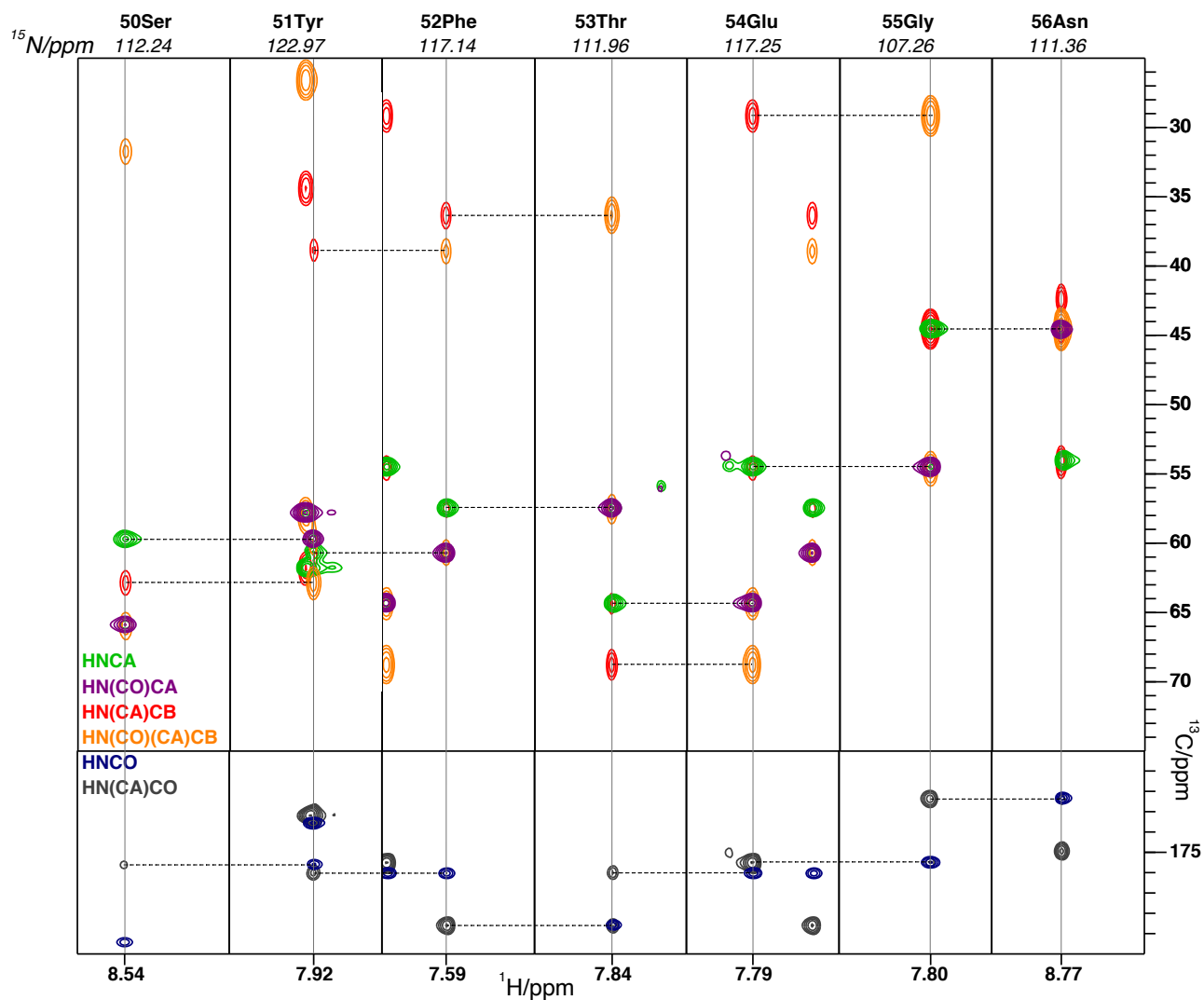
Figure 5.6: Lrp assignment strategy for sol-Llp residues S50-N56. Spectra strips (colour legend on figure) contain inter- and intra-residue C\alpha , C\beta and CO resonances for each NH groups, which ^{15}\text{N} frequency is written in italic. Dotted lines show the connexion between spectra while full vertical grey lines show the corresponding ^1\text{H} frequency observed in each strip.
