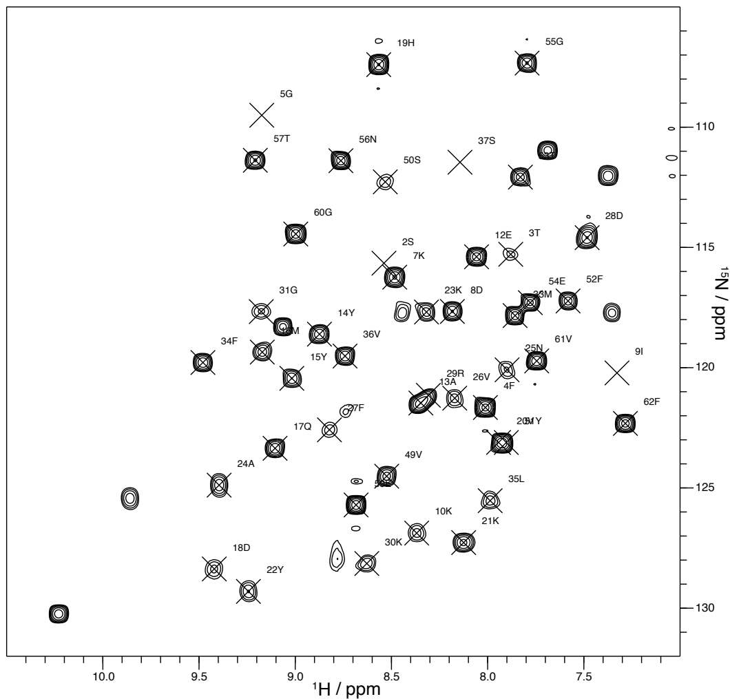
Figure 5.7: Llp ^1\text{H},^{15}\text{N} -HSQC spectrum, with assignment. Spectrum was recorded at 600 MHz and 303 K. Each peak position provides ^1\text{H} and ^{15}\text{N} chemical shifts for the protein amino groups. 47 of the 58 non-proline amino acids have been assigned, resulting in 76% completed assignment.
