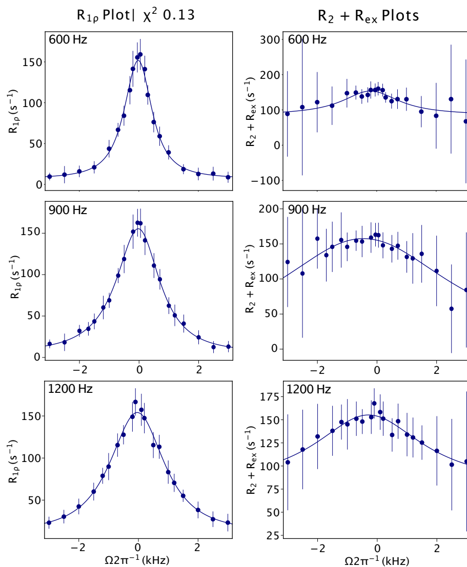
Figure 3.16: 19 F off-resonance R_{1\rho} of let-7 in interaction with LIN41 as a function of spinlock offset to the U9 resonance, at 600, 900 and 1200 Hz, 298 K and 600 MHz
