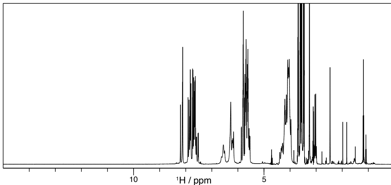
Figure 3.10: ^1\text{H} NMR spectrum of let-7 -U6F (600 MHz, 298 K).
