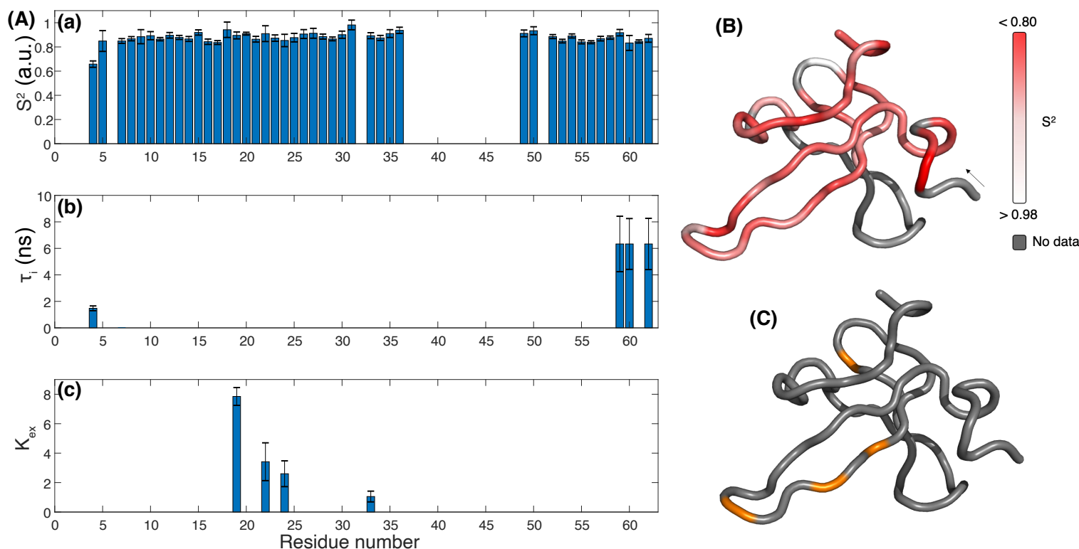
Figure 5.12: (A) sol-Llp model-free analysis using Tensor software: (a) order parameters for each backbone ^1\text{H} - ^{15}\text{N} vector; (b) corresponding \tau_i when fitted; and for models 3 or 4 (c) the corresponding exchange K_{ex} . (B) Order parameters repartition on Llp structure, the redder the more flexible is the residue (grey for no data); the arrow indicates the N-terminal. (C) Residues experiencing exchange are highlighted in orange on the structure.
