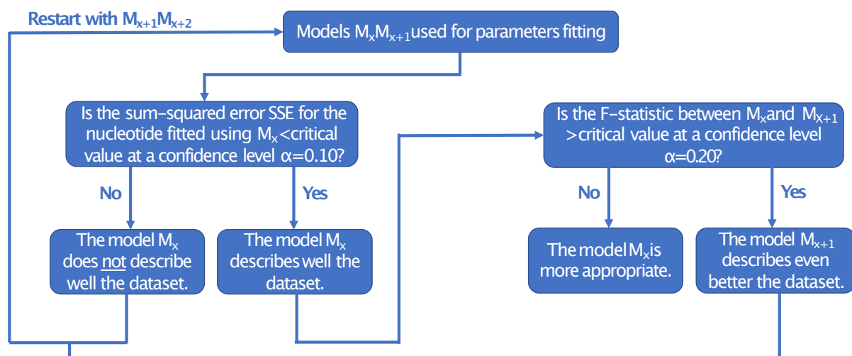
Figure 4.6: Scheme of the model selection by comparison of parameters fitting to the experimental data, in the model-free analysis.
