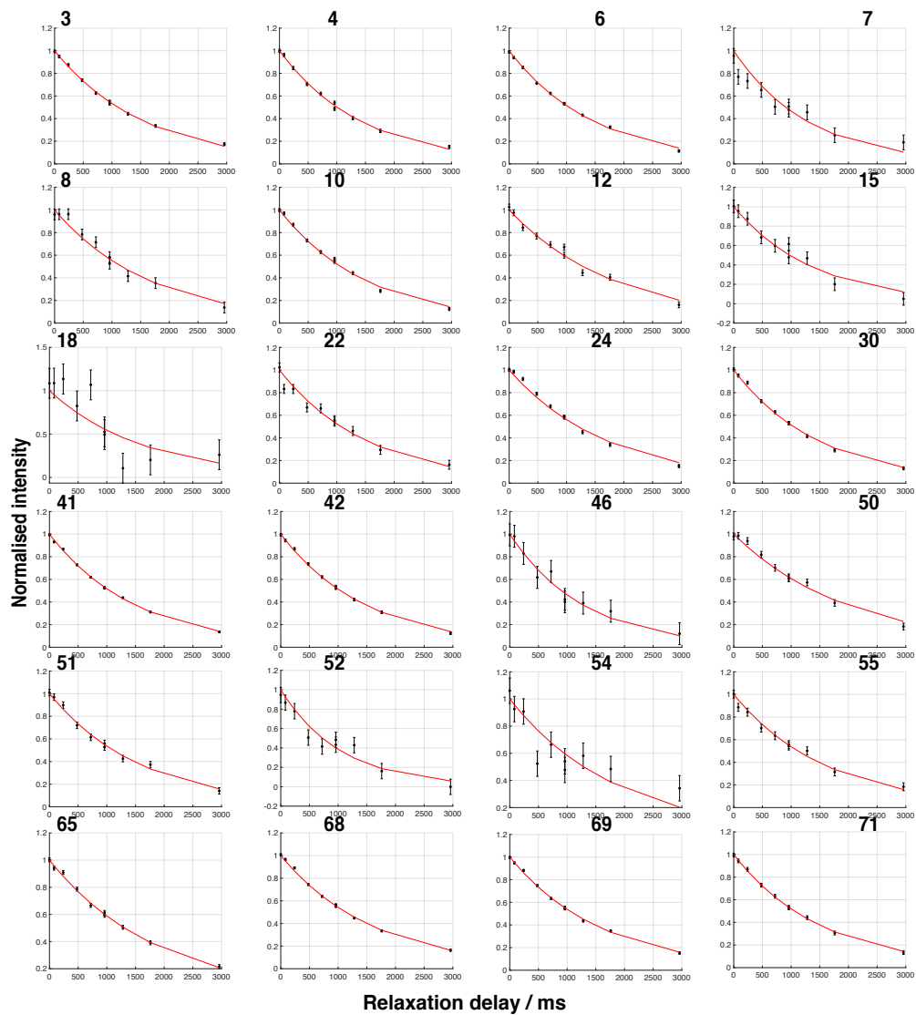
Figure 5.19: tRNA Phe ^{15}\text{N} site-specific longitudinal relaxation rates R_1 at 600 MHz and 310K.
