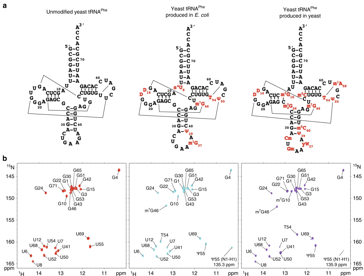
Figure 4.2: a) Structure and b) 1 H, 15 N-HSQC spectra comparison for unmodified and matured form of the yeast tRNA Phe . Reproduced with authorisation from [150].
