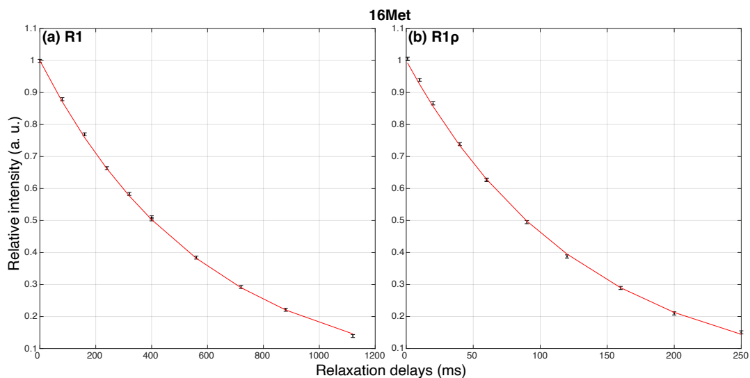
Figure 5.10: Intensity fluctuation of 16Met in ^1\text{H} , ^{15}\text{N} -HSQC spectra upon relaxation delay variation, for (a) R1 and (b) R1 \rho , at 600 MHz and 303 K.
