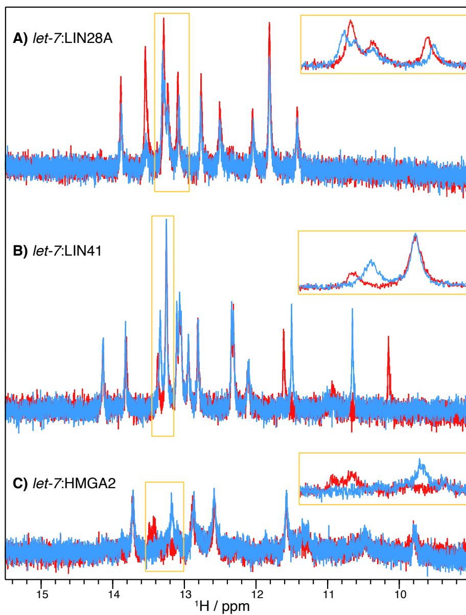
Figure 3.11: ^1\text{H} imino part of the NMR spectra of let-7 interaction with targets (A) LIN28A, (B) LIN41 and (C) HMGA2 (600 MHz, 298 K for LIN28A and LIN41, 280K for HMGA2). In each case, red spectra highlight the interaction between targets and let-7 labeled ^{19}\text{F} on 2'-U6, while light blues ones are samples containing ^{19}\text{F} 2'-U9 let-7 .
