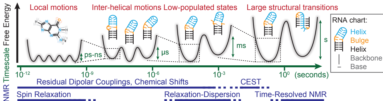
Figure 1.1: Typical motional timescales identifiable by NMR spectroscopy.
