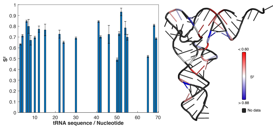
Figure 4.8: Order parameter determined by model-free analysis, plotted against the nucleotide sequence, and on structure.
