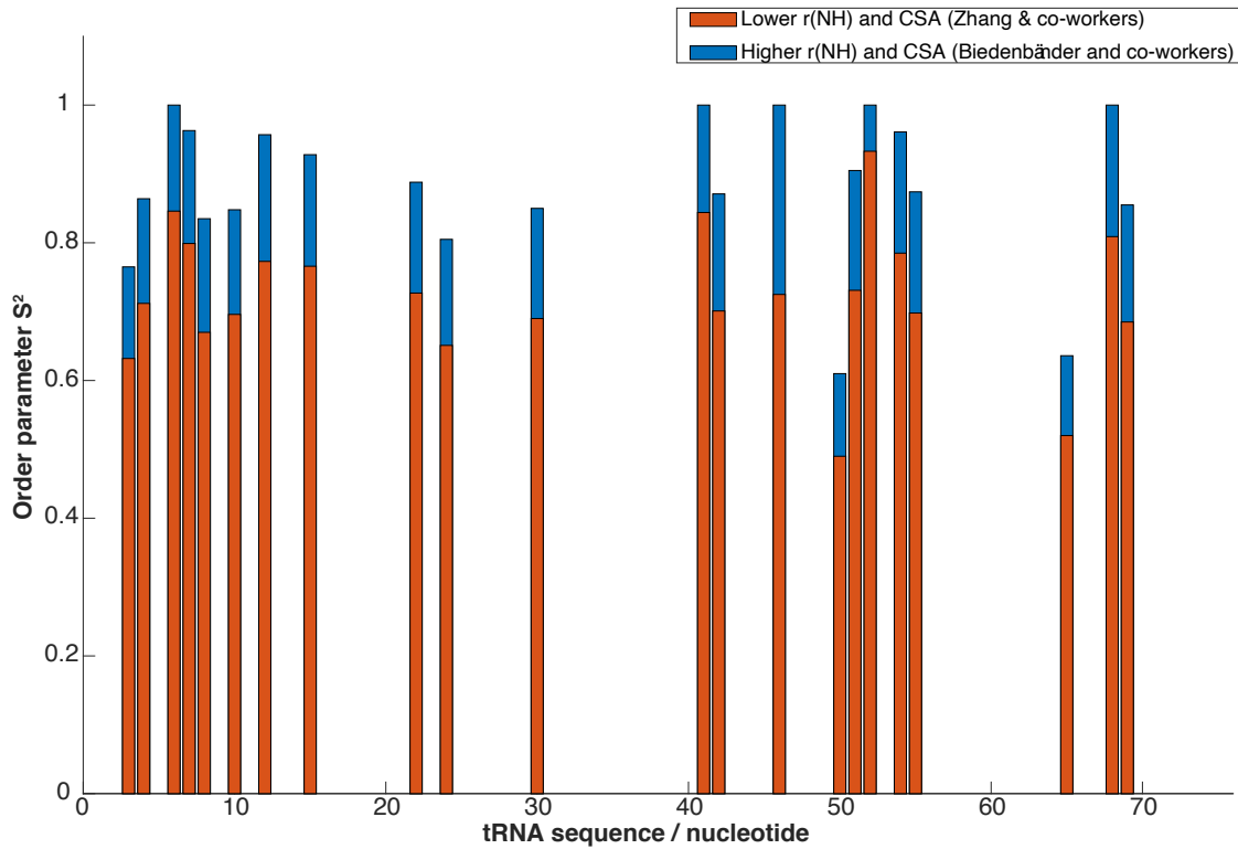
Figure 5.23: tRNA Phe model-free analysis using various CSA and r(NH) values from literature: order parameters are plotted for each nucleotide.
