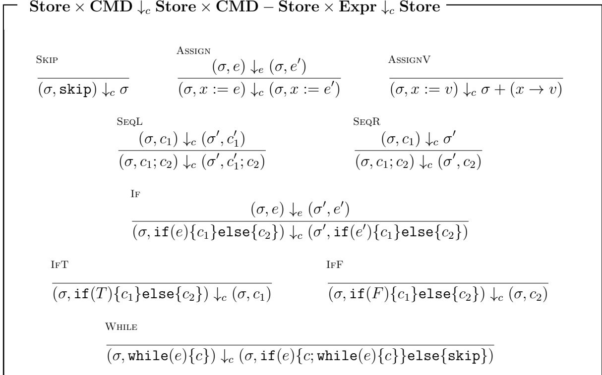
Figure 1.5: Small-Step commands evaluation.
