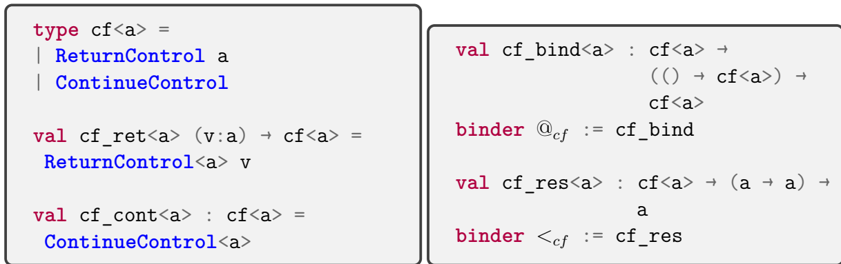
Figure 4.7: The controlFlow type with binders and setters
