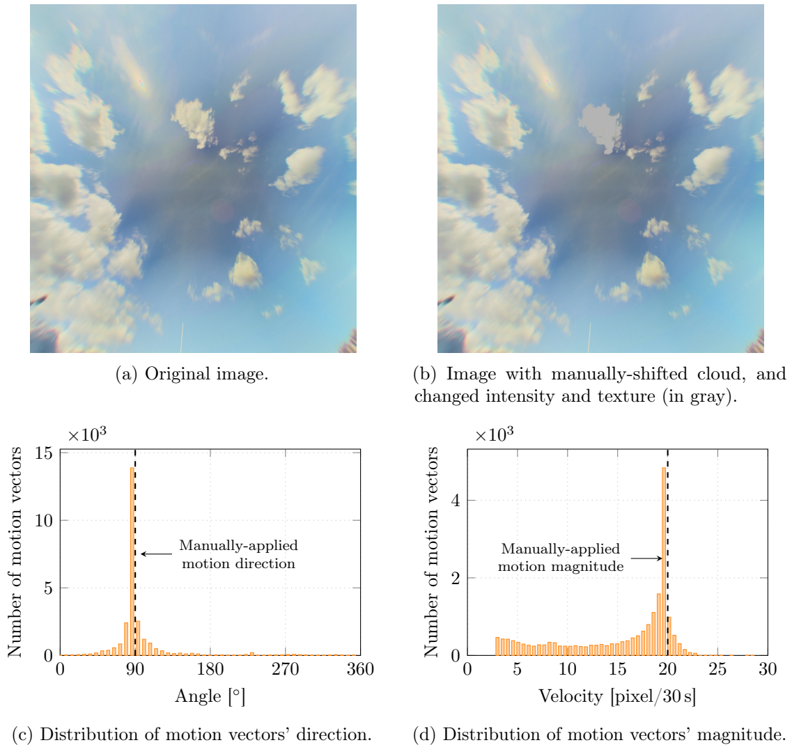
Figure 4.15: Cloud motion estimation: test case 2.
