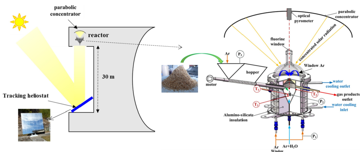
Figure 5.1: Solar reactor design [157].
