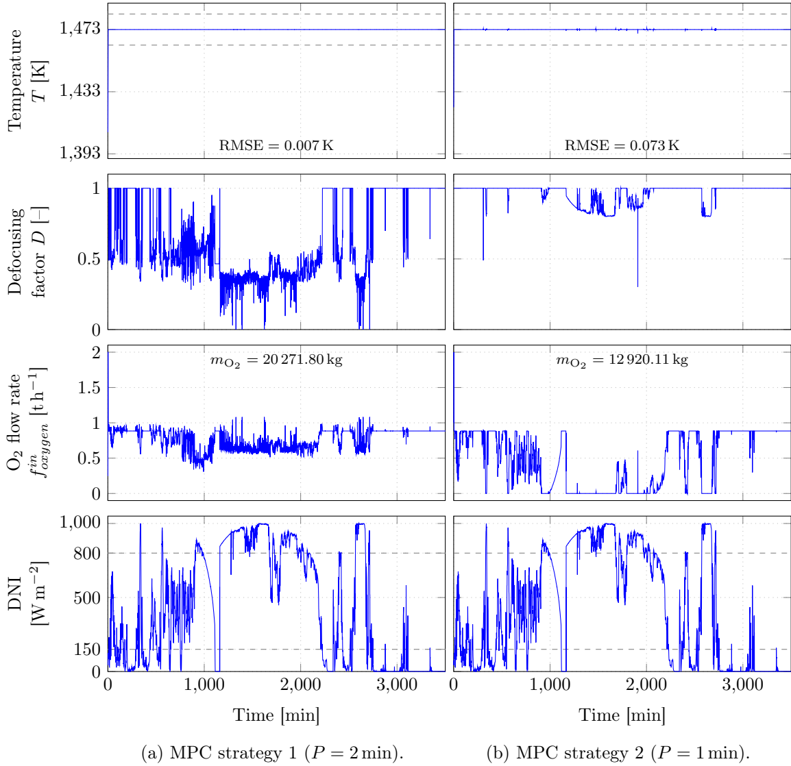
Figure 6.9: Case study: results of the two MPC strategies with perfect forecasts.
