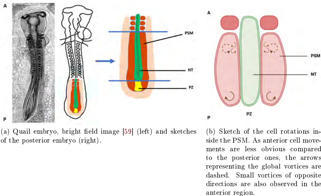
Figure 4.1 – Schematics of the tissues (a) and the cell movements (b). The notations A and P respectively denote the anterior and the posterior parts of the embryo.
