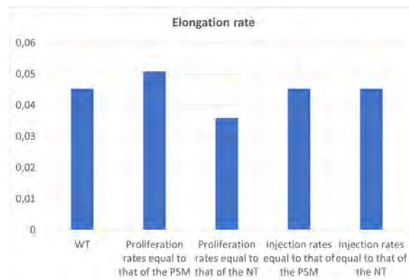
Figure 5.9 – Comparison of elongation rates (from left to right): in the wild type case, when proliferation rates are equal to that of the PSM, when proliferation rates are equal to that of the NT, when injection rates are equal to that of the PSM, when injection rates are equal to that of the NT. The y -axis is in unit \mu\text{m}/\text{s} .
