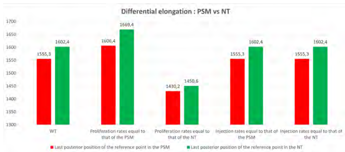
Figure 5.10 – Comparison of differential elongation. From left to right: in the wild type case, when proliferation rates are equal to that of the PSM, when proliferation rates are equal to that of the NT, when injection rates are equal to that of the PSM, when injection rates are equal to that of the NT. The y -axis unit in microns.
