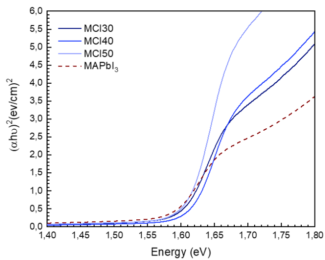
Figure S14: Tauc plot of elaborated PK films (deduced from their UV-visible absorption spectra)
