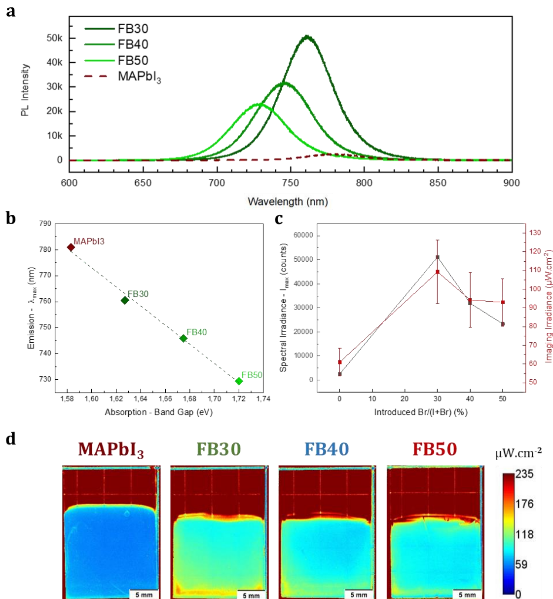
Figure 29: a) Photoluminescence spectra of the four elaborated films excited at 520 nm, b) the variation of \lambda_{max} as a function of the Band Gap when increasing the Br content in the conversion solution, c) the variation of I_{max} of the PL spectra and the average irradiance calculated from the PL images as a function of the Br percentage in the conversion solution, and d) the quantified PL images of the perovskite layers (the unit of calibration bar is \mu W \cdot cm^{-2} )
