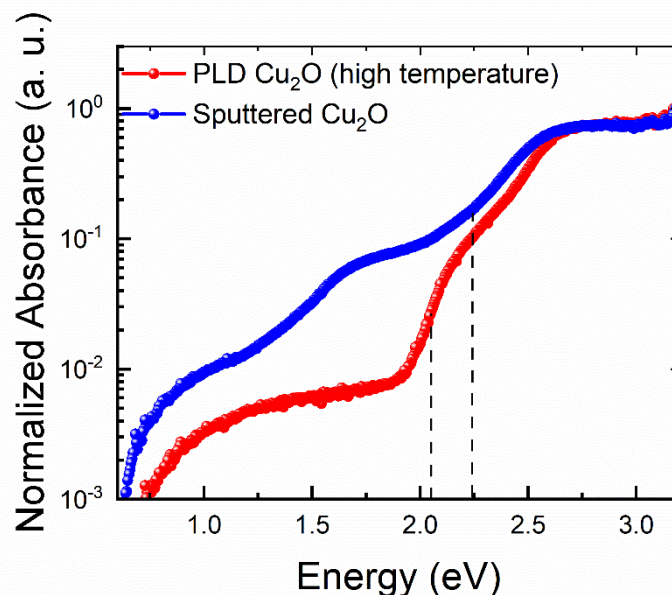
Figure 5.9 Normalized Absorbance spectra of PLD and sputtered Cu 2 O measured from Photothermal Deflection Spectroscopy.
