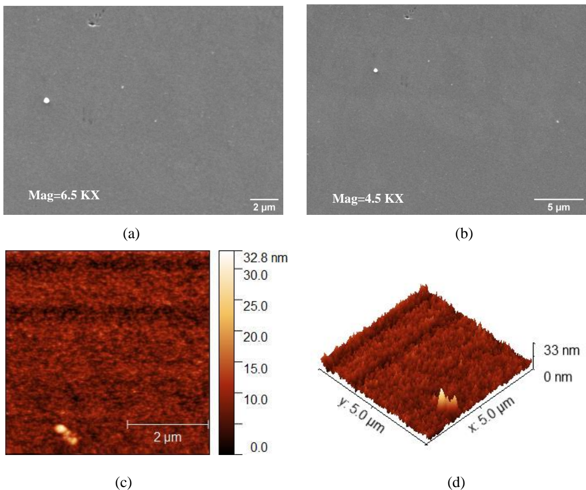
Figure 3.4 (a) and (b) Secondary electron images of \text{Cu}_2\text{O} film deposited by RF magnetron sputtering at different magnifications. AFM image ( 5\ \mu\text{m} \times 5\ \mu\text{m} ) of sputtered \text{Cu}_2\text{O} film (c) in two-dimension (d) in three-dimension
