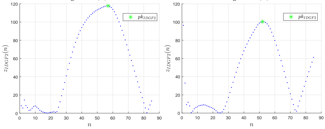
(c) Signal z_{IDGF2}(n) at instantaneous index n_3 of signal z_w(n) (d) Signal z_{IDGF2}(n) at instantaneous index n_4 of signal z_w(n)
