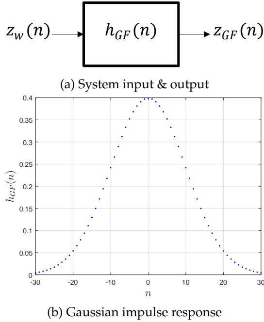
FIGURE 5.6: Gaussian filter system
