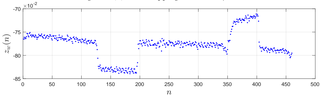
(c) Signal z_w(n) after clipping at elevation \beta = -3^\circ
