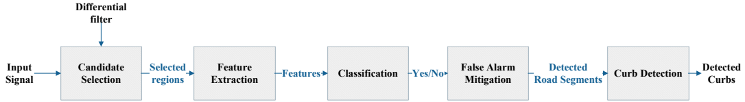
FIGURE 2.10: Flowchart of road/road-edge detection algorithm [91]
