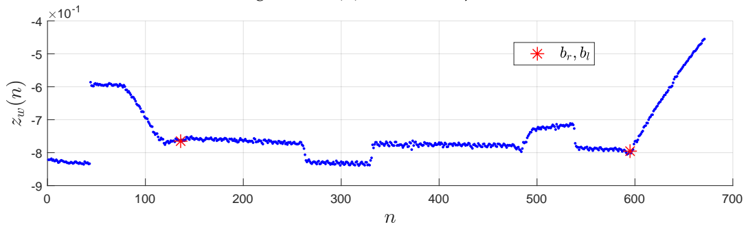
(b) Signal z_w(n) before clipping at elevation \beta = -3^\circ
