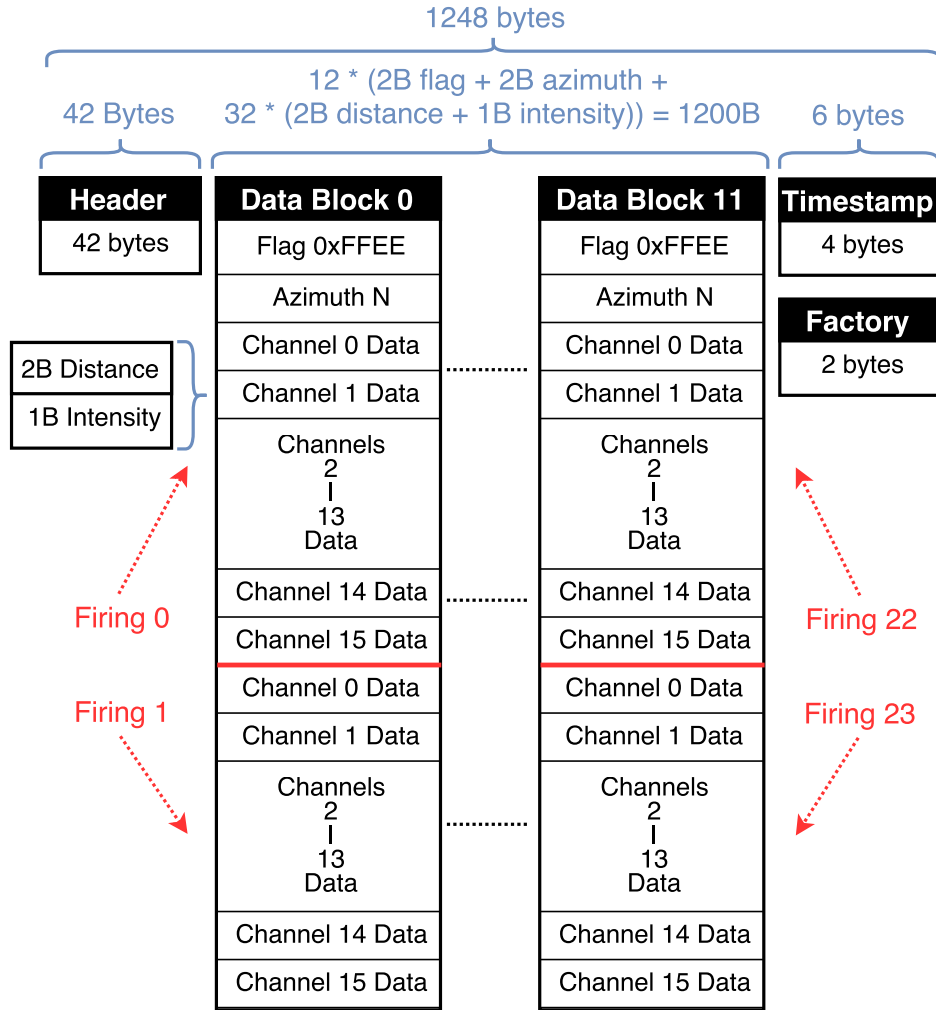
FIGURE A.2: VLP-16 Packet Structure [138]
