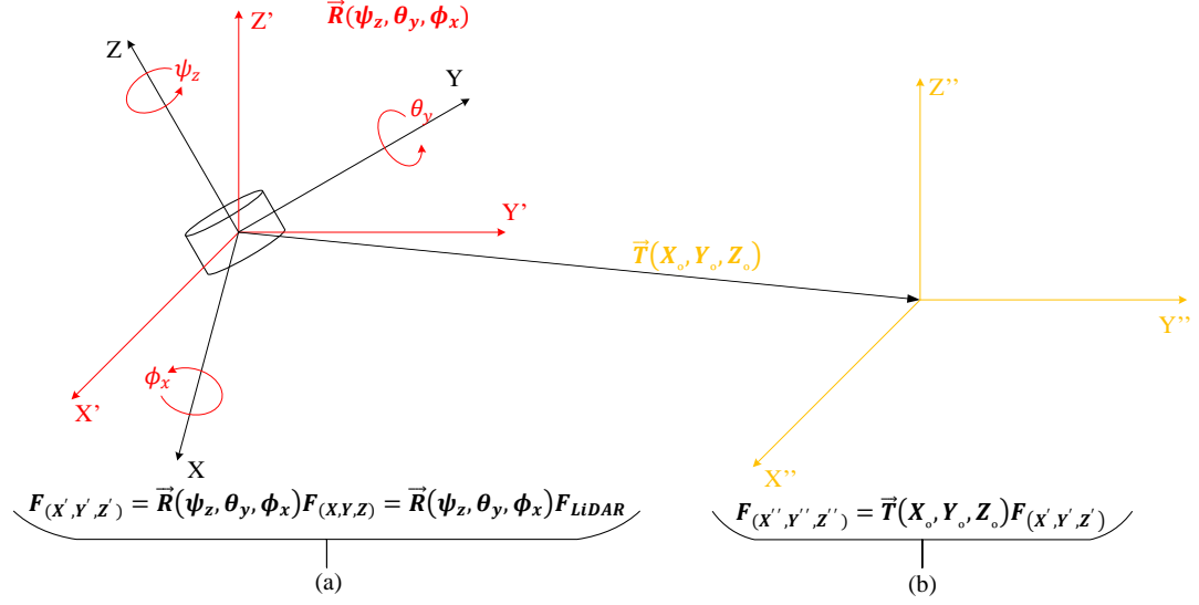
FIGURE 2.6: (a) 3D orientation of LiDAR frame, (b) 3D Translation of LiDAR frame
