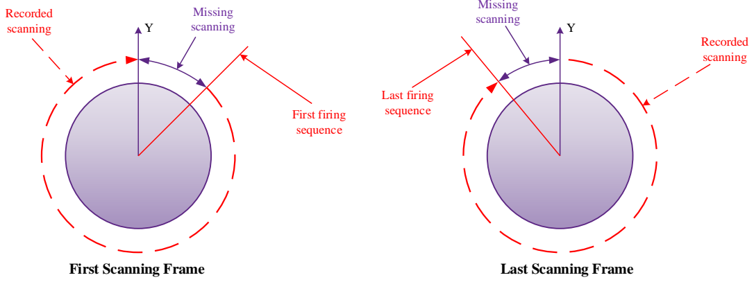
FIGURE 3.4: First and last scanning frames
