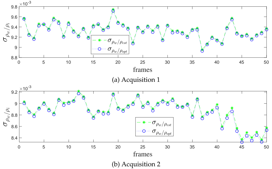
FIGURE 4.12: The variation of \sigma_{\rho_w/\rho_i} with respect to LiDAR frame
