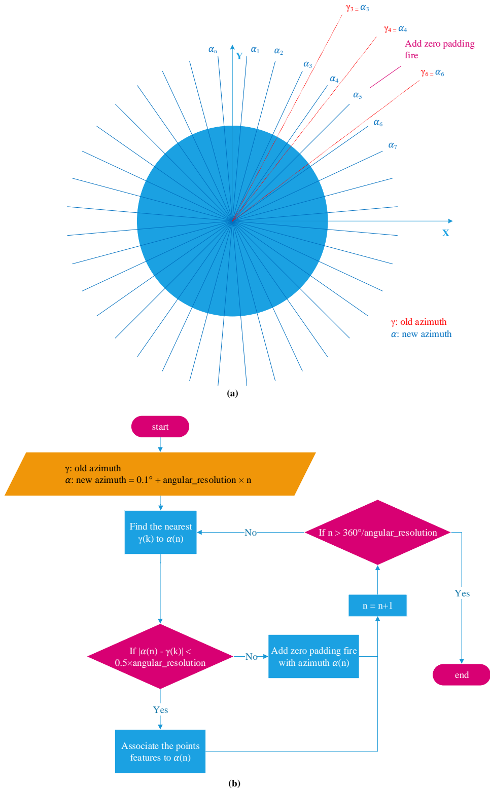
FIGURE 3.5: (a) Top view for old and new azimuth association, (b) Azimuth association algorithm Flowchart
