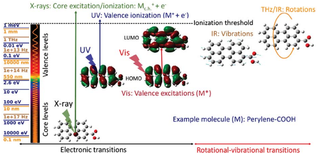
Figure 2.8: Typical molecular excitation processes at various excitation energies, wavelengths and frequencies from X-ray to THz. M_{c.h.}^+ , stands for the ionized molecule with a core hole, M^+ for the ionized molecules with a valence hole and M^* for an excited molecule. *The figure was taken from the reference [69]
