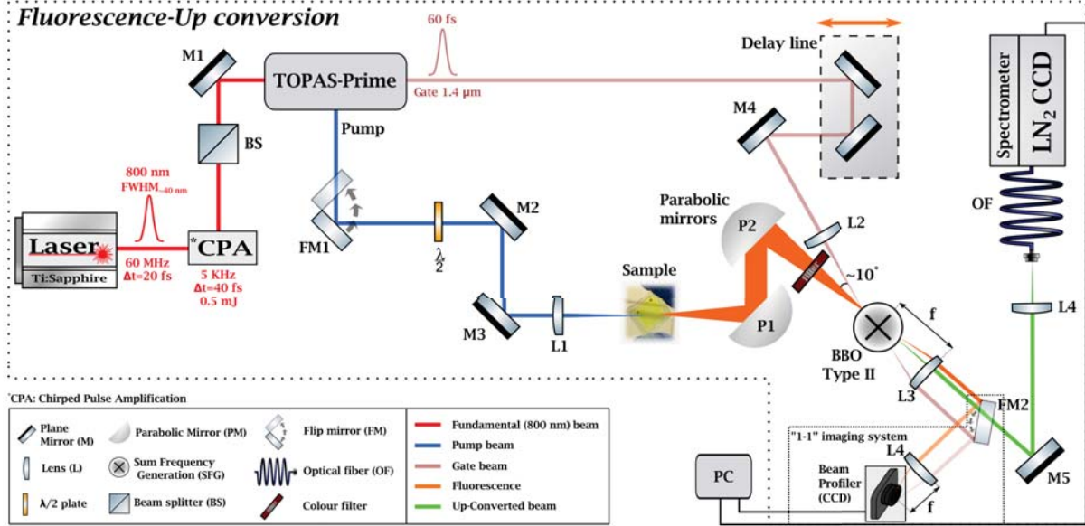
Figure 4.5: Simplified schematic representation of the broadband Fluorescence-Up Conversion (FLUPS) set-up. Right-below (dashed-frame) it demonstrates the "1-1" imaging system of the center of the BBO crystal.
