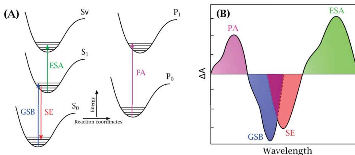
Figure 4.9: (A) Schematic illustration of the major electronic processes probed with TAS. (B) A stochastic representation of the different absorption ( \Delta A ) spectra reflecting the different photophysical processes of Ground State Bleach (GSB), Stimulate Emission (SE), Excited-State Absorption (ESA) and Photo-product Absorption (PA).
