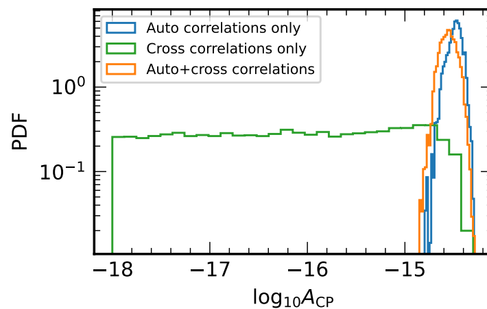
Figure 3.8: Marginalized posterior distributions of the amplitude A of power-laws with fixed spectral index at \gamma = 13/3 for the CURN (blue), the GWB (orange) and the cross correlation only (green) CRS models using the IPTA DR2.
