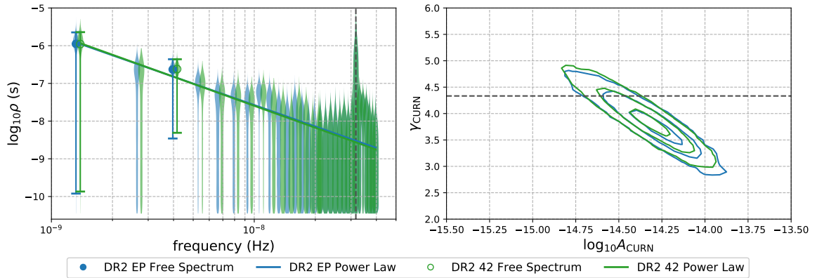
Figure 3.3: Results from CURN analysis using ENTERPRISE (EP) and FORTYTWO (42) with the EPTA DR2 6-pulsars, both for the free-spectrum (left panel) and the single power-law (right panel) analyses. The left plot shows the posterior distribution for the amplitude of the power at each frequency bin using violin plots. Where the inference provides good measurement of the power, we denote the median with a circle and the 95% uncertainties. We consider the measurement good, if more than 95% of the posterior probability lies above the lowest 6.25% of the prior. As the results of the two algorithms are almost identical, we slightly shift the 42 distributions of the lowest 15 frequency bins for easier visual comparison. The right plot shows the two-dimensional posterior distribution for the CURN power-law amplitude and spectral index with the dashed line indicating the expected \gamma = 13/3 from a GWB from SMBHBs. The two analysis pipelines have produced consistent results.
