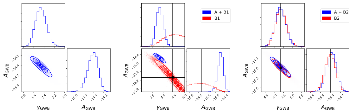
Figure 4.4: 2D marginalized posterior distribution of the GWB model power-law amplitude and spectral index applied on different simulated datasets. In the left panel, the data contains injection of SSE systematics only. In the center panel, it contains either SSE systematics + GWB (blue) or GWB only (red), both with GWB amplitude A = 10^{-16} . In the right panel, the dataset contains either SSE systematics + GWB (blue) or GWB only (red) at A = 10^{-15} (right). The black solid lines indicate the injected amplitude and spectral index of the GWB power-law.
