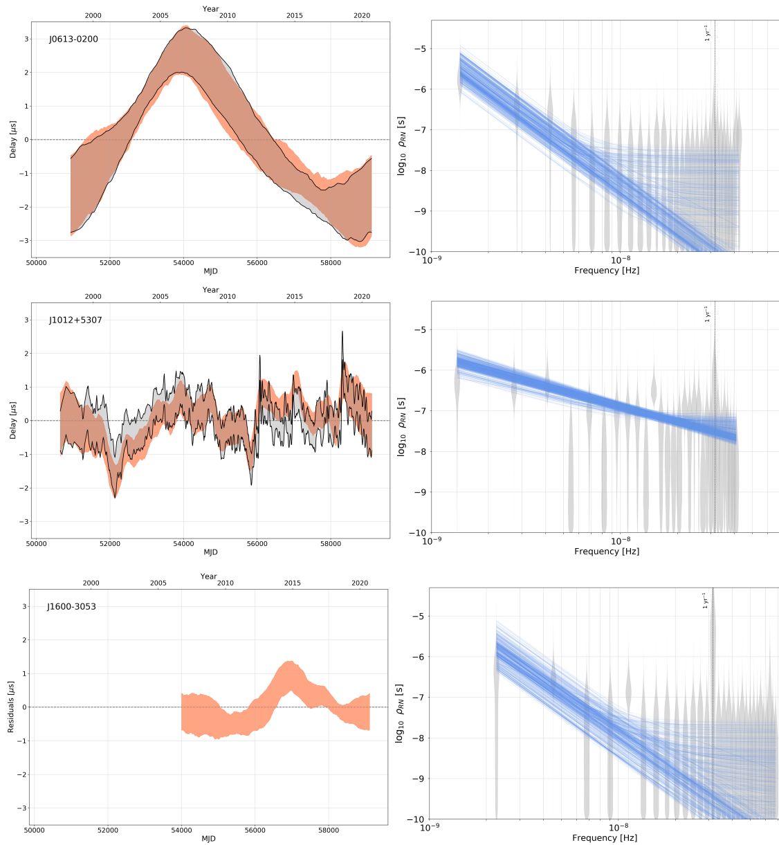
Figure 2.9: (left panels) 68% confidence interval of 100 time-domain random realizations of the achromatic red-noise included in the default base ( RN30_DM100 ) model (red) and the "custom" selected models (light grey) (cf. Table 2.5) for each of the six pulsars. (right panels) Achromatic red-noise spectrum for the corresponding pulsar (noted in left panel) included in the default base model and described with (1) a free-spectrum PSD (grey violins) or (2) a broken power-law (blue), here showing 1000 random realizations drawn from the posterior distributions. The figure continues on the next page.
