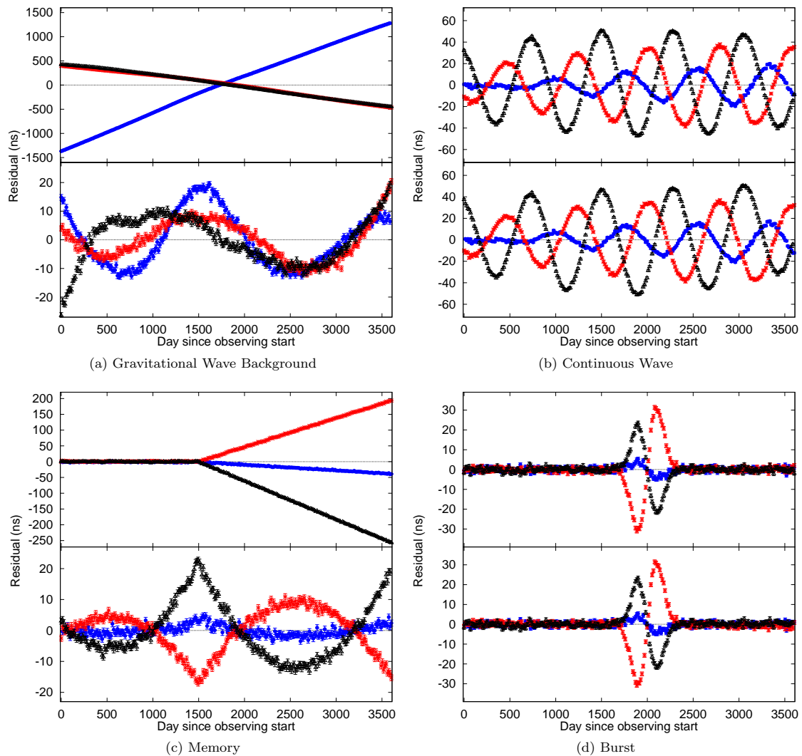
Figure 1.10: Simulated pulsar timing residuals before and after fitting for the TM parameters (resp. top and bottom of each sub-panel) for three pulsars with different sky locations (black, blue and red) that contains signals from (a) a GWB from a SMHBH population, (b) a single SMBHB system, (c) a burst with memory and (d) a generic (Gaussian) burst (from Burke-Spolaor 2015).
