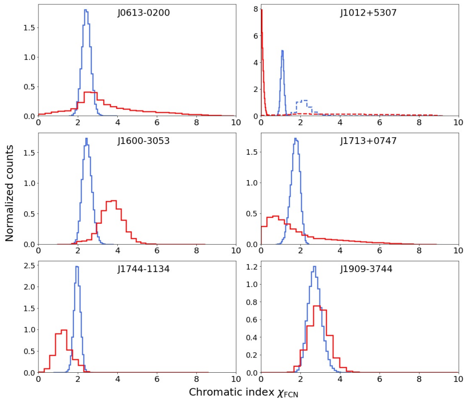
Figure 2.3: Marginalized posterior distributions of chromatic index \chi_{\text{FCN}} in RN_{\text{FCN}} (solid blue) and RN_{\text{DMv\_FCN}} (solid red) for the six pulsars. The number of frequency bins for RN and DMv power-law are taken from Table 2.2. For PSR J1012+5307 we performed additional analysis with models RN150_{\text{FCN}150} (dashed blue) and RN150_{\text{DMv}150_{\text{FCN}150} (dashed red).
