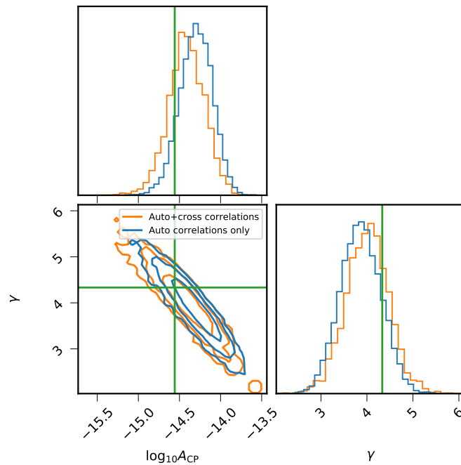
Figure 3.7: 2D marginalized posterior distributions of the power-law amplitude and spectral index for the common process (CP) modelled as a CURN (Auto correlations only) or a GWB (Auto + cross correlations) with the IPTA DR2. The green lines indicate A_{CP} = 2.8 \times 10^{-15} and \gamma_{\text{SMBHB}} = 13/3 .
