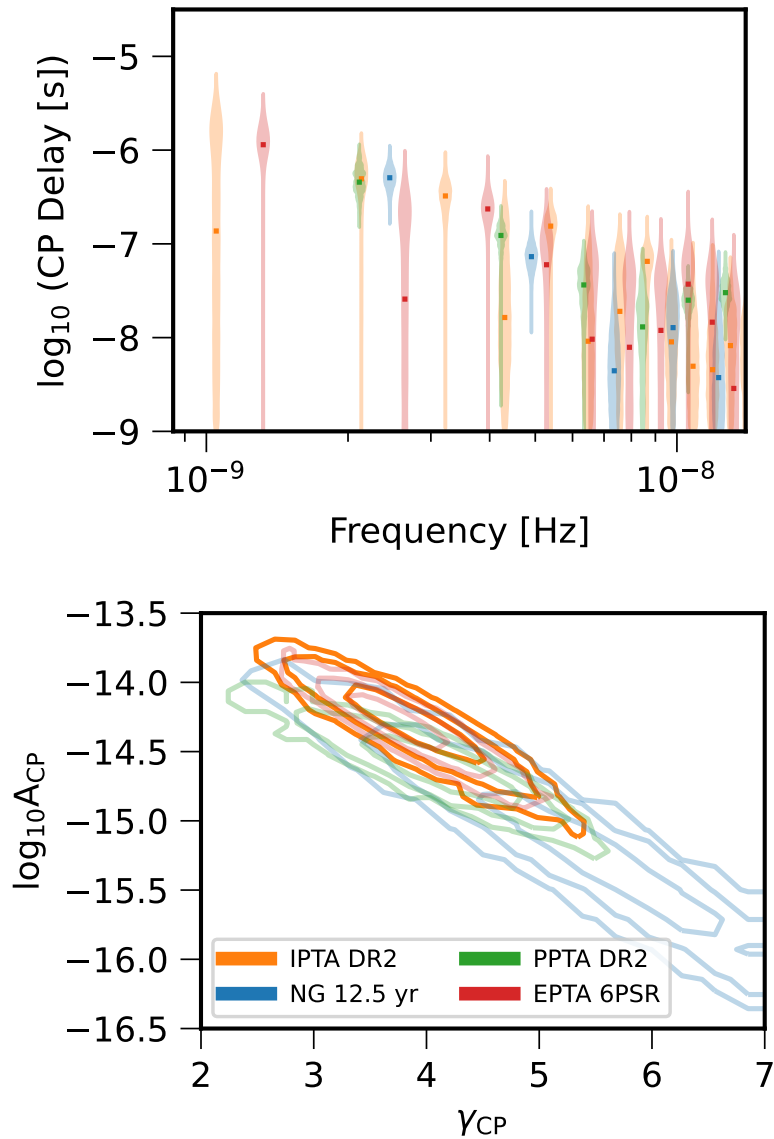
Figure 3.10: Comparison of the CRS modelled with a free-spectrum (top) or a power-law PSD (bottom) between the following datasets: IPTA DR2 (orange; Perera et al. 2019), NANOGrav 12.5 years dataset (blue; Alam et al. 2021), PPTA DR2 (green; Kerr et al. 2020) and six pulsars from EPTA DR2. Note that even if the datasets of the three continental PTAs include more recent ToAs than the IPTA DR2, the time span of the latter is bigger because it contains legacy data with observations performed in the 1980's. Figure from Antoniadis et al. 2022.
