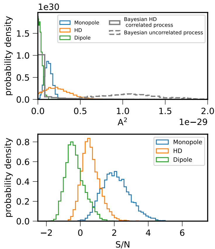
Figure 3.9: Amplitude A^2 (top) and S/N (bottom) obtained from the noise marginalized optimal statistic applied for a CRS modelled with monopolar (blue), dipolar (green) or Hellings-Downs correlations using the IPTA DR2. The amplitudes obtained from Bayesian analysis are also plotted (top) for the CURN (black line) and the cross correlation only (black dashed-lines).
