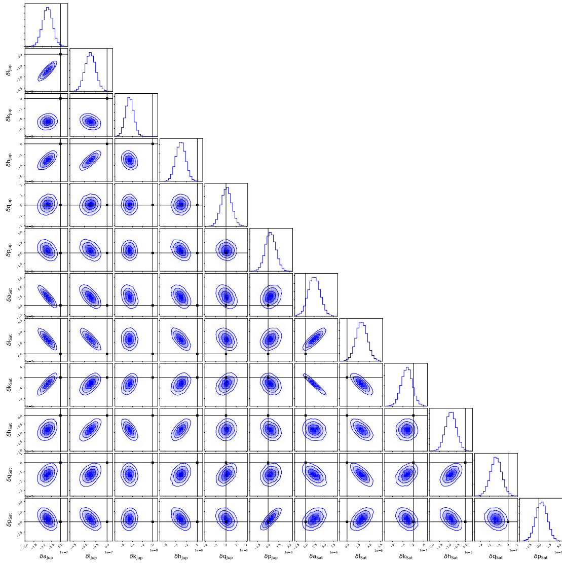
Figure 4.5: Posterior distributions of EPHEMGP parameters applied on the dataset including the signal A only. The black solid lines indicate the zero value for each parameter.
