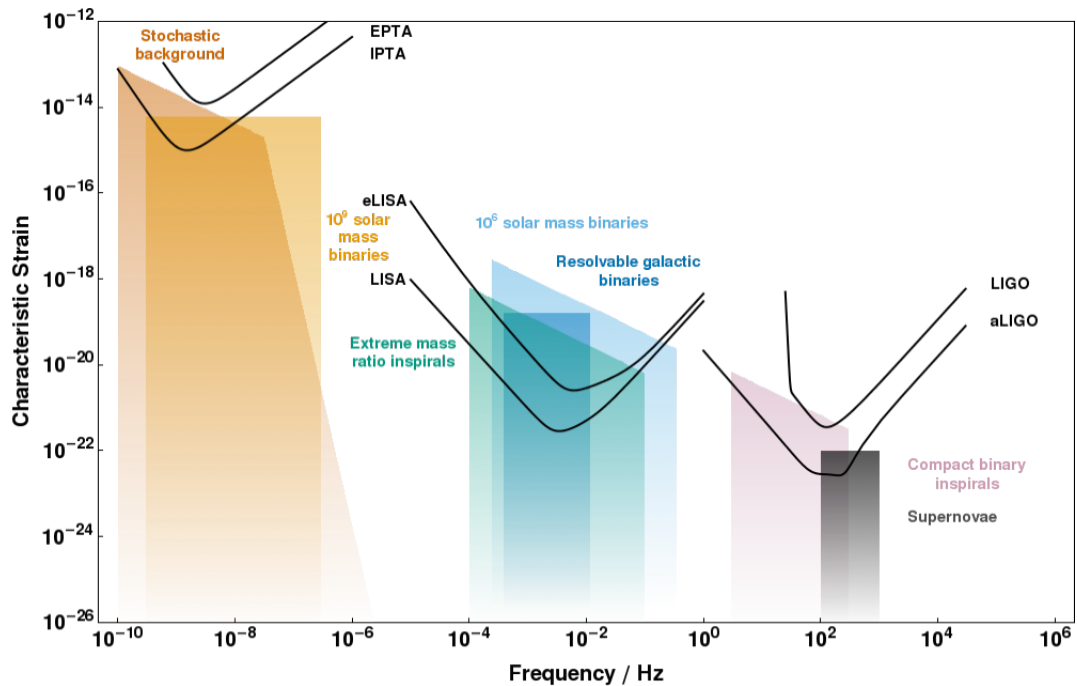
Figure 1.11: The gravitational wave spectrum with the related sources and detectors (from Moore et al. 2014).
