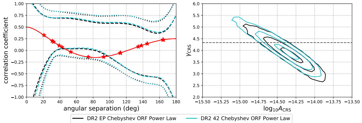
Figure 3.2: ENTERPRISE (EP) and FORTYTWO (42) results from a search for a CRS modelled with a single-power-law spectrum simultaneously sampled with the ORF using the EPTA DR2 6-pulsars. The ORF is approximated with a 4th-order Chebyshev polynomial. Left: The posterior distribution for the angular correlation curve of the CRS, shown as boundaries of the credible regions. The dashed and dotted lines denote the 95% and 99.7% credible regions, respectively. The theoretical Hellings-Downs curve is overplotted for comparison as a solid red line. The red stars denote the angular separations of the pulsars used in this study. Right: Two-dimensional posterior distribution of the spectral parameters for the single-power-law CRS model with the dashed line indicating the expected \gamma = 13/3 from a GWB from SMBHBs.
