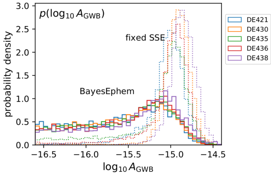
Figure 4.2: Marginalized posterior distribution of the power-law amplitude A_{GWB} (set at f = 1 \text{ yr}^{-1} ) of a CRS model with a fixed spectral index at \gamma = 13/3 and Hellings-Downs correlations (GWB) using the NANOGrav 11-year dataset and including (solid lines) or not (dashed lines) a model named BAYESEPHM that takes into account SSE uncertainties (from Vallisneri et al. 2020). The colors denote different choice of JPL ephemeris used by the timing model.
