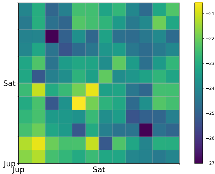
Figure 4.6: Color map of the Jupiter and Saturn non-singular orbital element covariance matrix given by INPOP19a. For each body, the parameters are a, l, k, h, q, p .
