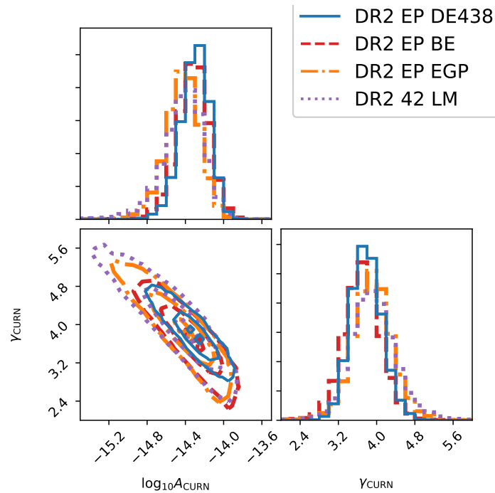
Figure 4.8: Posterior distributions of CURN power-law parameters using ENTERPRISE with (i) fixed DE438 SSE, (ii) BAYESEPHM (BE), (iii) EPHEMGP (EGP) and FORTYTWO with LINIMOSS (LM). Figure from Chen et al. 2021.
