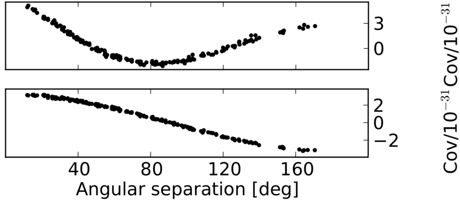
Figure 4.1: Angular separation pairs of pulsars pair vs. correlation coefficient in the presence of GWB (top) and Solar system Roemer delay error (bottom) which is injected as a stochastic dipolar signal (from Tiburzi et al. 2016).
