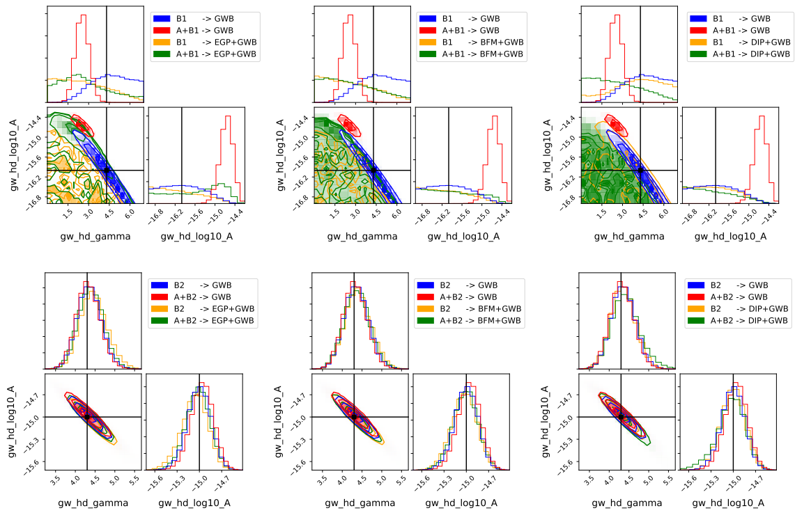
Figure 4.7: Comparison of the three investigated SSE error models: EGP (left), BFM (center) and DIP (right). The figures display the GWB amplitude and spectral index posterior distributions obtained with different datasets processed with different noise models. All simulations involve a GWB signal at (top panels) low-S/N regime ('B1' : A = 10^{-16} ) or high S/N regime ('B2' : A = 10^{-15} ). For each plot, the legend indicates the injected signals ('B1' or 'B2' with or without 'A'), and the related noise model (GWB with or without SSE error). The black solid lines show the injected GWB value.
