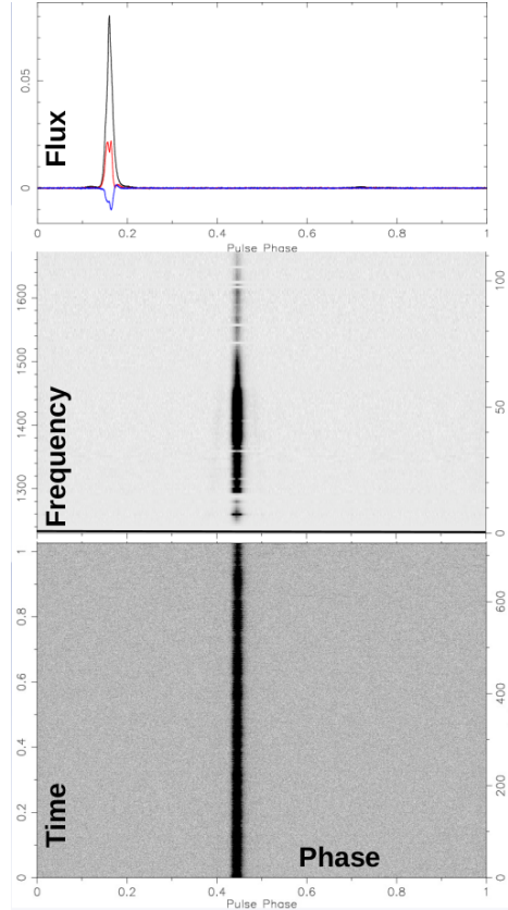
Figure 1.6: L-band observation of PSR J1909-3744 from the Nançay Radio Telescope.
