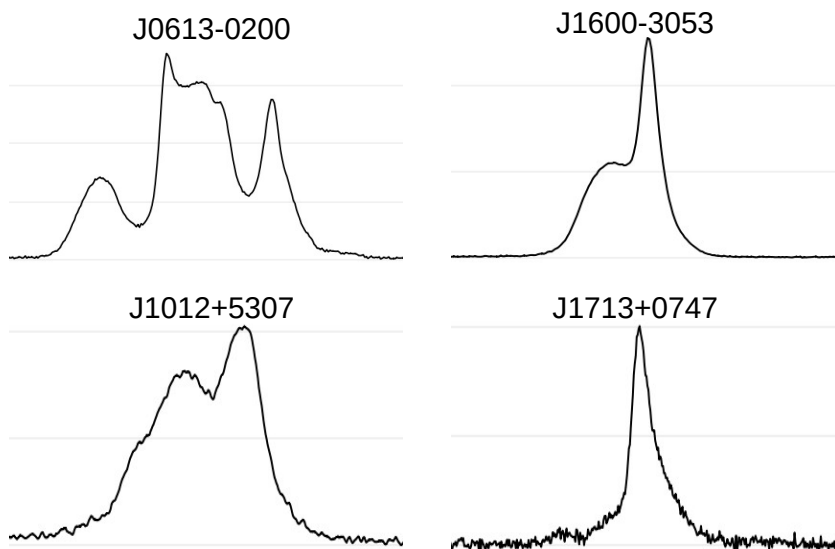
Figure 1.2: Rotational phase fractions of integrated pulse profiles of four different pulsars from the European Pulsar Network 2 (EPN) database.
