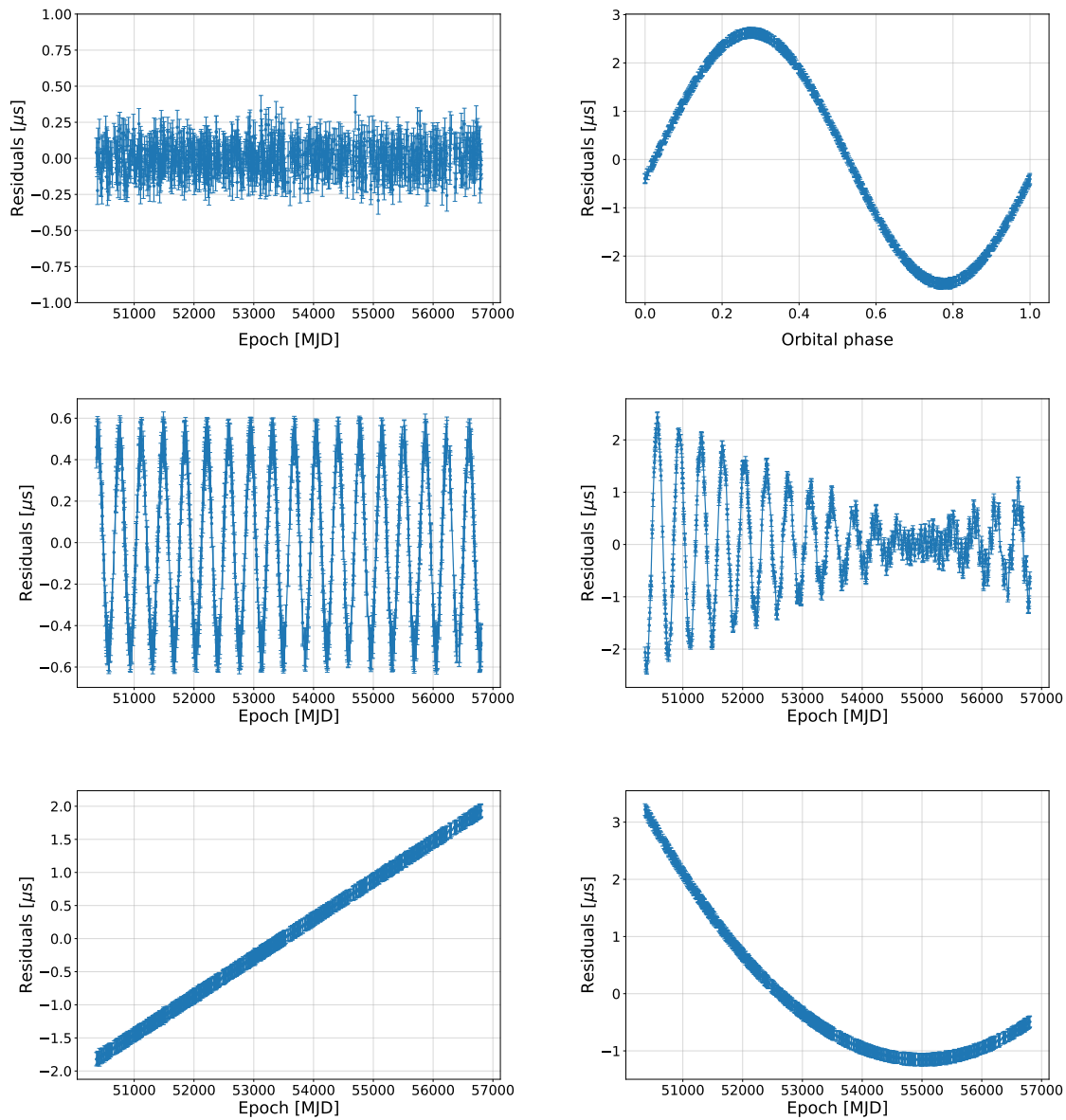
Figure 1.5: Simulated timing residuals for the case of (top left) a perfect TM fit, (top right) error in the projected semi-major axis A_1 , (second row left) error in positions RAJ and DECJ, (second row right) errors in proper motions PMRA and PMDEC, (lower left) error in frequency F_0 and (lower right) error in the frequency derivative F_1 . The reference epochs for the position and frequency are both at MJD 55000.
