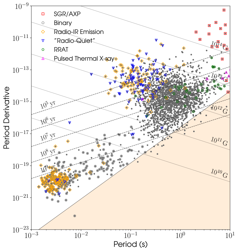
Figure 1.3: The pulsar zoology with the P-\dot{P} diagram obtained from the ATNF Pulsar Catalogue v.1.65. All pulsars are shown with grey dots and different subgroups are represented: soft Gamma-ray repeaters (SGR) and anomalous X-Ray pulsars (AXP) in red squares, those in a binary system with a grey circle, those observed in the infrared in yellow diamonds, those not detected in radio in blue triangle, rotating radio transient sources (RRAT) with intermittent pulsed radio emission in green hexagons and neutron stars with thermal pulsed X-ray emission in pink triangles. The orange shaded region is called the pulsar "graveyard", delimited by the "death line", under which the pulsars are not expected to emit detectable radio beams because they supposedly cannot support pair production (Chen and Ruderman 1993).
