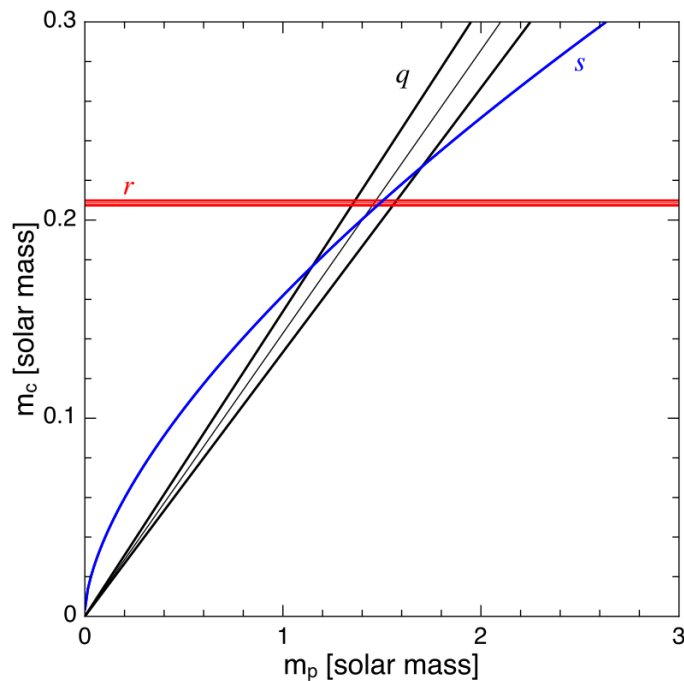
Figure 1.9: Mass–mass diagram of PSR J1909-3744 binary system (Liu et al. 2020). Constraints from r and s parameters are obtained from the pulsar timing analysis and q is obtained from optical observations of the white dwarf companion (Antoniadis 2013).
