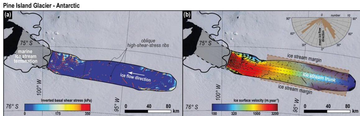
Figure 13. Maps of inverted (a) basal shear stress (kPa) beneath Pine Island Glacier and (b) ice-surface velocity (modified from Sergienko and Hindmarsh, 2013). Small and isolated areas of very high basal shear stress (red in panel a and black in panel b) referred to as “high-shear-stress ribs” are obliquely set to the main ice flow direction. The orientations of oblique ribs relative to the mean ice flow direction, located in the rectangular brown areas (along ice stream margins), are compiled in a rose diagram in (b) (© Landsat/Copernicus – © Google Earth).
