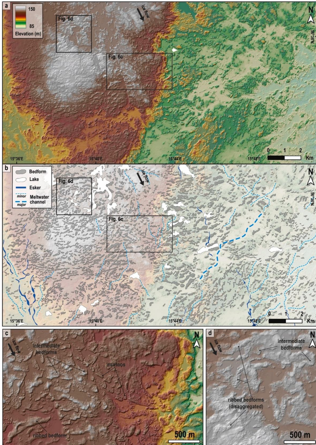
Fig. 6. (a) Lidar DEM and (b) interpretive morphological map with digitized bedforms of a southern portion of the south Sweden Ice Lobe. (c) Murtoos, intermediate bedforms and ribbed bedforms form a morphological transition from the center toward the lateral margin of the murtoo field. (d) Some ribbed bedforms display a disaggregated appearance and are spatially associated with murtoos and intermediate bedforms.
