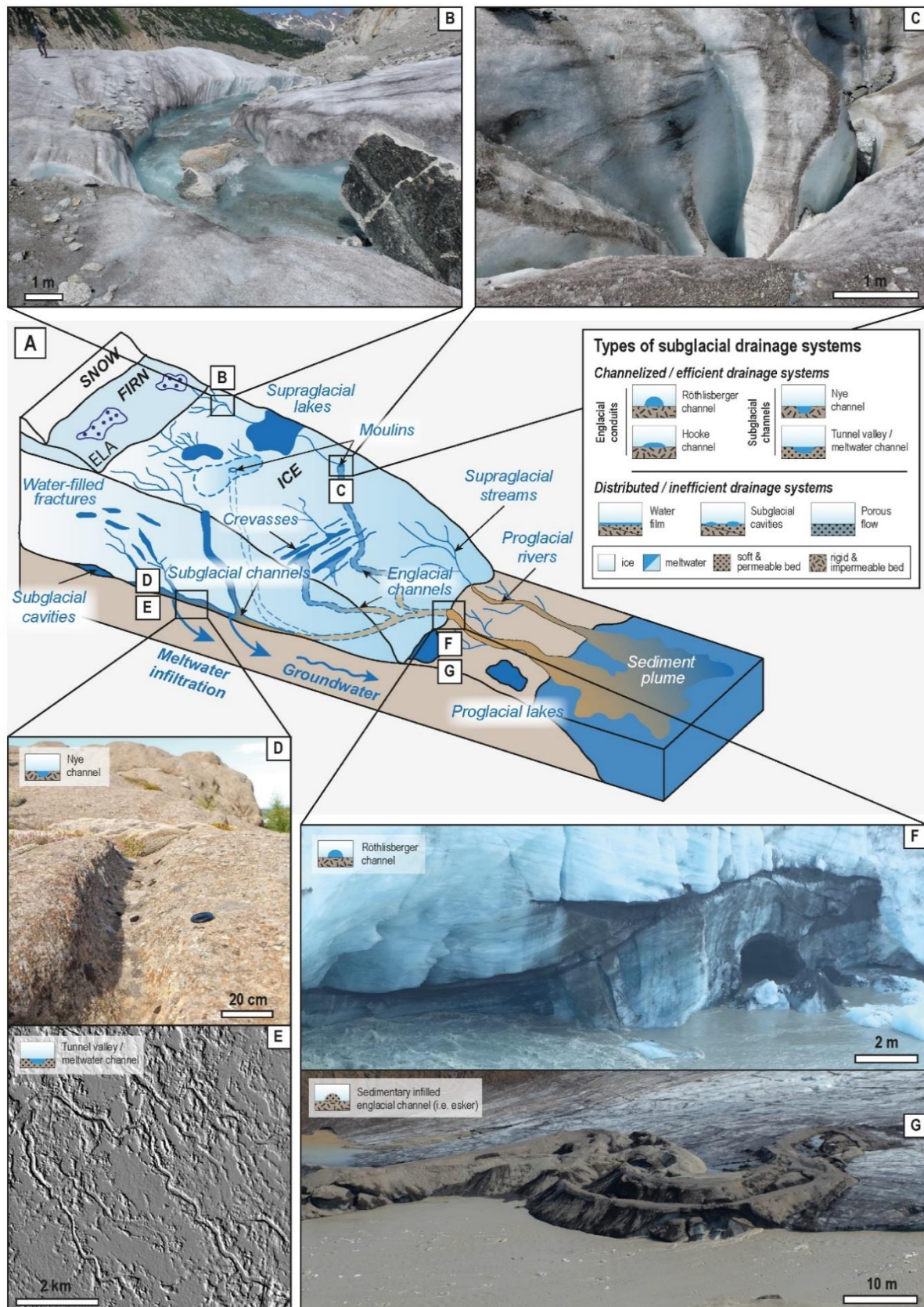
Figure 1.8. (A) Ice sheet hydrological system with a focus on the variety of subglacial drainage systems (Ravier & Buoncristiani, 2018 modified after Cuffey & Paterson, 2010). (B) and (C) Elements of supra-glacial hydrological system: (B) supra-glacial stream and (C) moulins (Mer de Glace, France). Elements of sub-glacial hydrological system: (D) Nye channel (Egilsstadir, Iceland), (E) meltwater channels (Fort Simpson, Great Slave Lake Ice Stream, Canada), (F) Röthlisberger channel (Eyjabakkajökull, Iceland), (G) esker as a morphological relic of an englacial channel (Eyjabakkajökull, Iceland) (all pictures are personal photographs).
